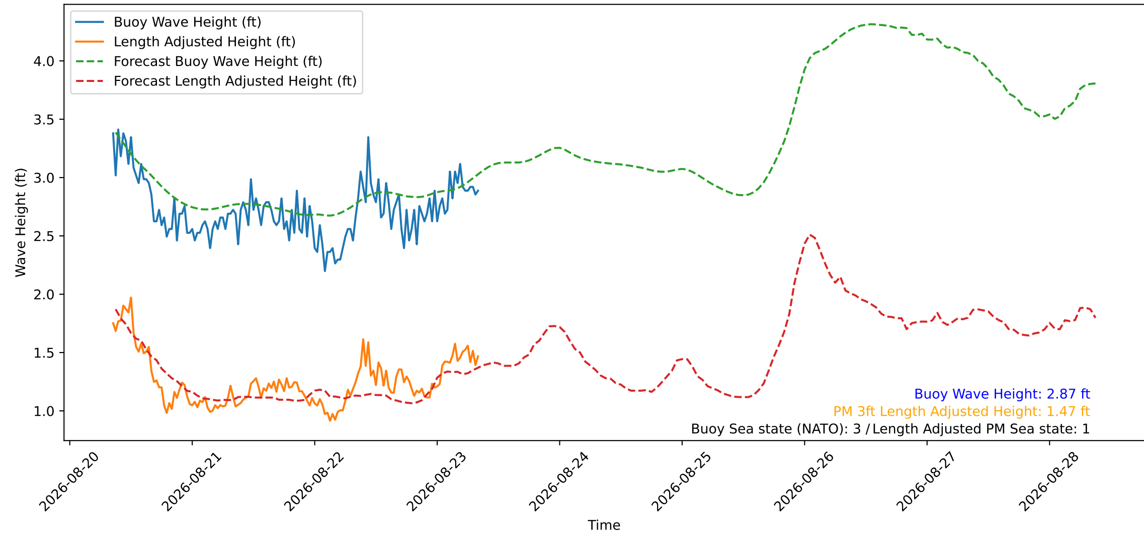
Wave Heights over Time for Oceanside Harbor at 2026-08-23 08:40:29
