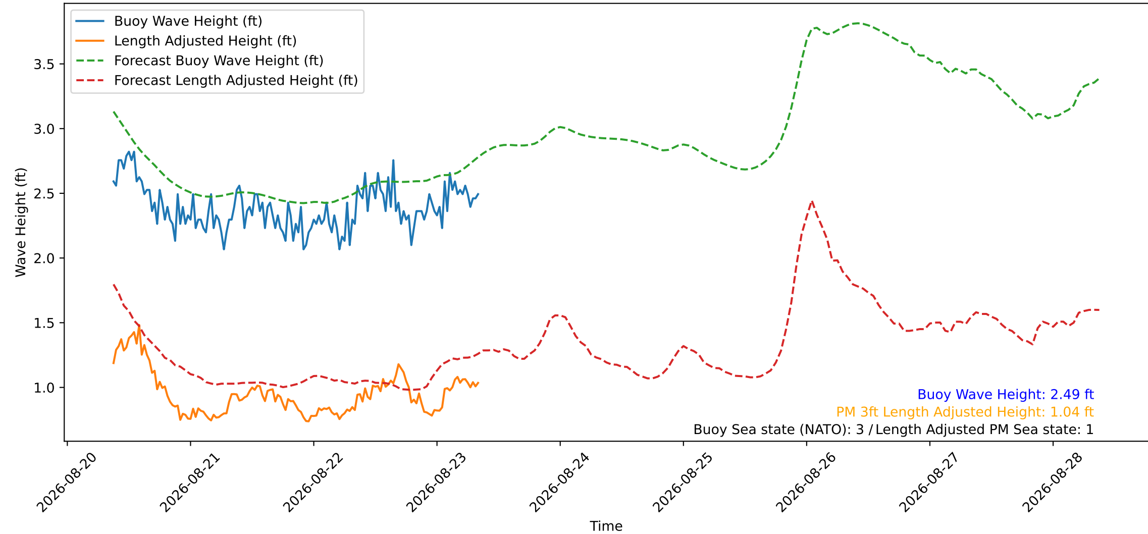
Wave Heights over Time for Red Beach at 2026-08-23 08:40:49
