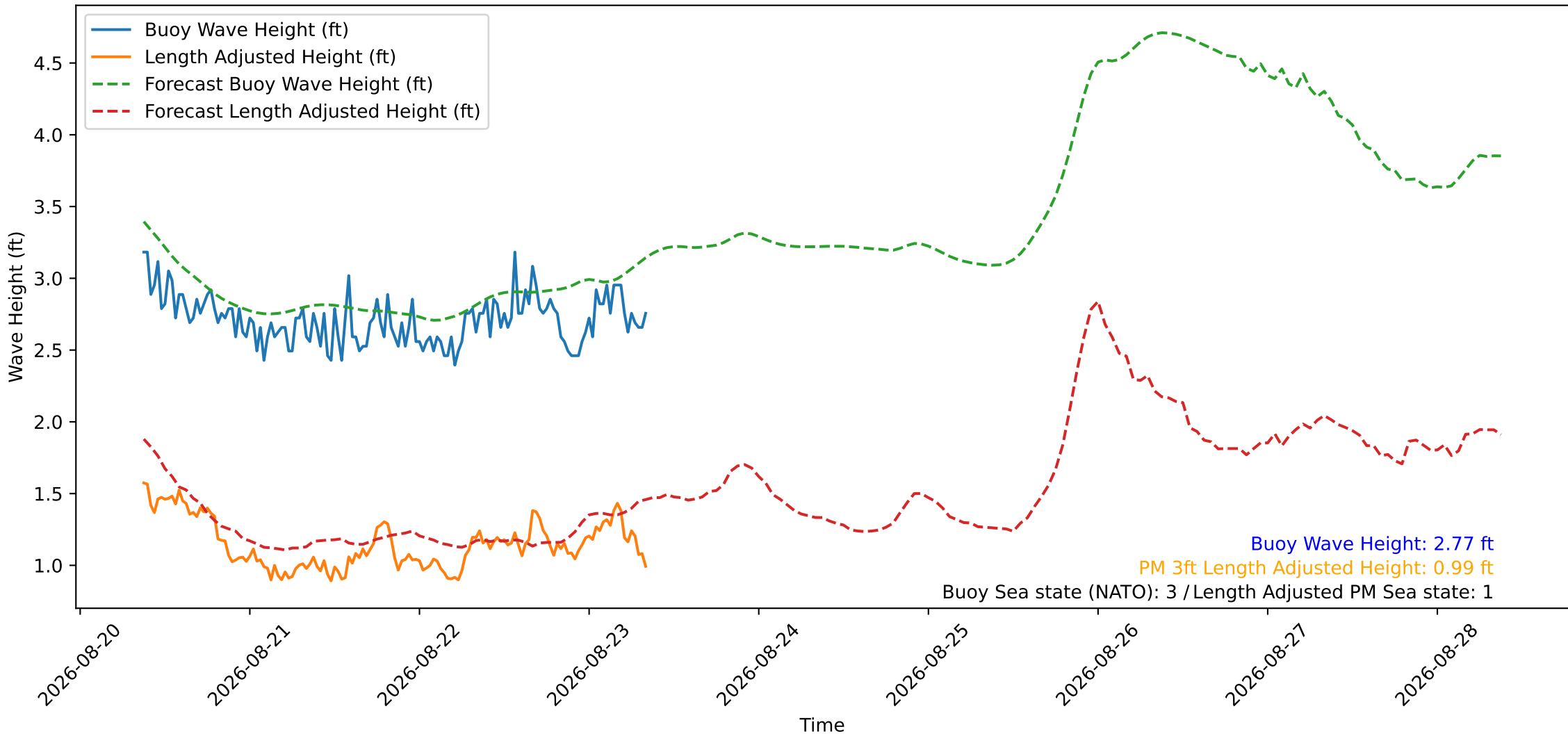
Wave Heights over Time for Green Beach at 2026-08-23 08:41:11
