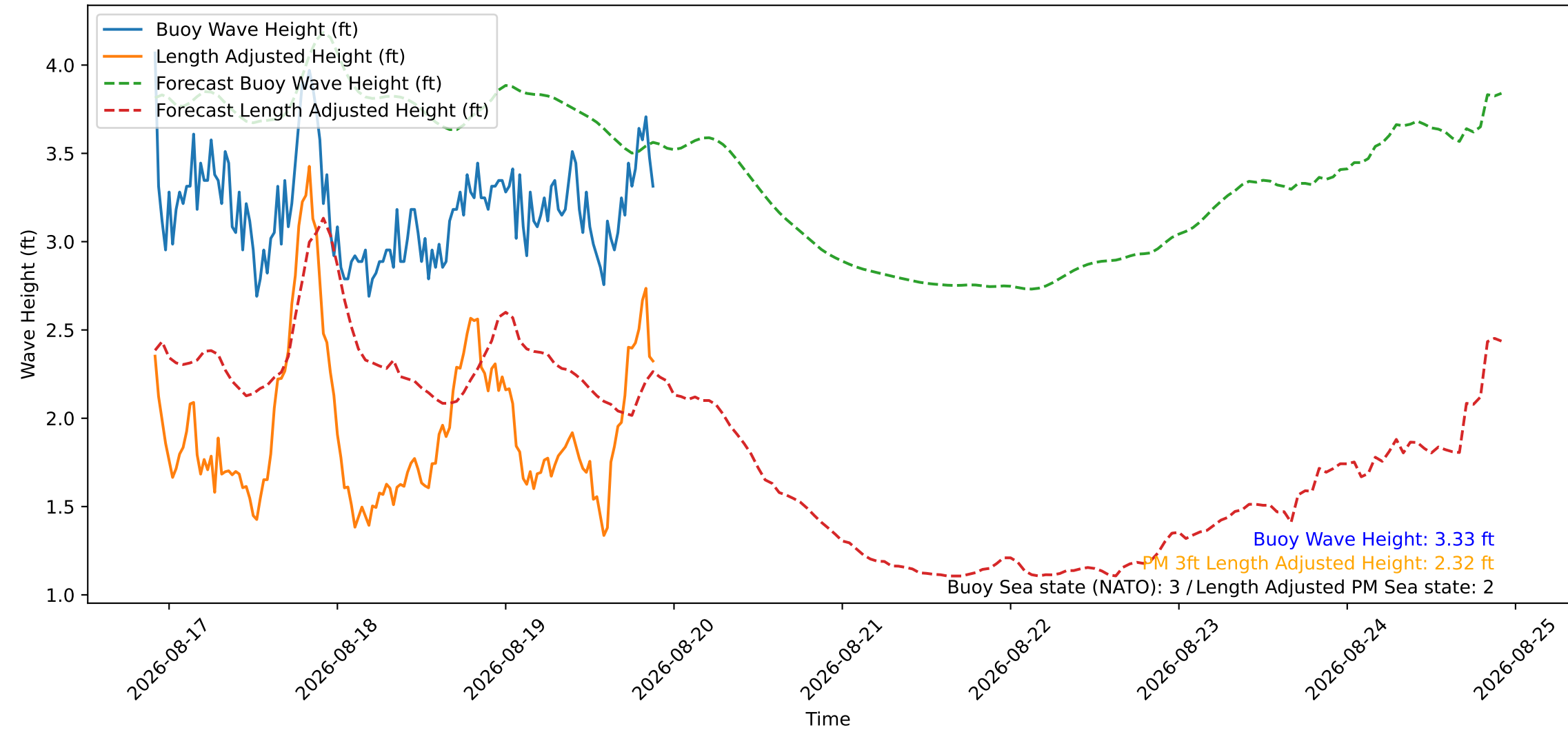
Wave Heights over Time for Green Beach at 2026-08-19 21:41:08
