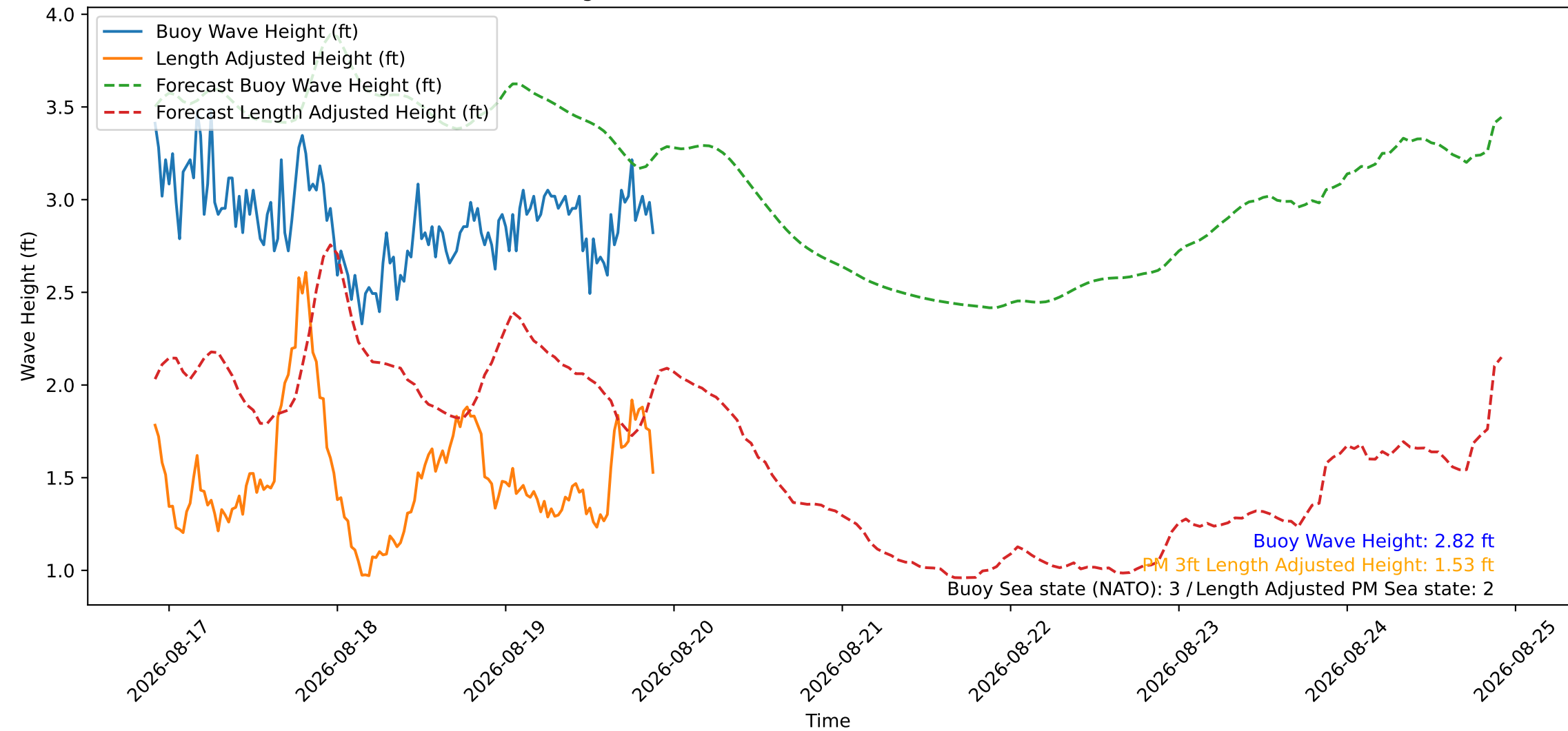
Wave Heights over Time for Red Beach at 2026-08-19 21:40:45
