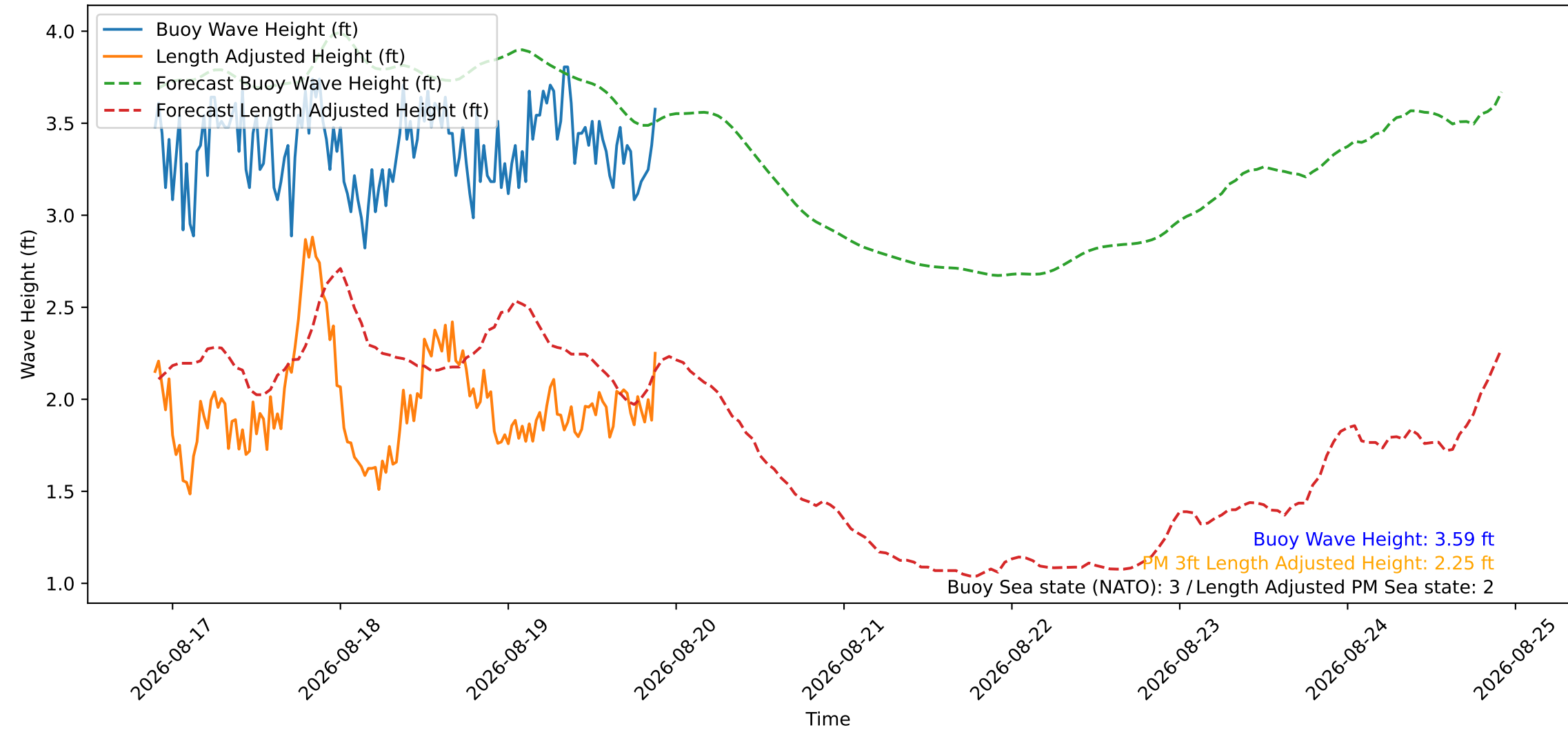
Wave Heights over Time for Oceanside Harbor at 2026-08-19 21:40:26
