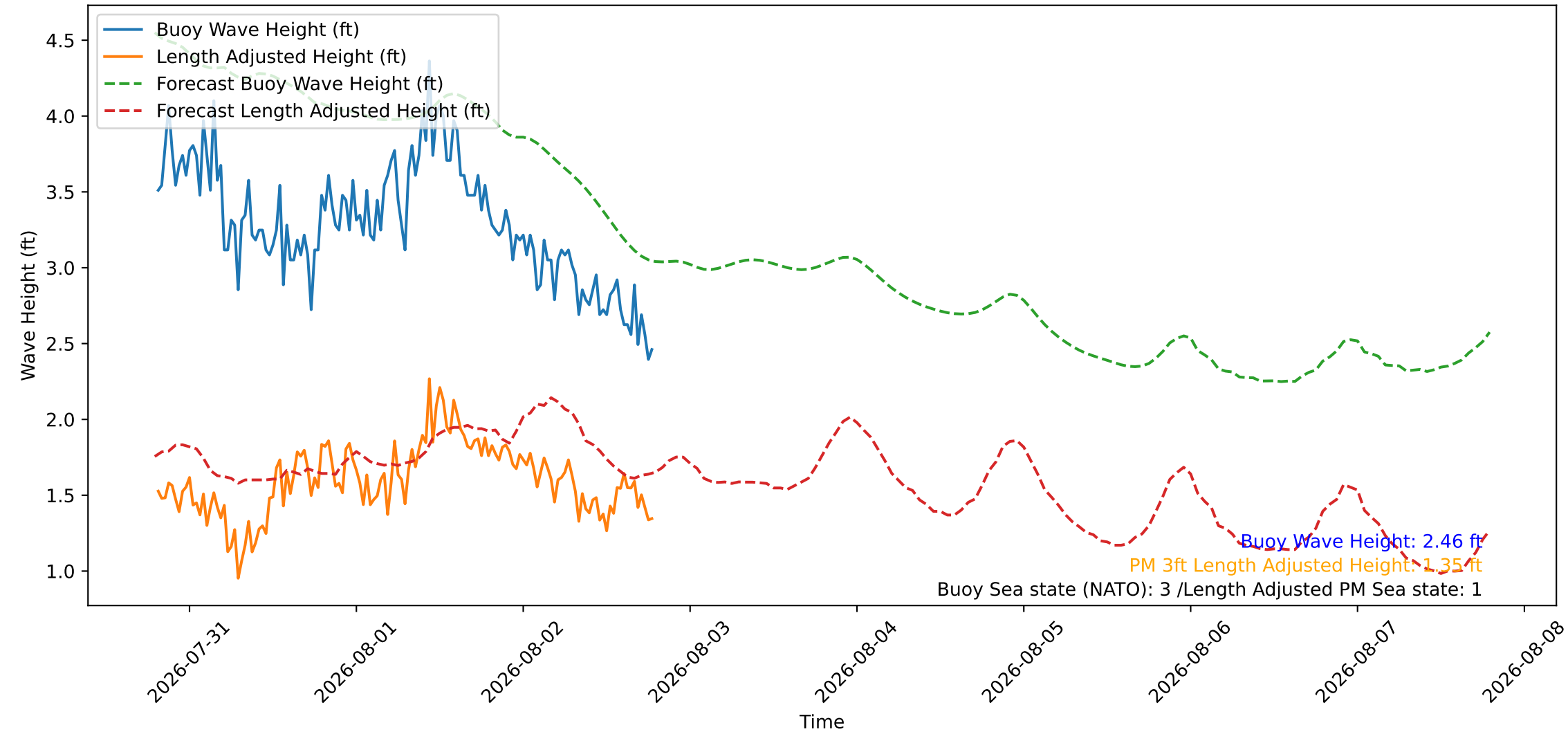
Wave Heights over Time for Oceanside Harbor at 2026-08-02 19:20:26
