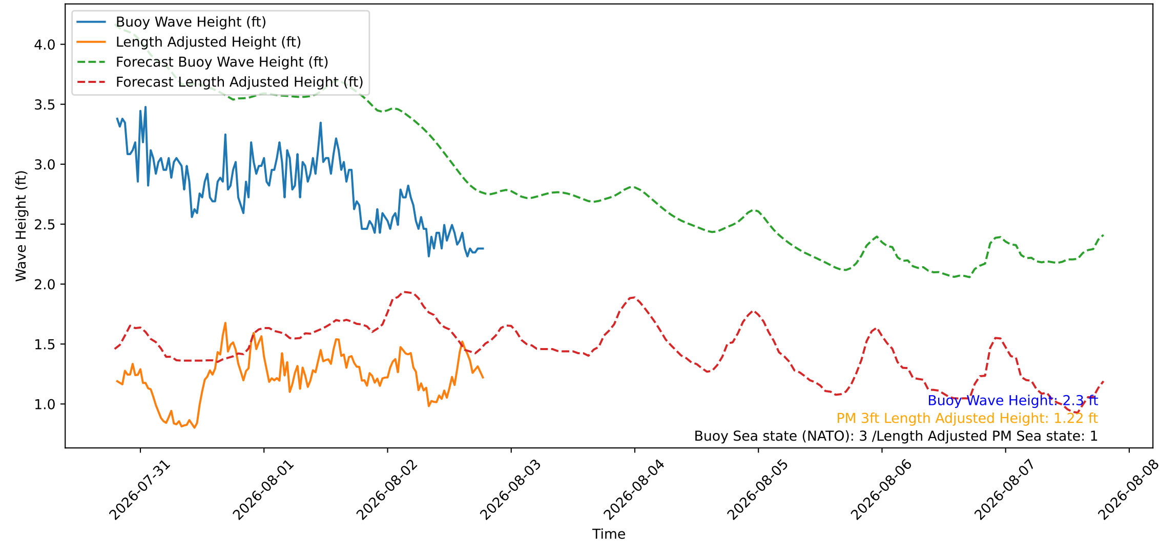
Wave Heights over Time for Red Beach at 2026-08-02 19:20:47
