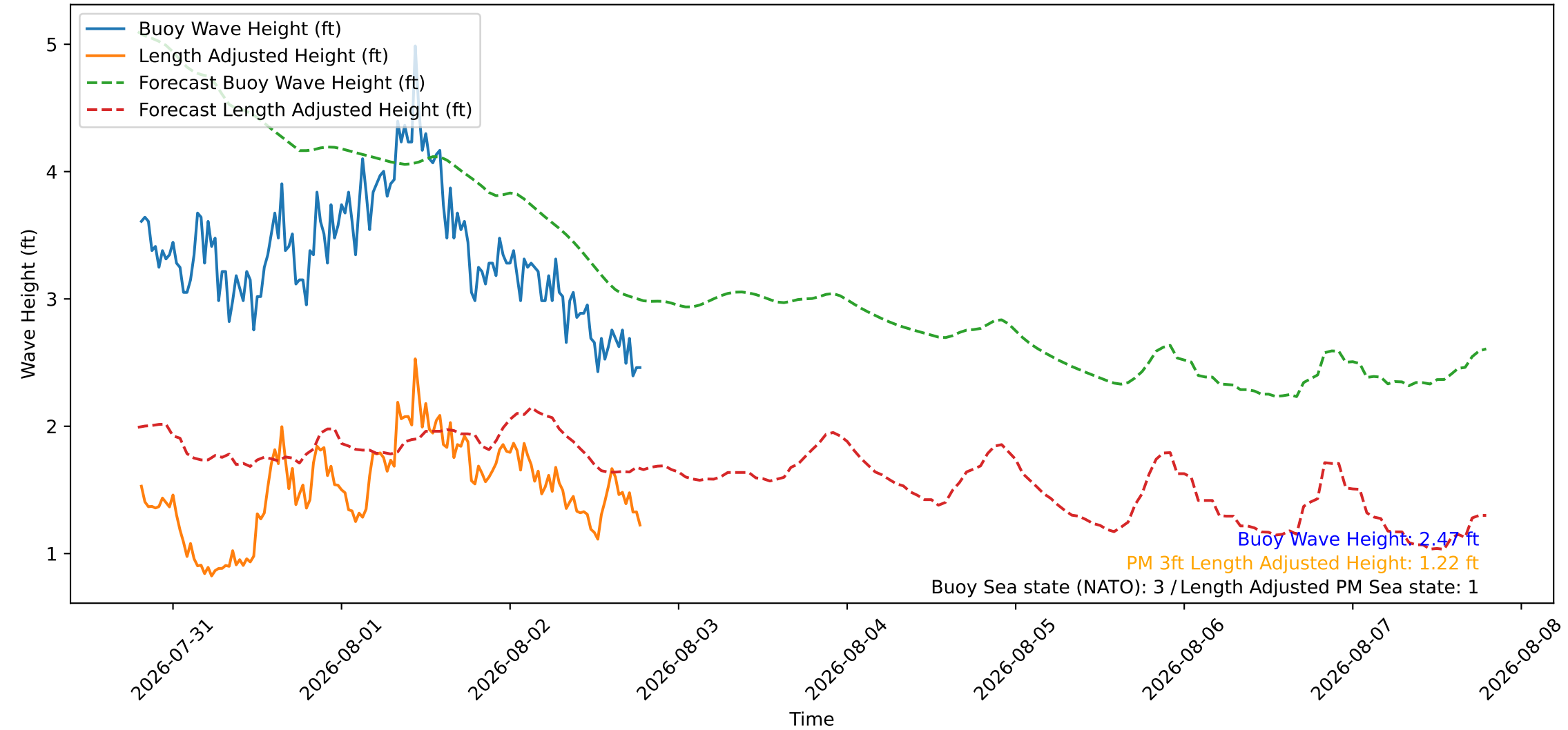
Wave Heights over Time for Green Beach at 2026-08-02 19:21:09
