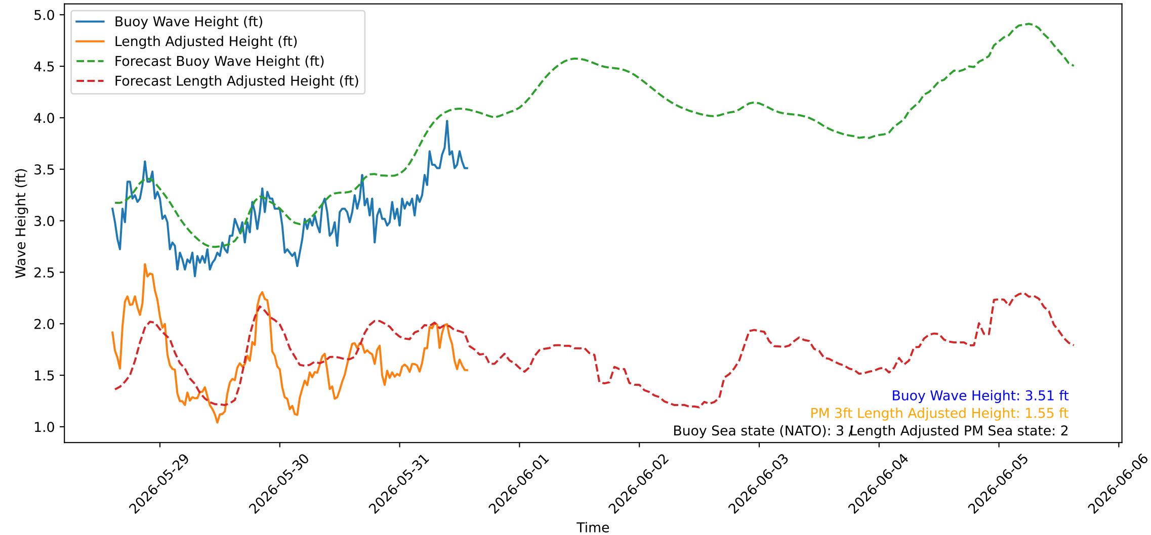
Wave Heights over Time for Green Beach at 2026-05-31 14:31:08
