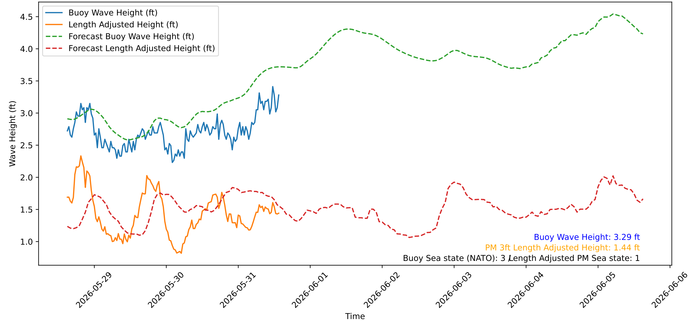
Wave Heights over Time for Red Beach at 2026-05-31 14:30:45
