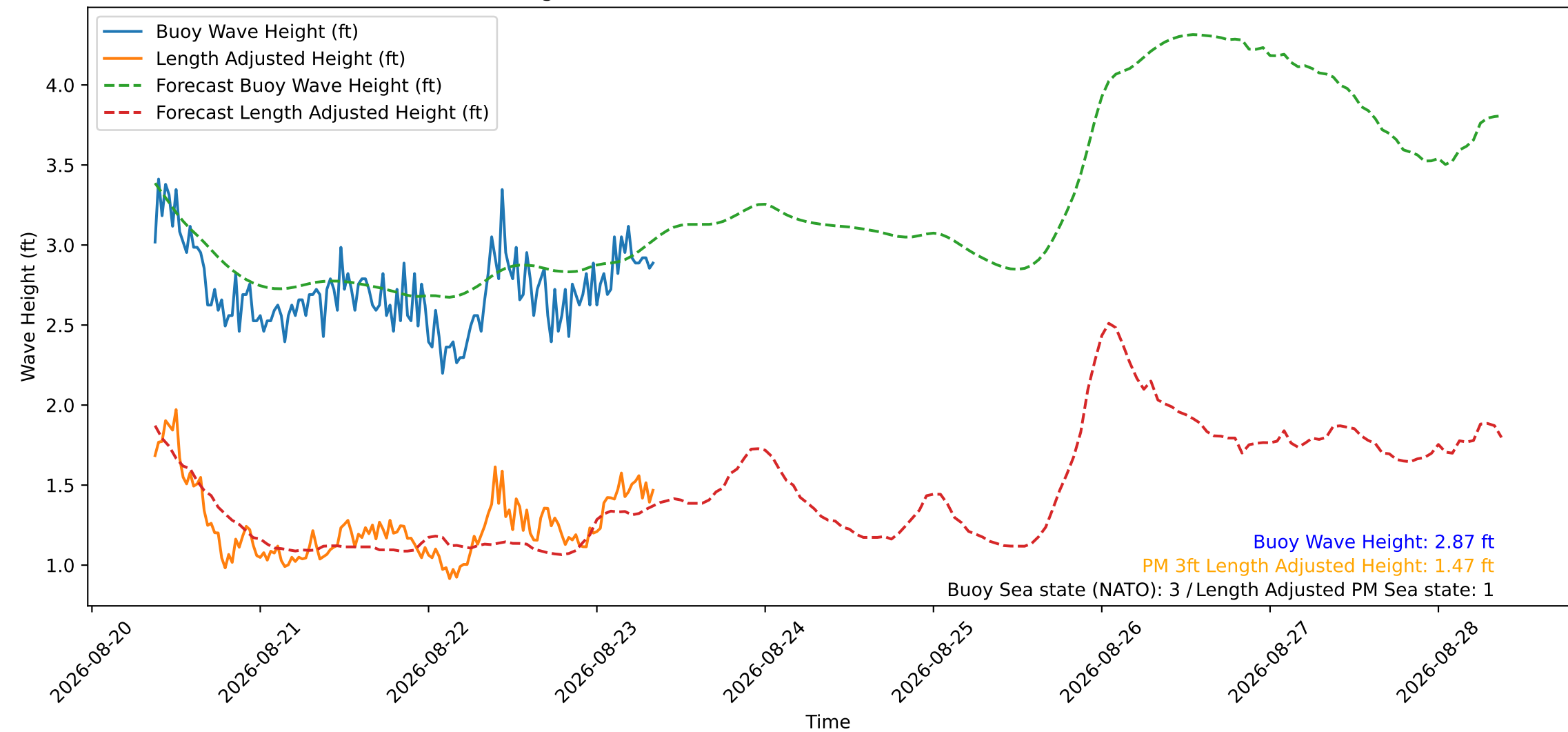
Wave Heights over Time for Oceanside Harbor at 2026-08-23 08:50:29
