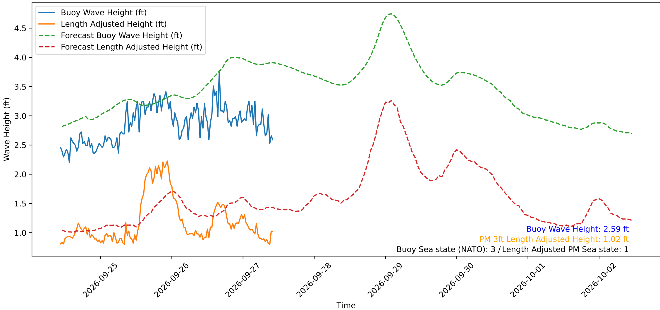
Wave Heights over Time for Oceanside Harbor at 2026-09-27 10:30:30
