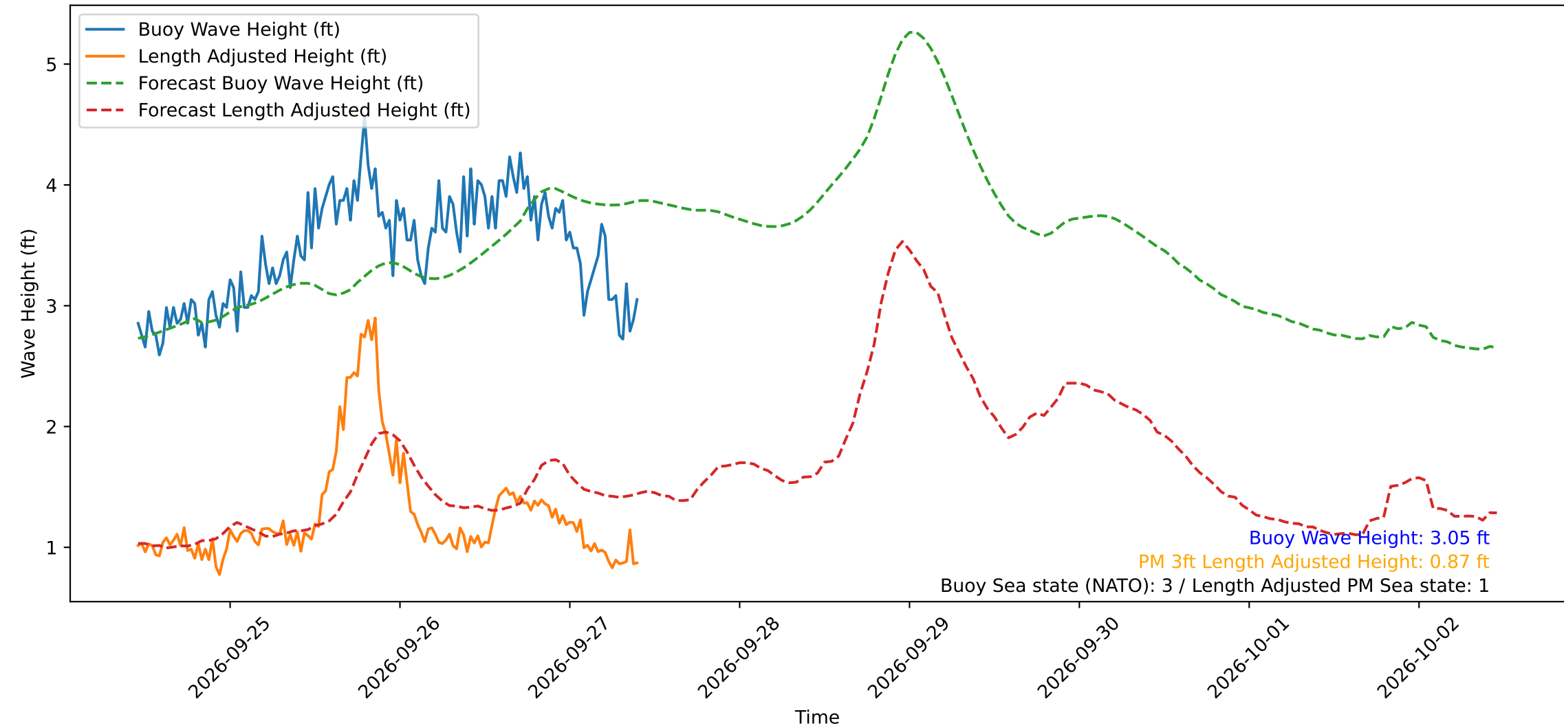
Wave Heights over Time for Green Beach at 2026-09-27 10:31:13
