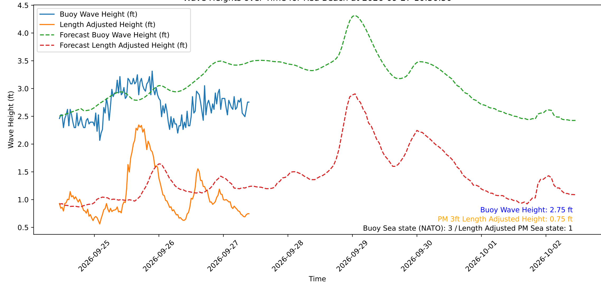
Wave Heights over Time for Red Beach at 2026-09-27 10:30:50
