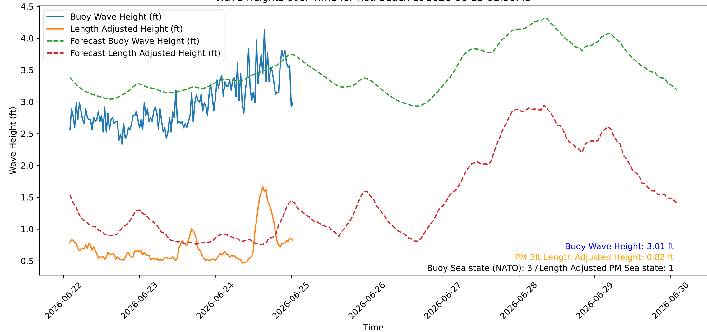
Wave Heights over Time for Red Beach at 2026-06-25 01:30:45
