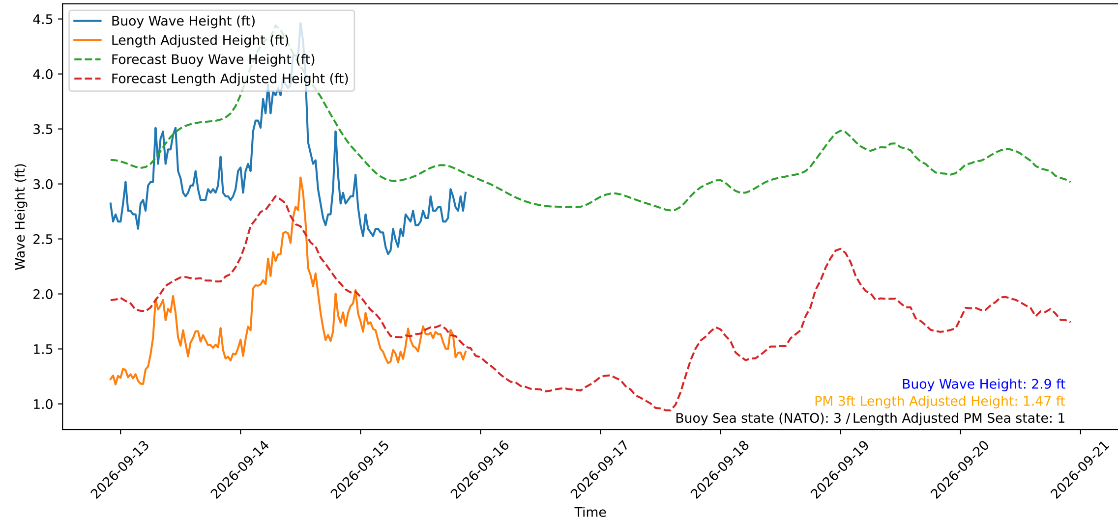
Wave Heights over Time for Oceanside Harbor at 2026-09-15 21:50:31
