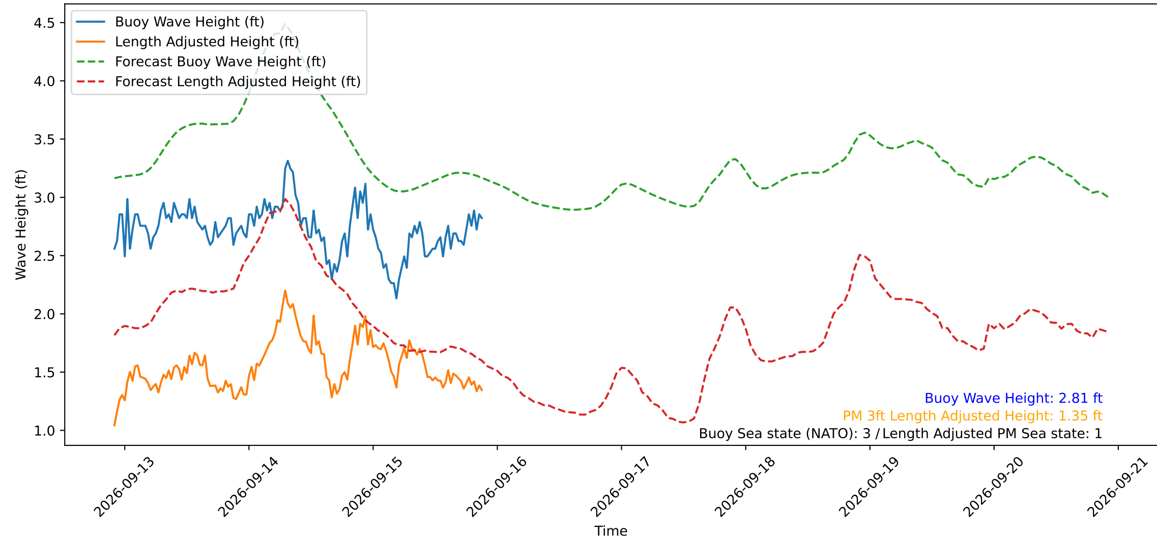
Wave Heights over Time for Green Beach at 2026-09-15 21:51:15
