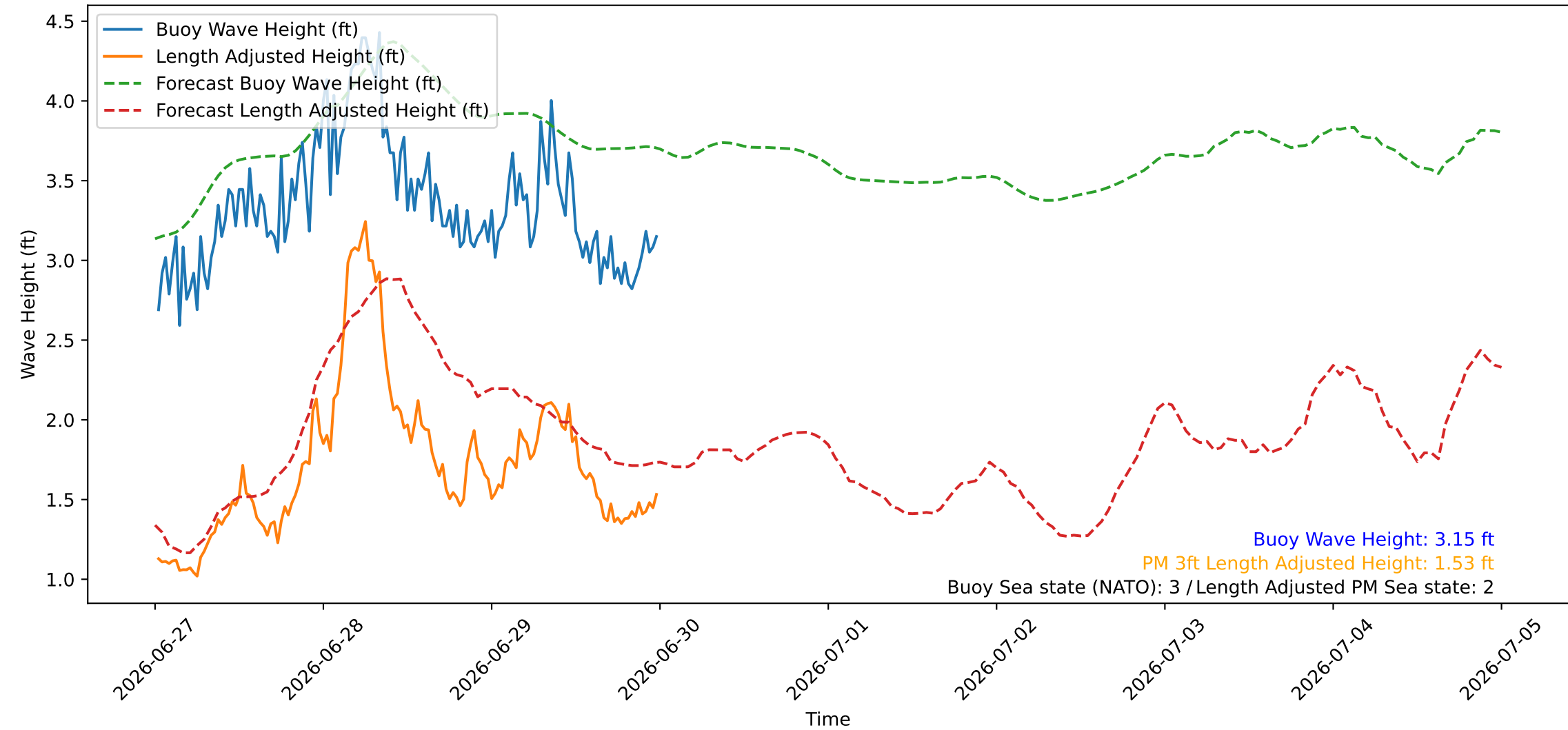
Wave Heights over Time for Oceanside Harbor at 2026-06-30 00:20:26
