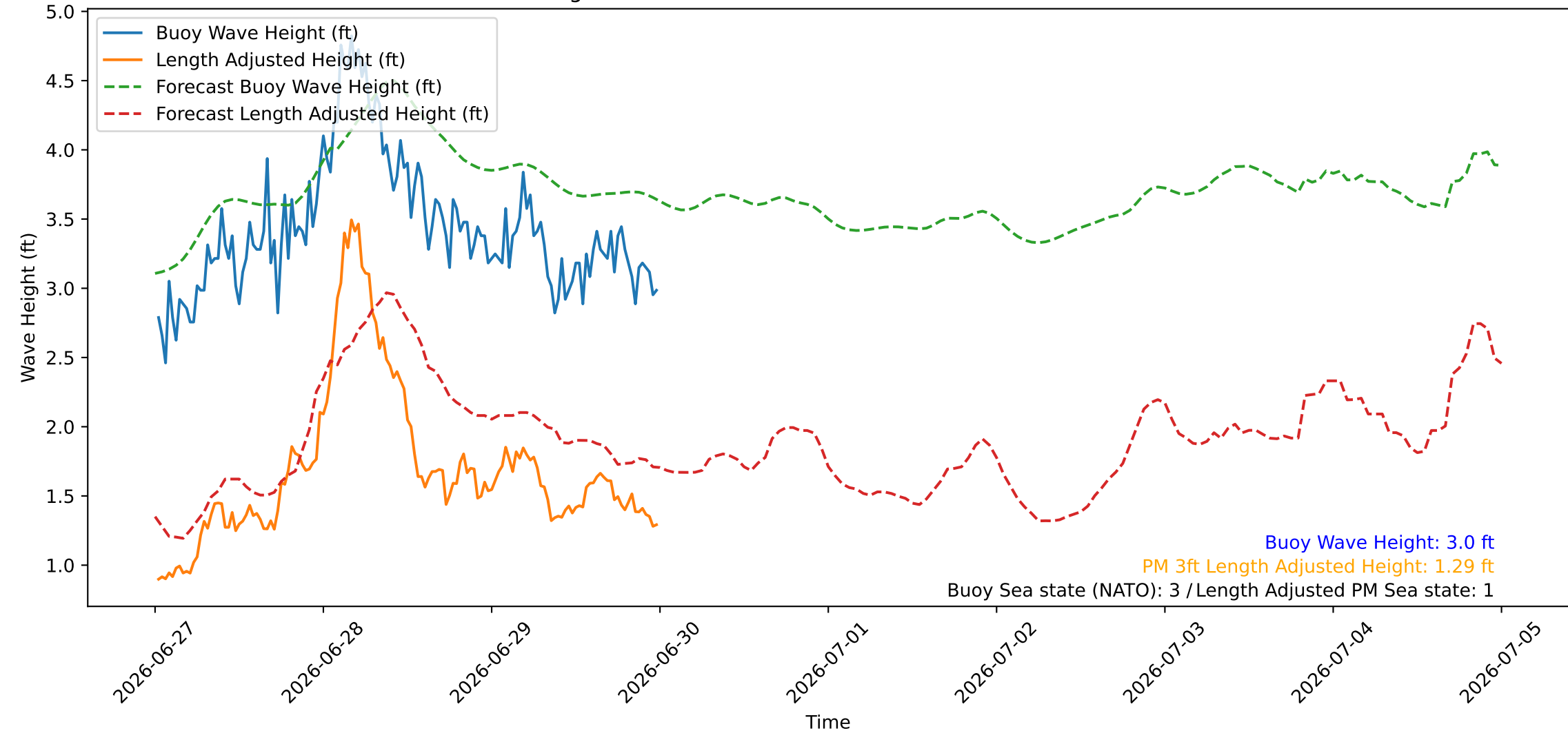
Wave Heights over Time for Green Beach at 2026-06-30 00:21:09
