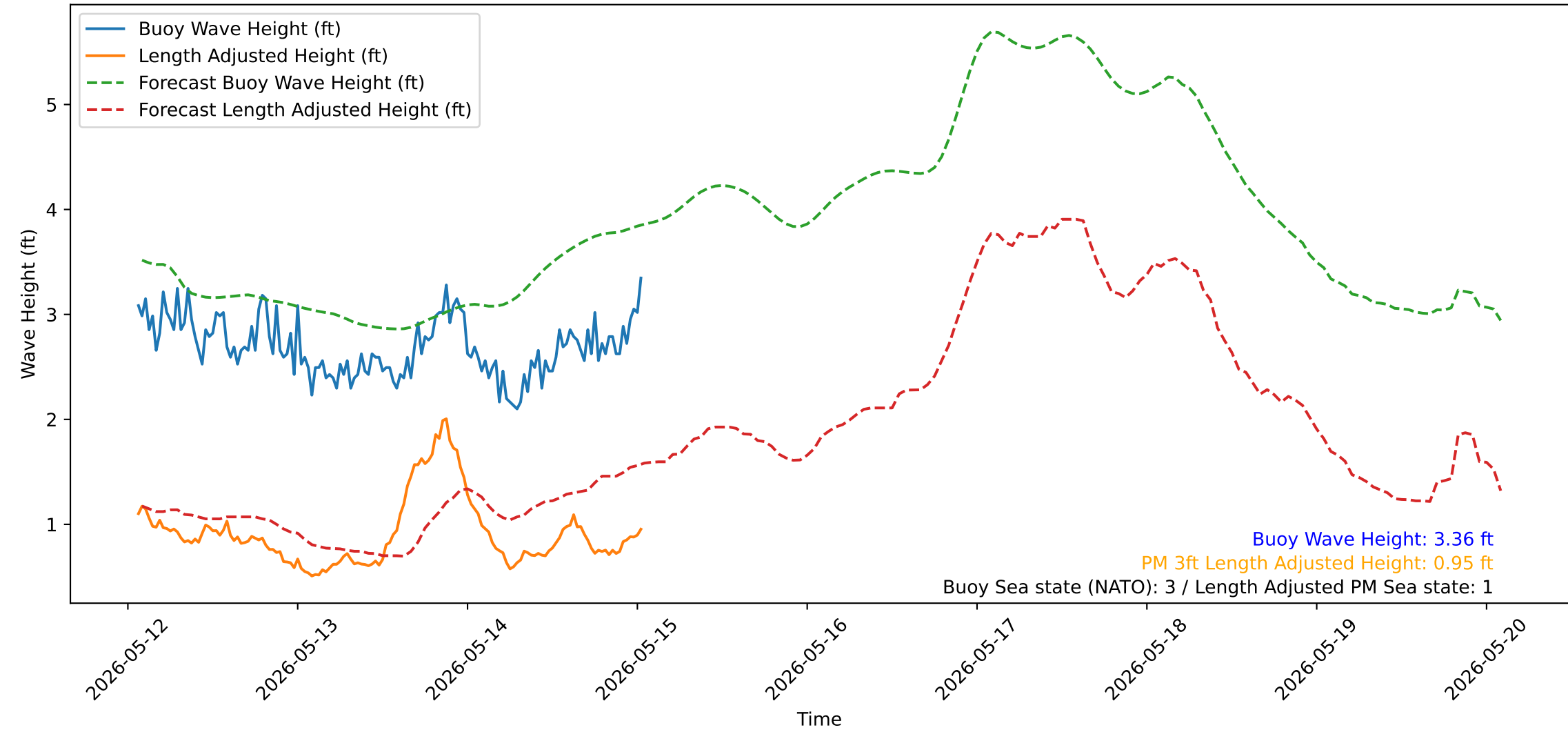
Wave Heights over Time for Green Beach at 2026-05-15 01:31:15
