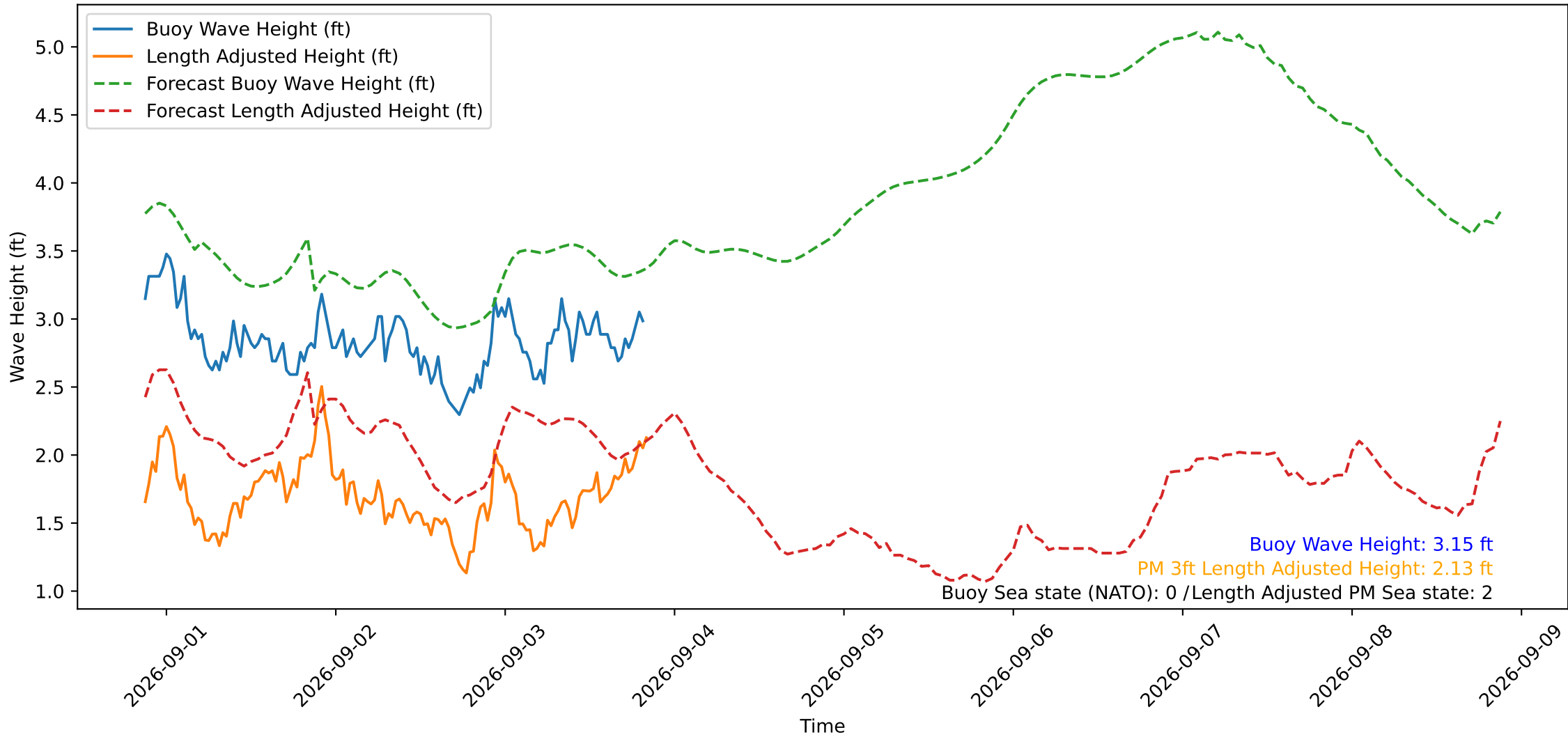
Wave Heights over Time for Red Beach at 2026-09-03 20:40:49
