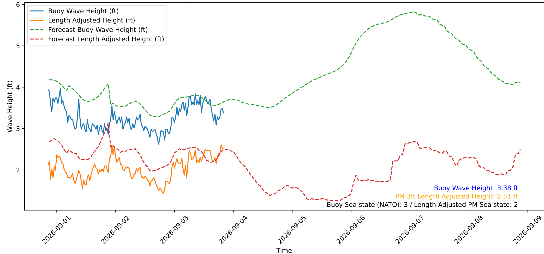
Wave Heights over Time for Oceanside Harbor at 2026-09-03 20:40:29
