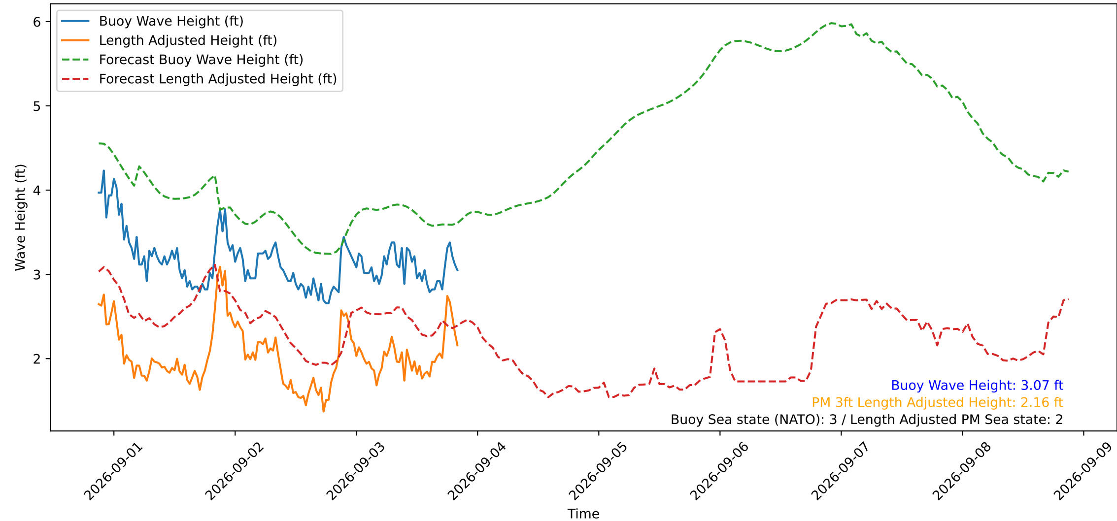
Wave Heights over Time for Green Beach at 2026-09-03 20:41:12
