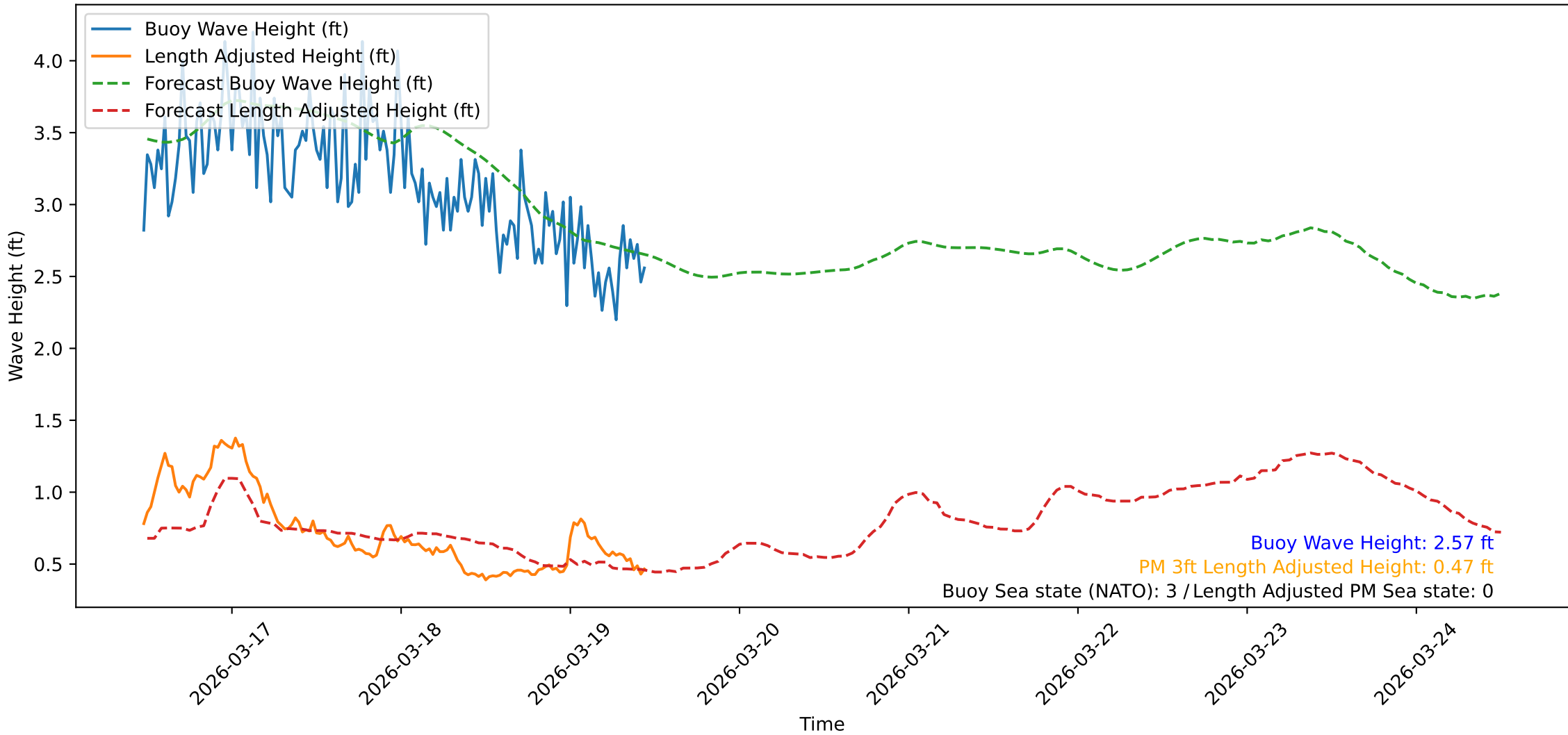
Wave Heights over Time for Green Beach at 2026-03-19 11:31:09
