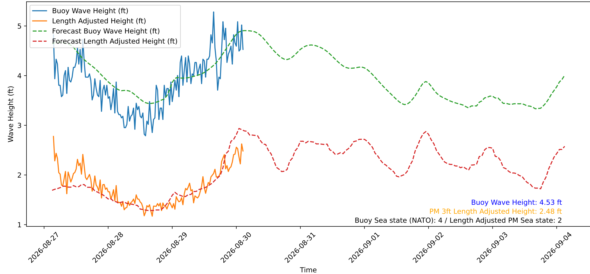
Wave Heights over Time for Oceanside Harbor at 2026-08-30 03:20:30
