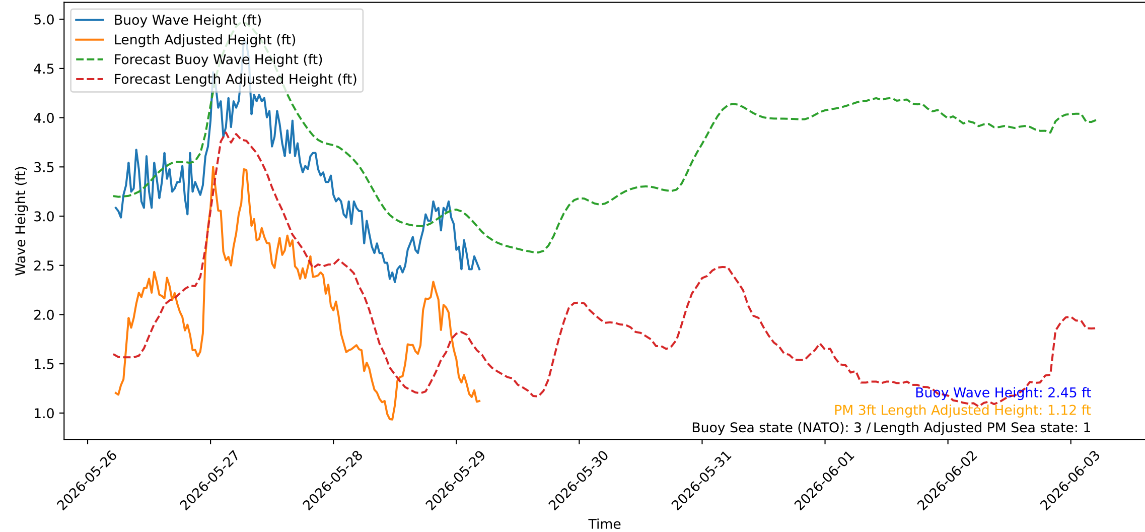
Wave Heights over Time for Red Beach at 2026-05-29 05:10:40
