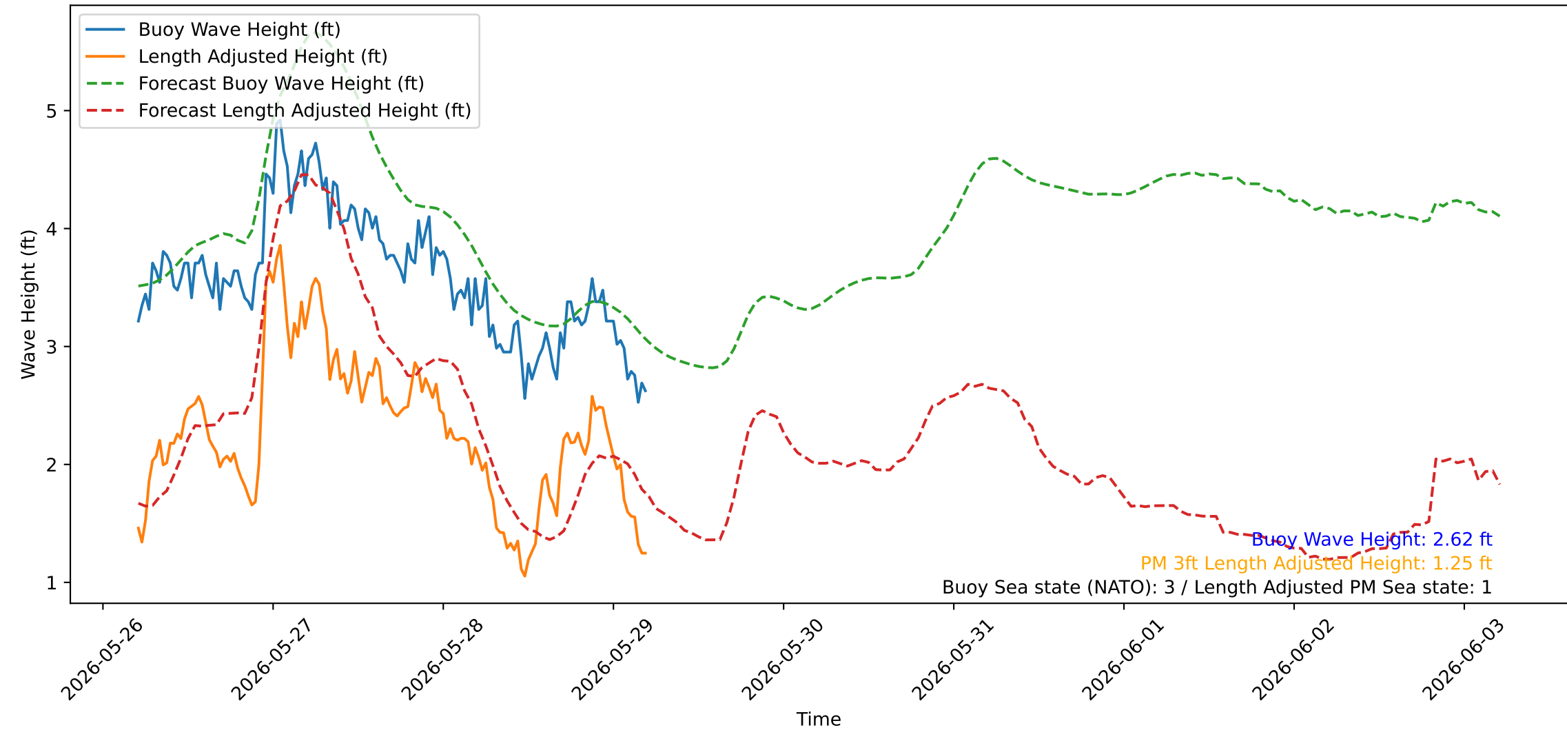
Wave Heights over Time for Green Beach at 2026-05-29 05:11:02
