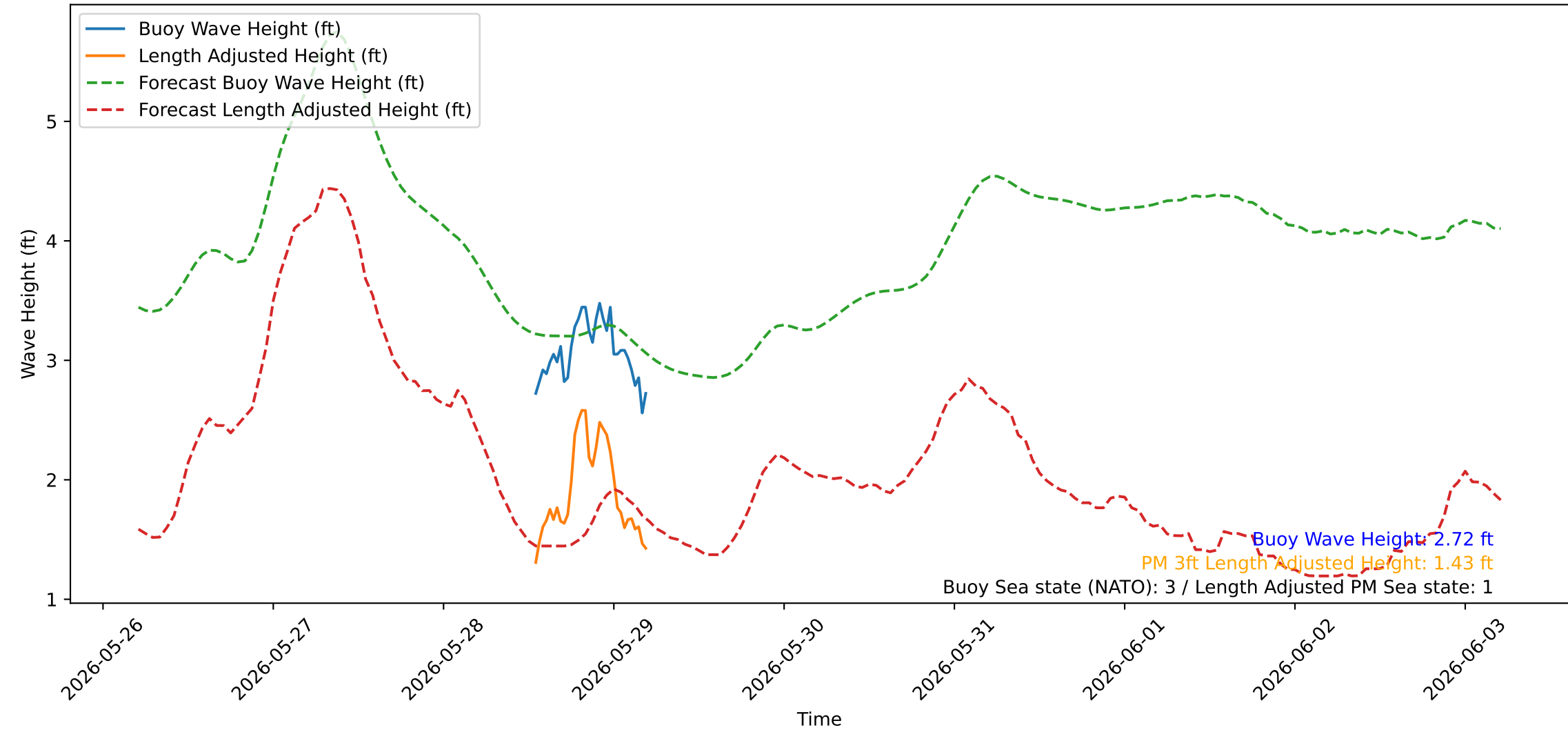
Wave Heights over Time for Oceanside Harbor at 2026-05-29 05:10:21
