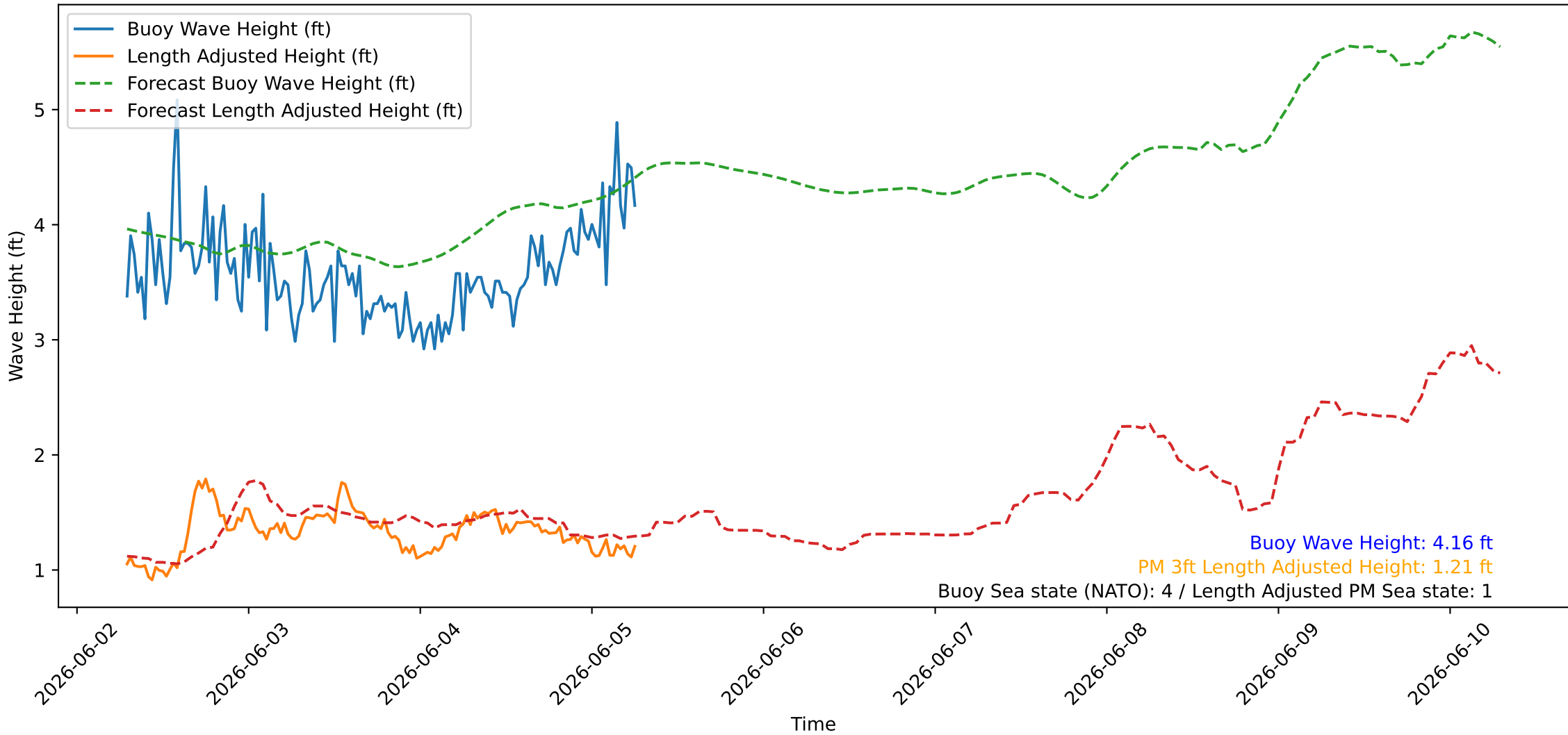
Wave Heights over Time for Oceanside Harbor at 2026-06-05 07:00:26
