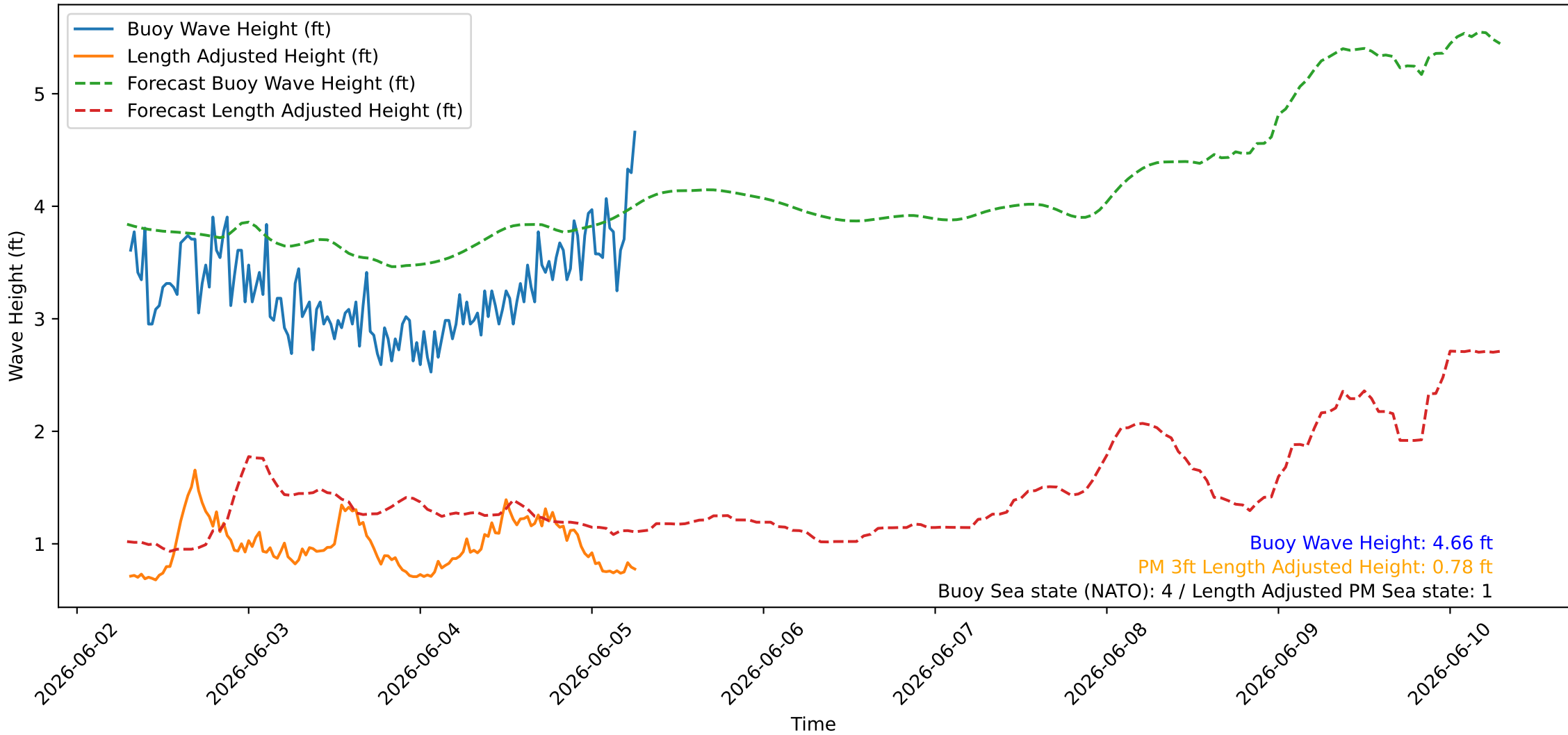
Wave Heights over Time for Red Beach at 2026-06-05 07:00:45
