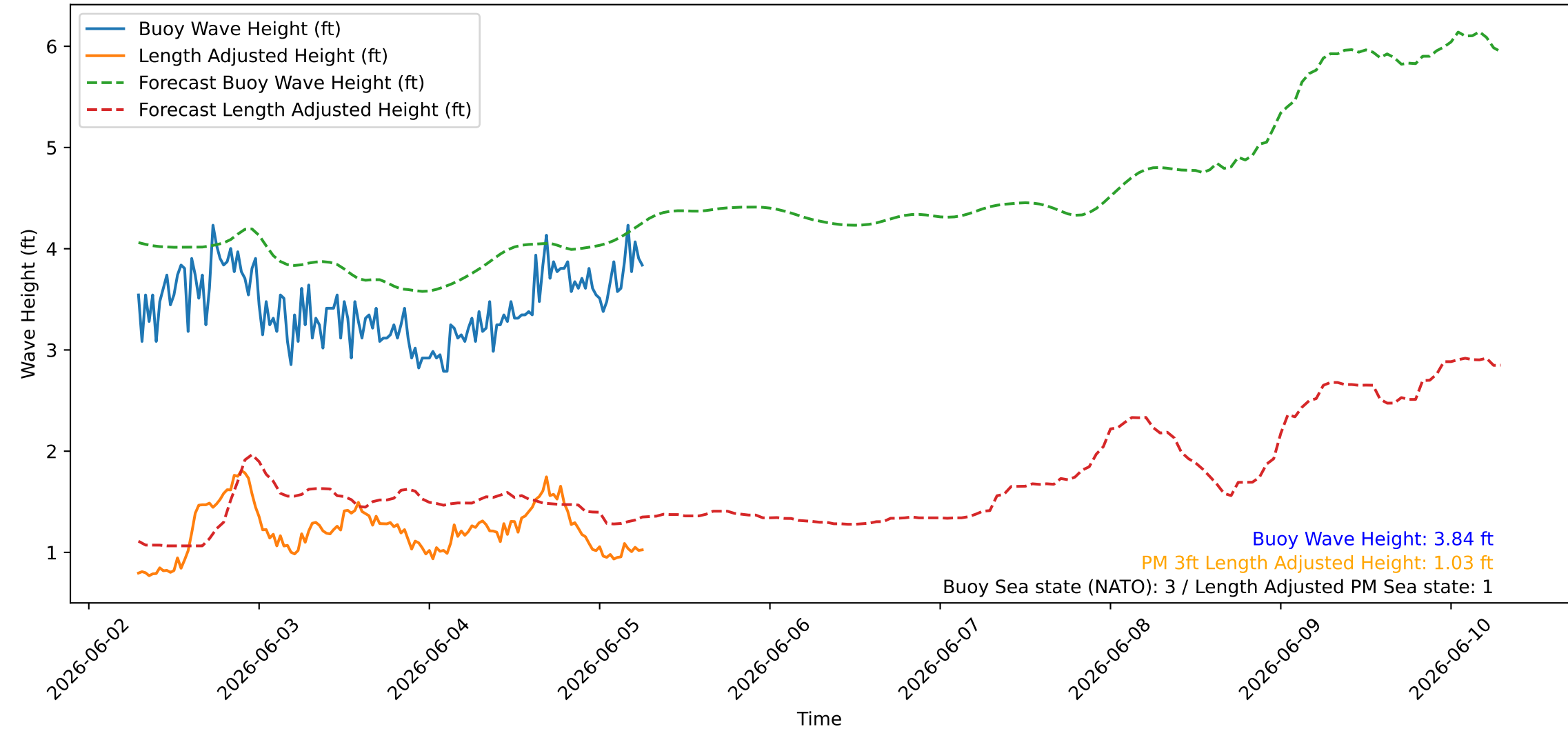
Wave Heights over Time for Green Beach at 2026-06-05 07:01:07
