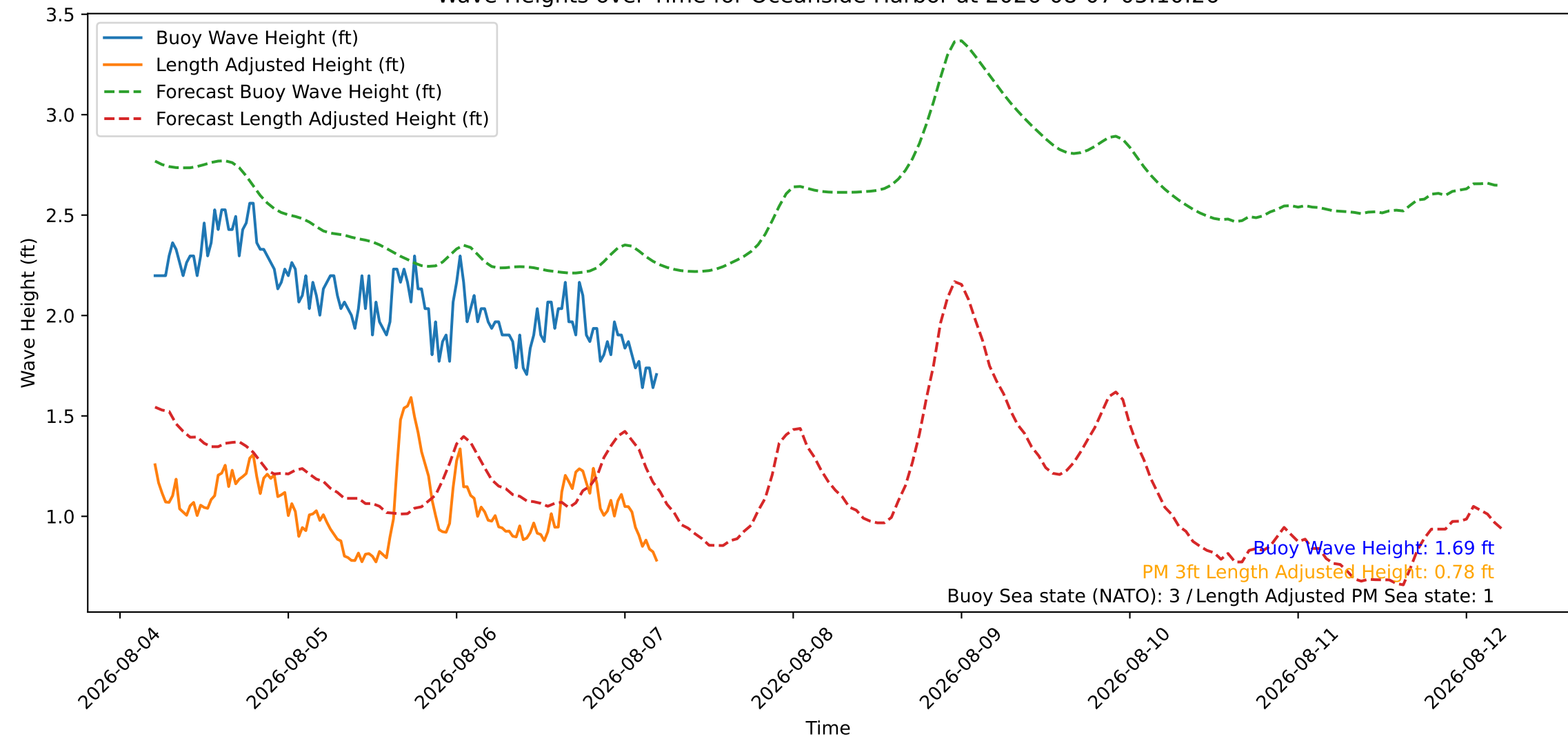
Wave Heights over Time for Oceanside Harbor at 2026-08-07 05:10:26
