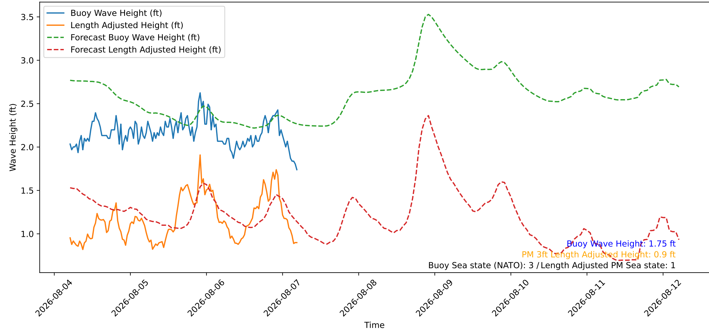
Wave Heights over Time for Green Beach at 2026-08-07 05:11:08
