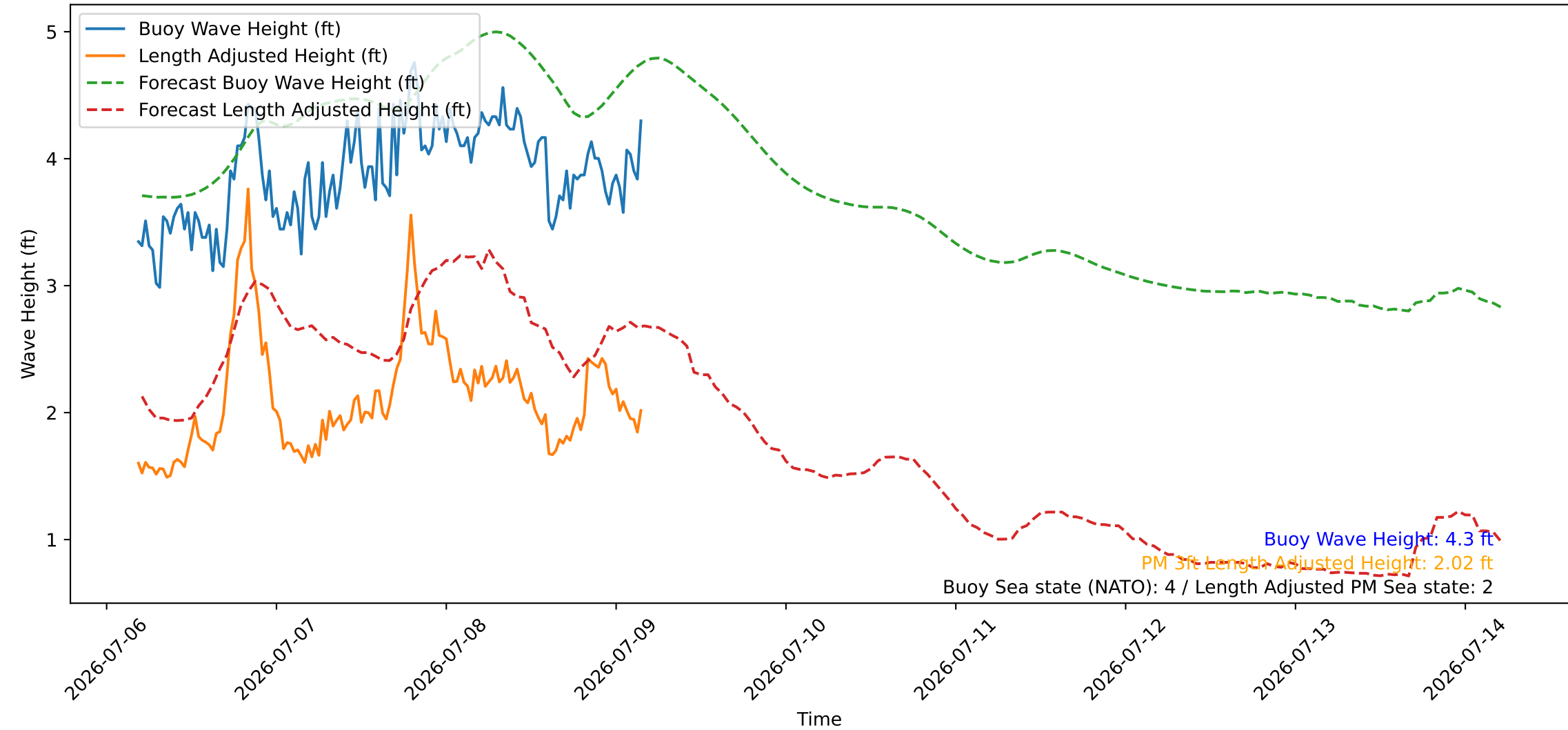
Wave Heights over Time for Green Beach at 2026-07-09 04:31:09
