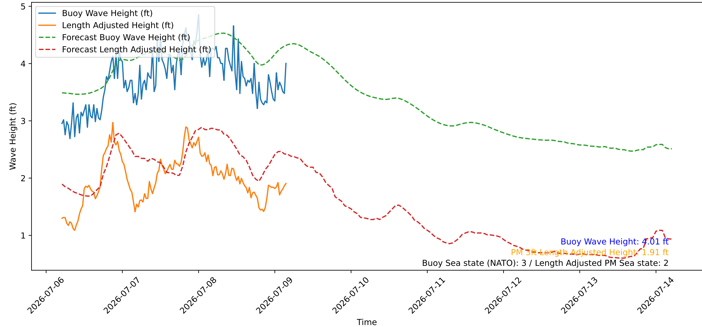
Wave Heights over Time for Red Beach at 2026-07-09 04:30:46
