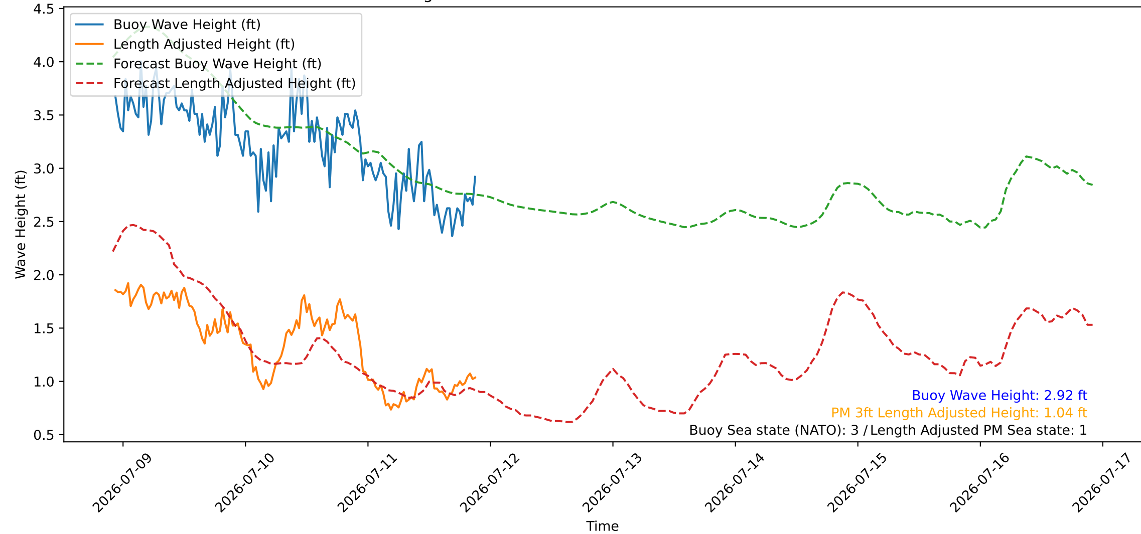
Wave Heights over Time for Red Beach at 2026-07-11 22:00:46
