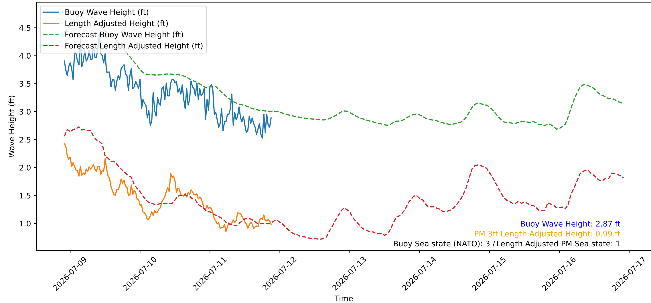
Wave Heights over Time for Green Beach at 2026-07-11 22:01:08
