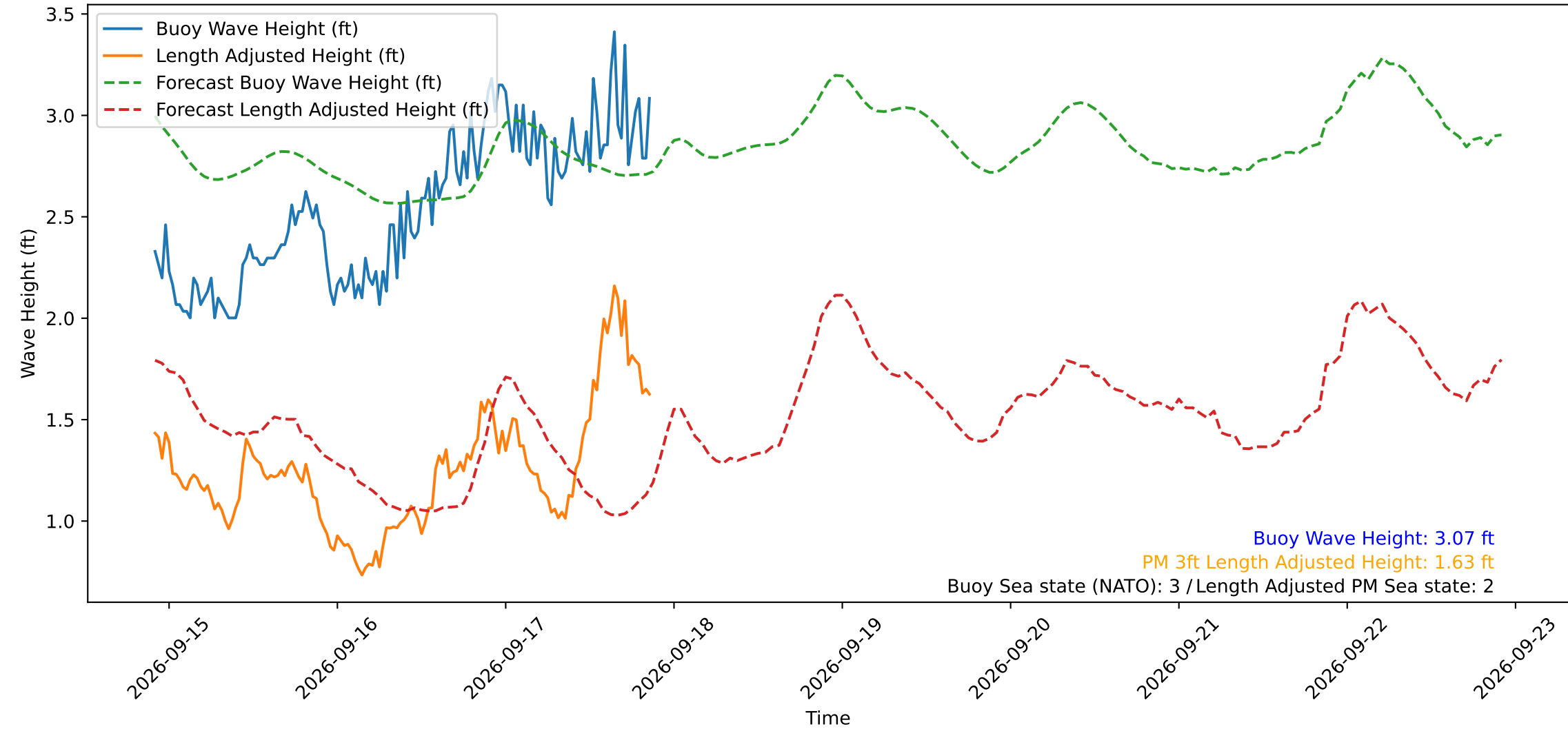
Wave Heights over Time for Red Beach at 2026-09-17 21:30:50
