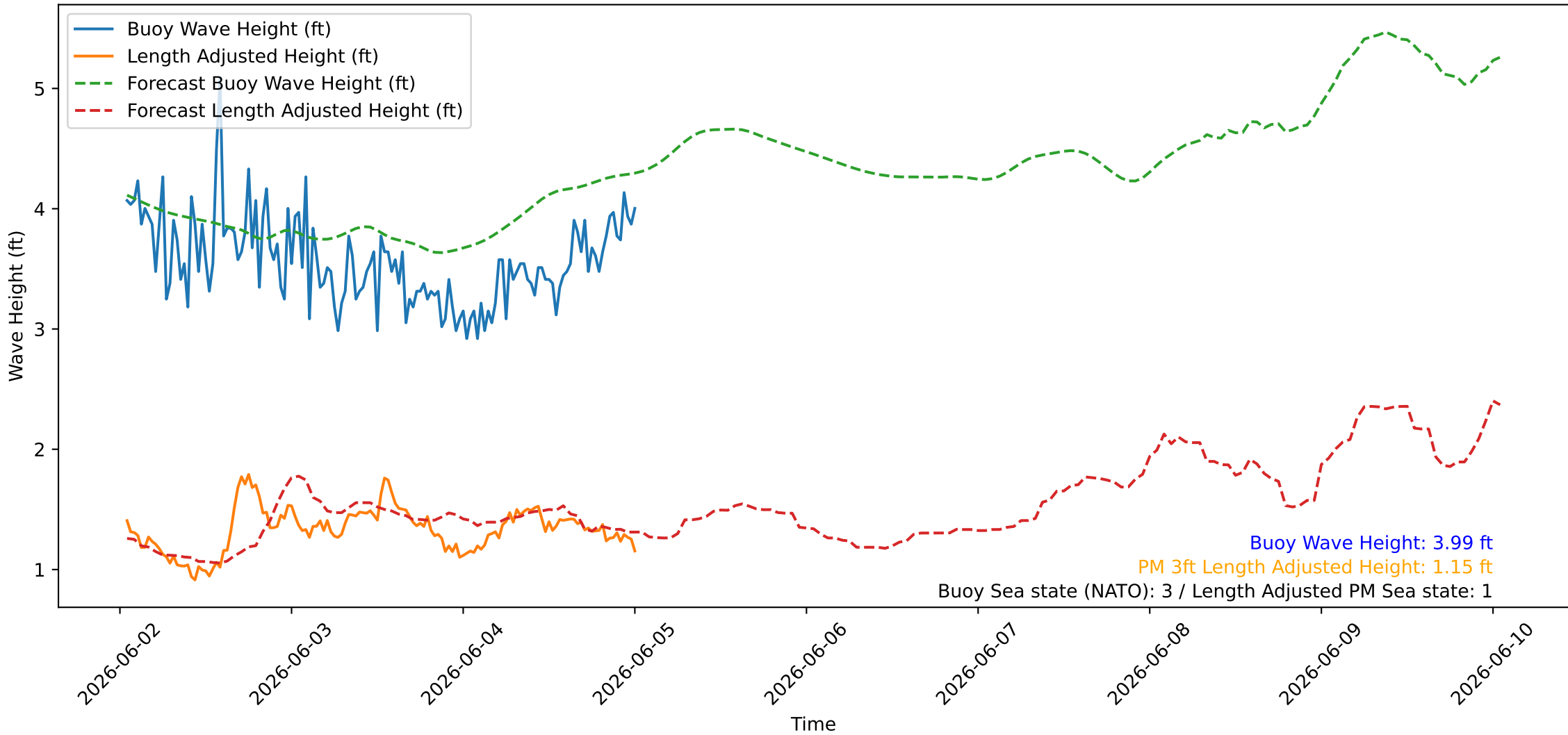
Wave Heights over Time for Oceanside Harbor at 2026-06-05 00:50:26
