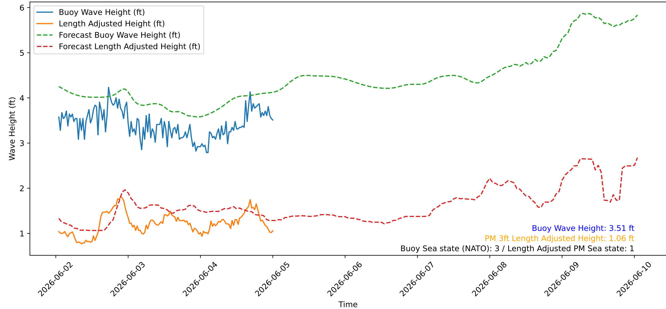
Wave Heights over Time for Green Beach at 2026-06-05 00:51:09
