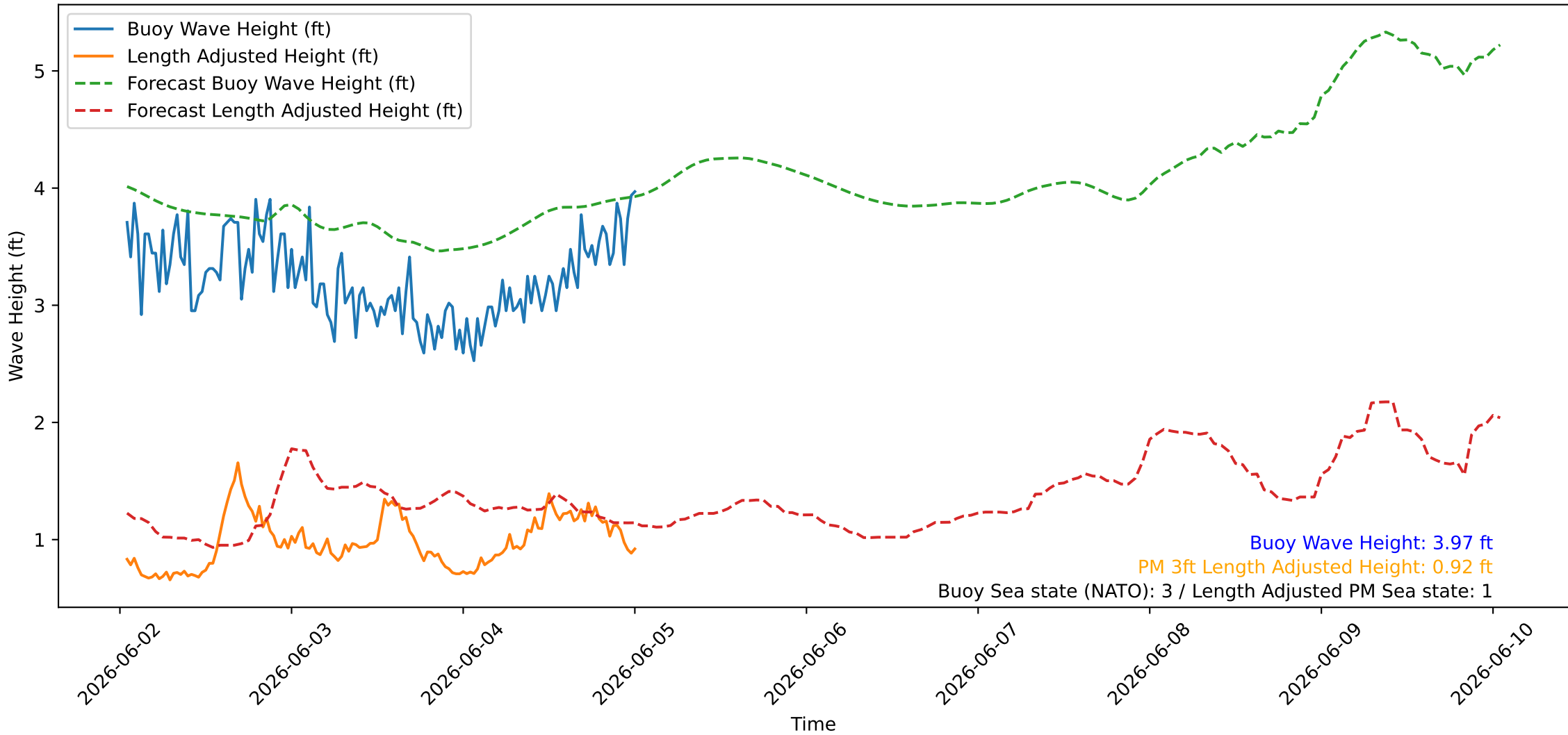
Wave Heights over Time for Red Beach at 2026-06-05 00:50:46
