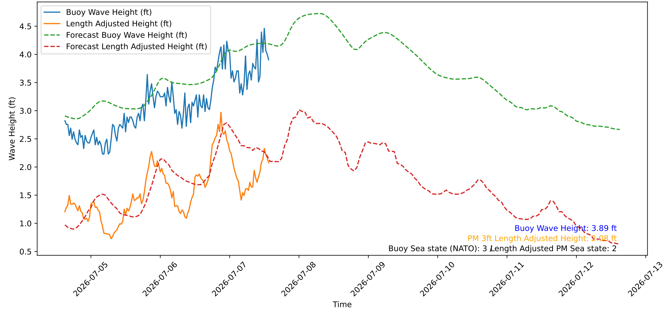
Wave Heights over Time for Red Beach at 2026-07-07 14:40:45
