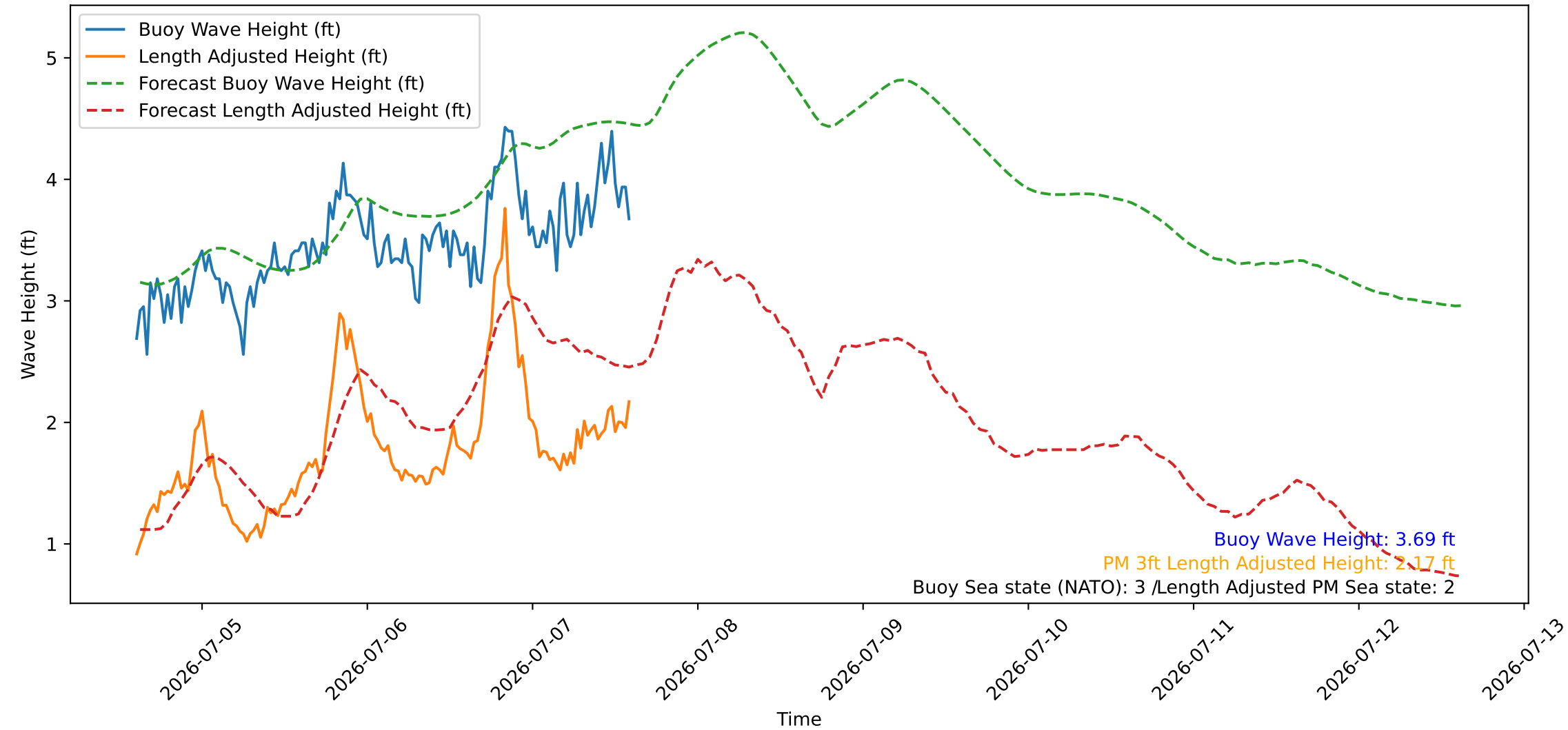
Wave Heights over Time for Green Beach at 2026-07-07 14:41:08
