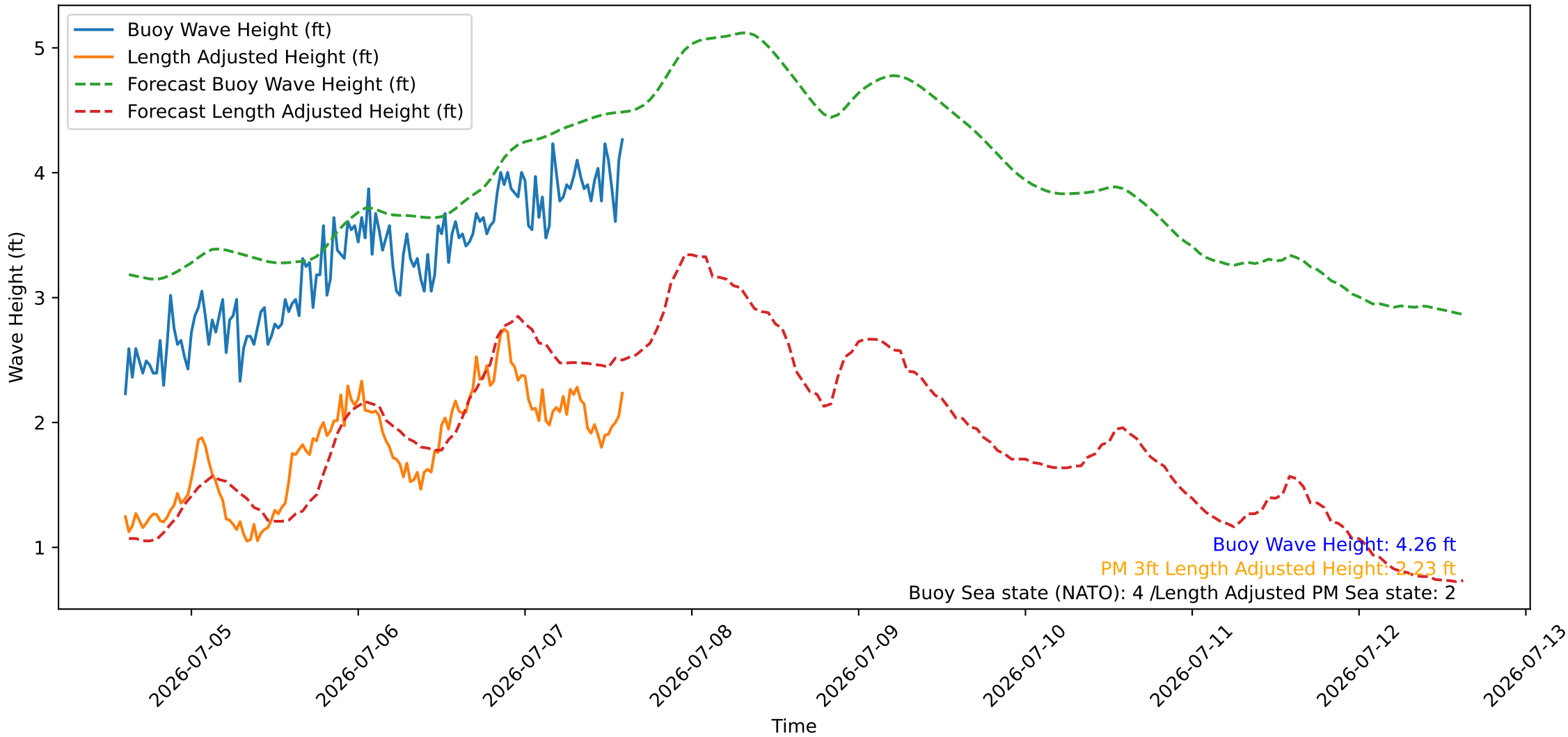
Wave Heights over Time for Oceanside Harbor at 2026-07-07 14:40:26
