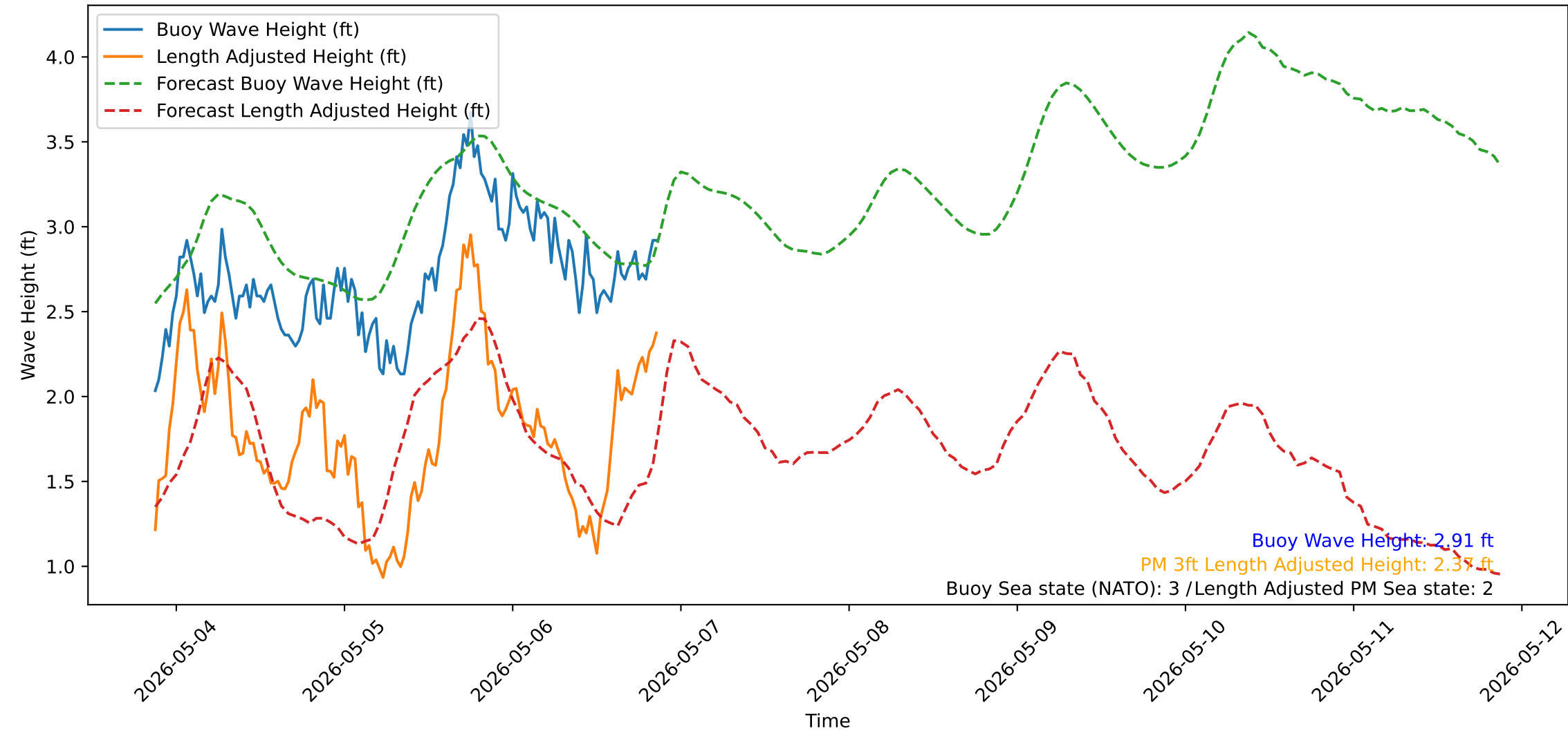
Wave Heights over Time for Green Beach at 2026-05-06 21:11:13
