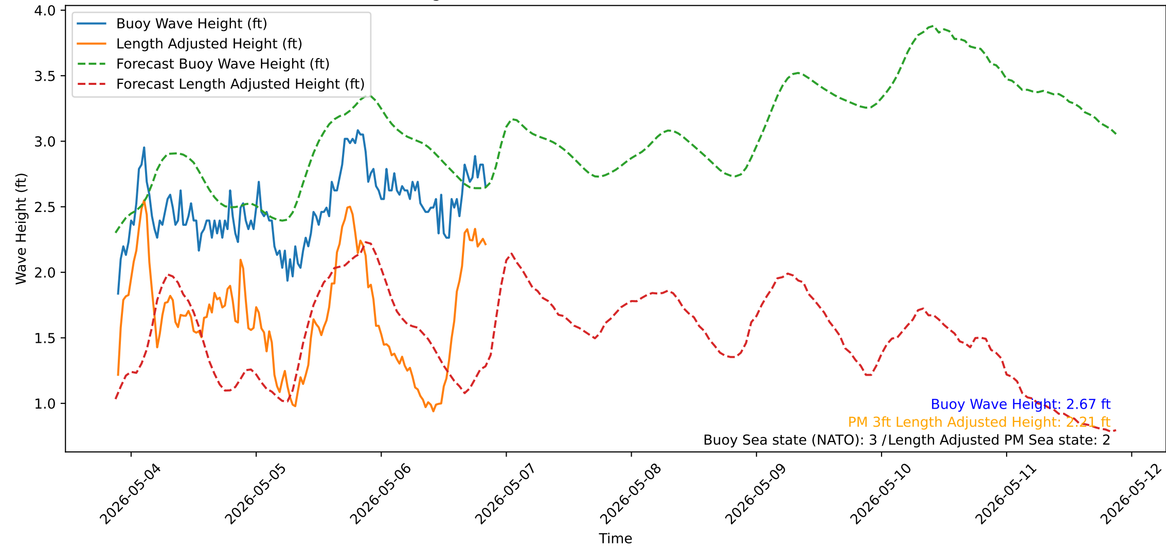
Wave Heights over Time for Red Beach at 2026-05-06 21:10:51
