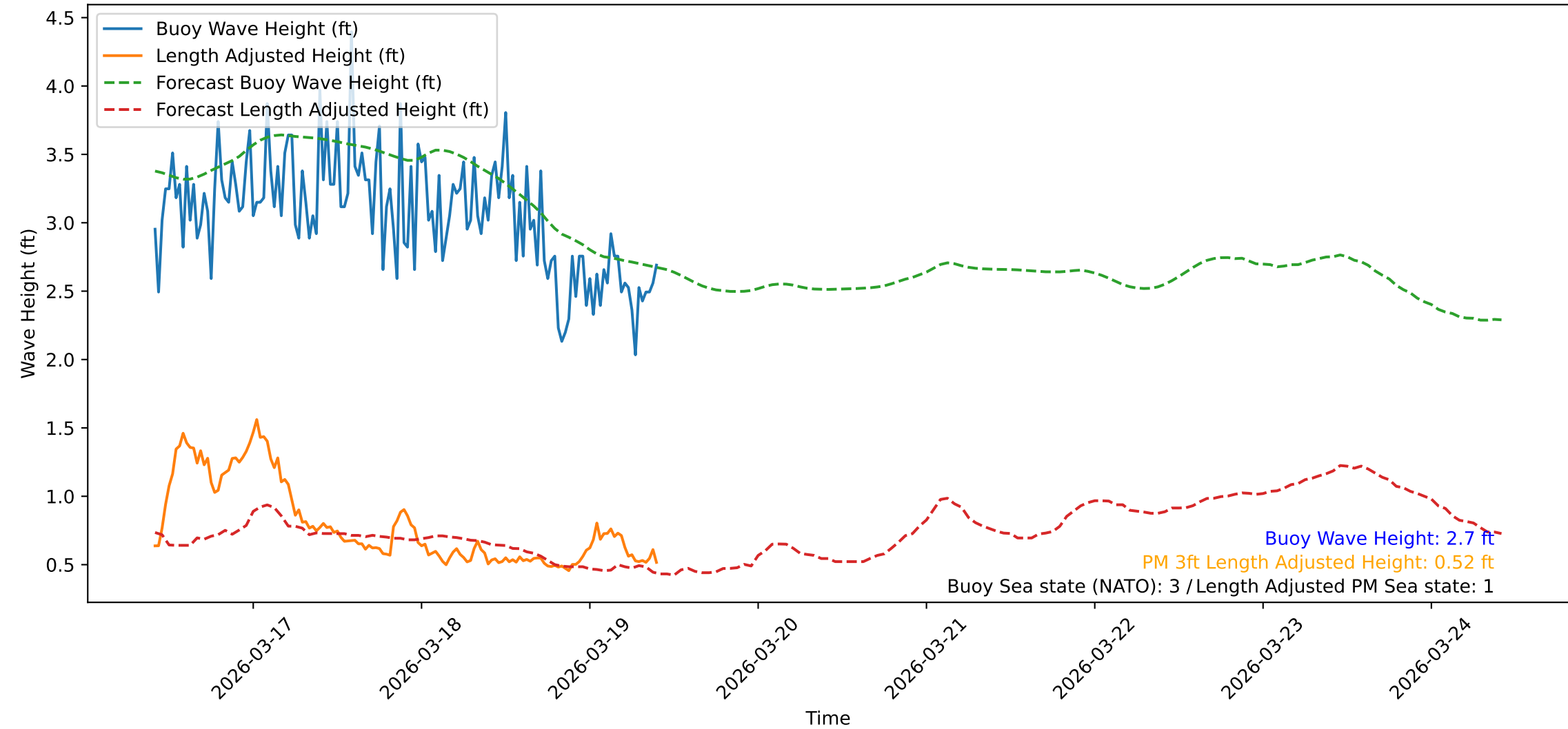
Wave Heights over Time for Oceanside Harbor at 2026-03-19 10:10:32
