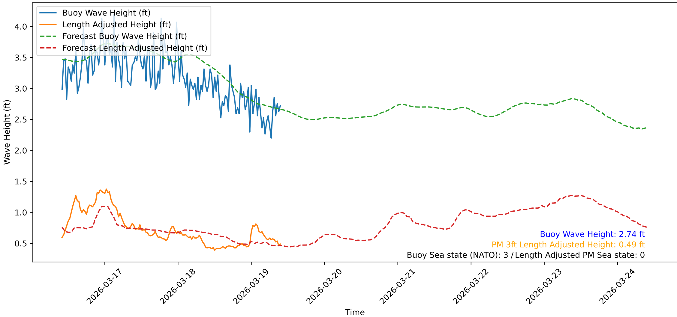
Wave Heights over Time for Green Beach at 2026-03-19 10:11:10
