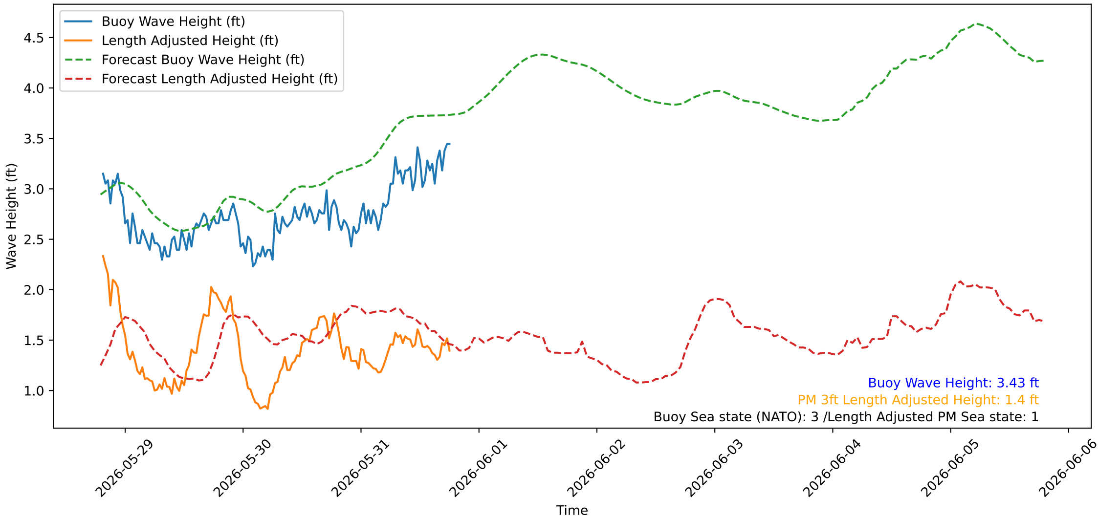
Wave Heights over Time for Red Beach at 2026-05-31 19:00:45
