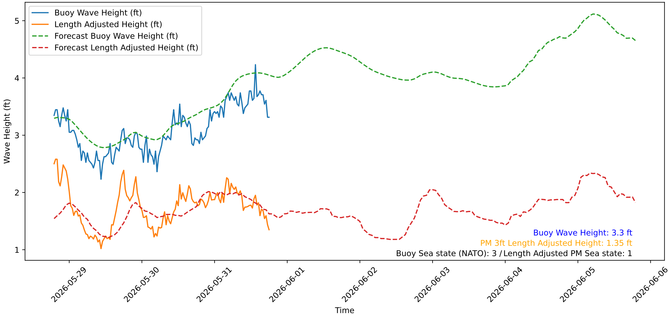
Wave Heights over Time for Oceanside Harbor at 2026-05-31 19:00:26
