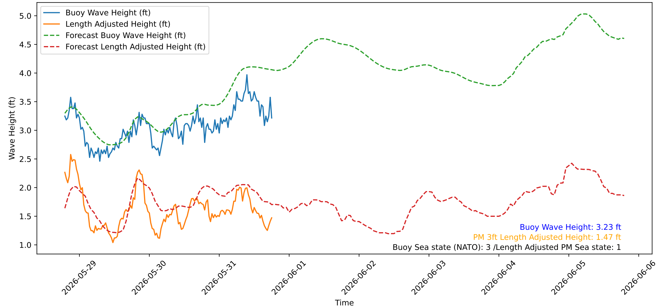
Wave Heights over Time for Green Beach at 2026-05-31 19:01:07
