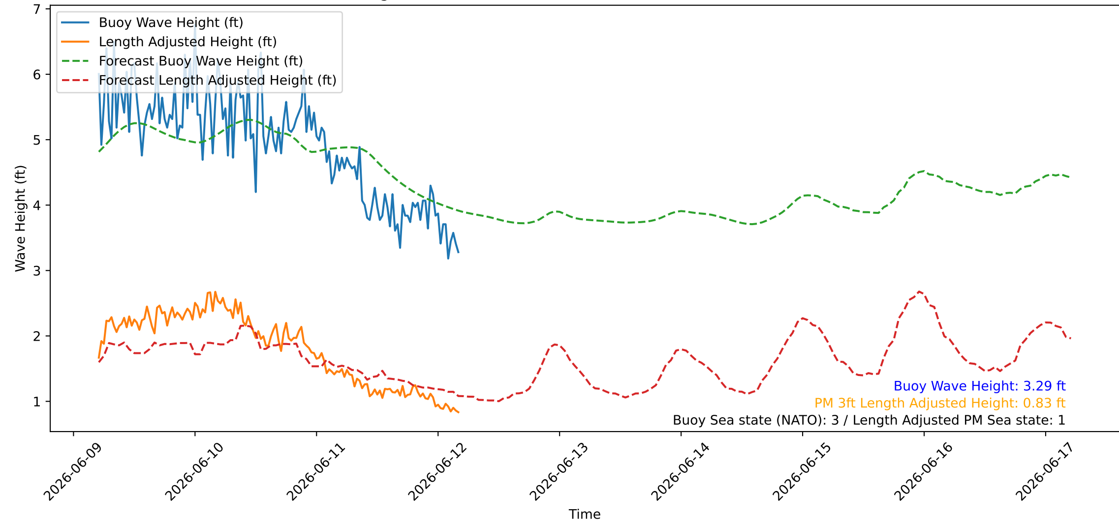
Wave Heights over Time for Oceanside Harbor at 2026-06-12 04:50:26
