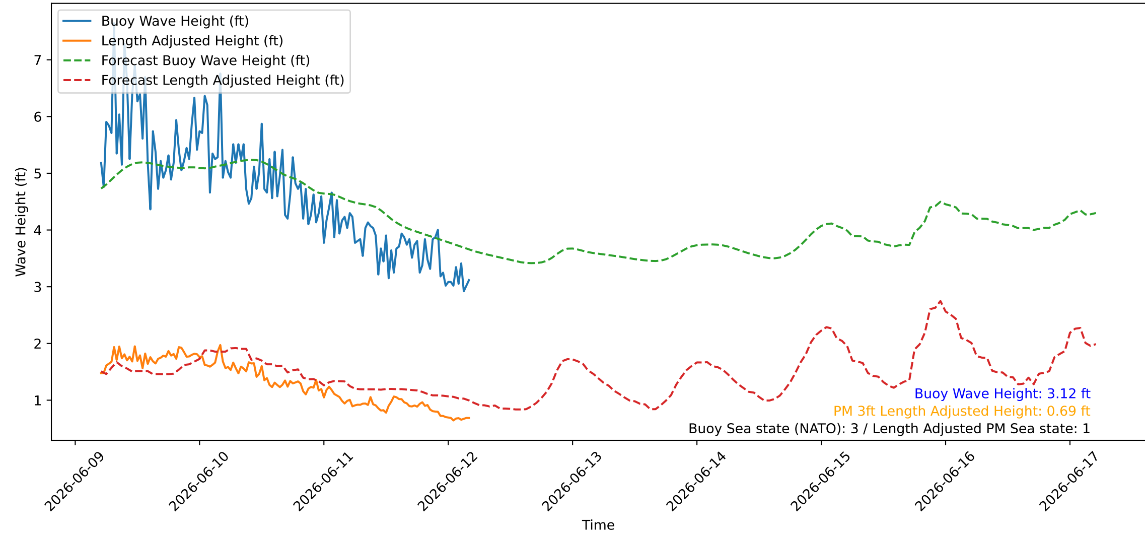
Wave Heights over Time for Red Beach at 2026-06-12 04:50:47
