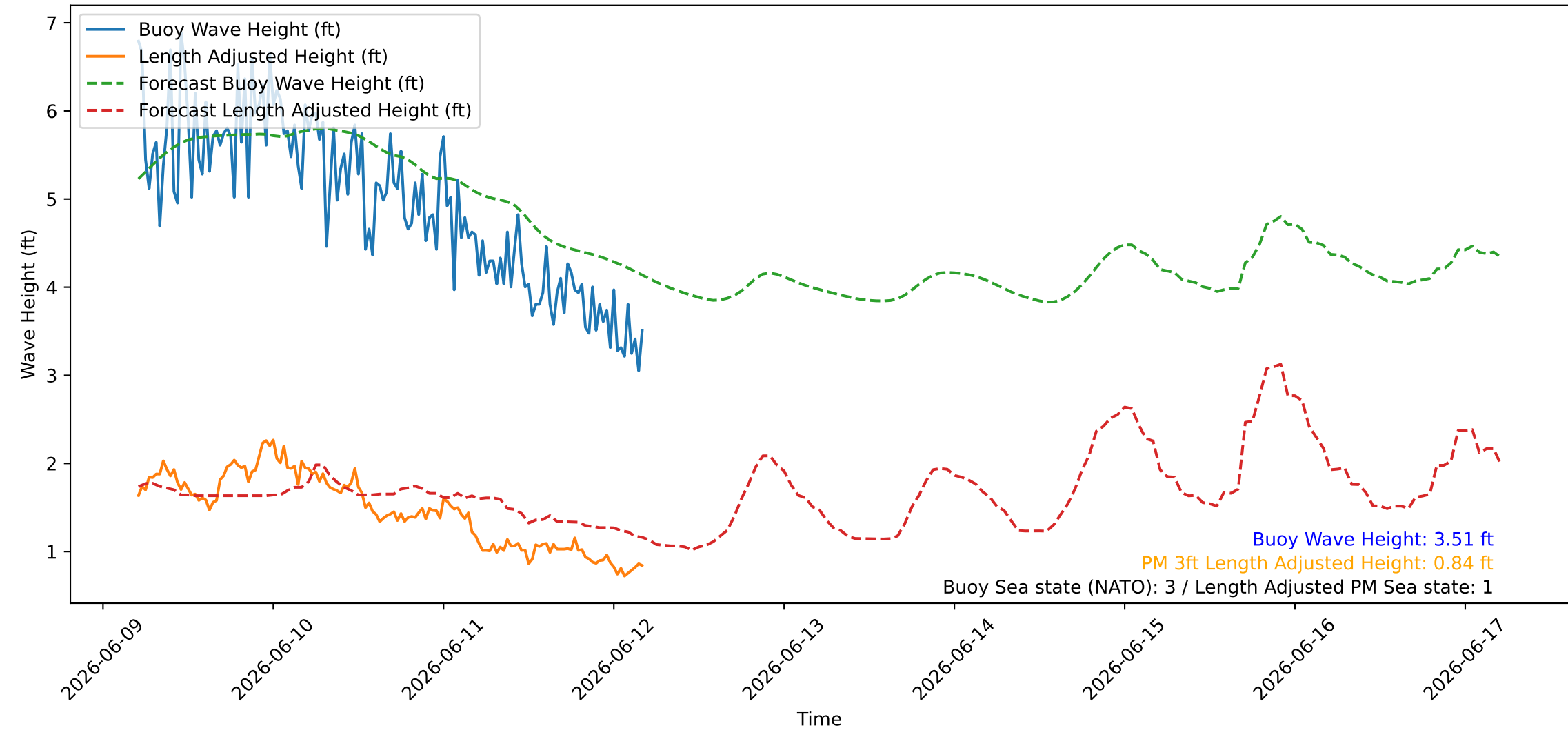
Wave Heights over Time for Green Beach at 2026-06-12 04:51:09
