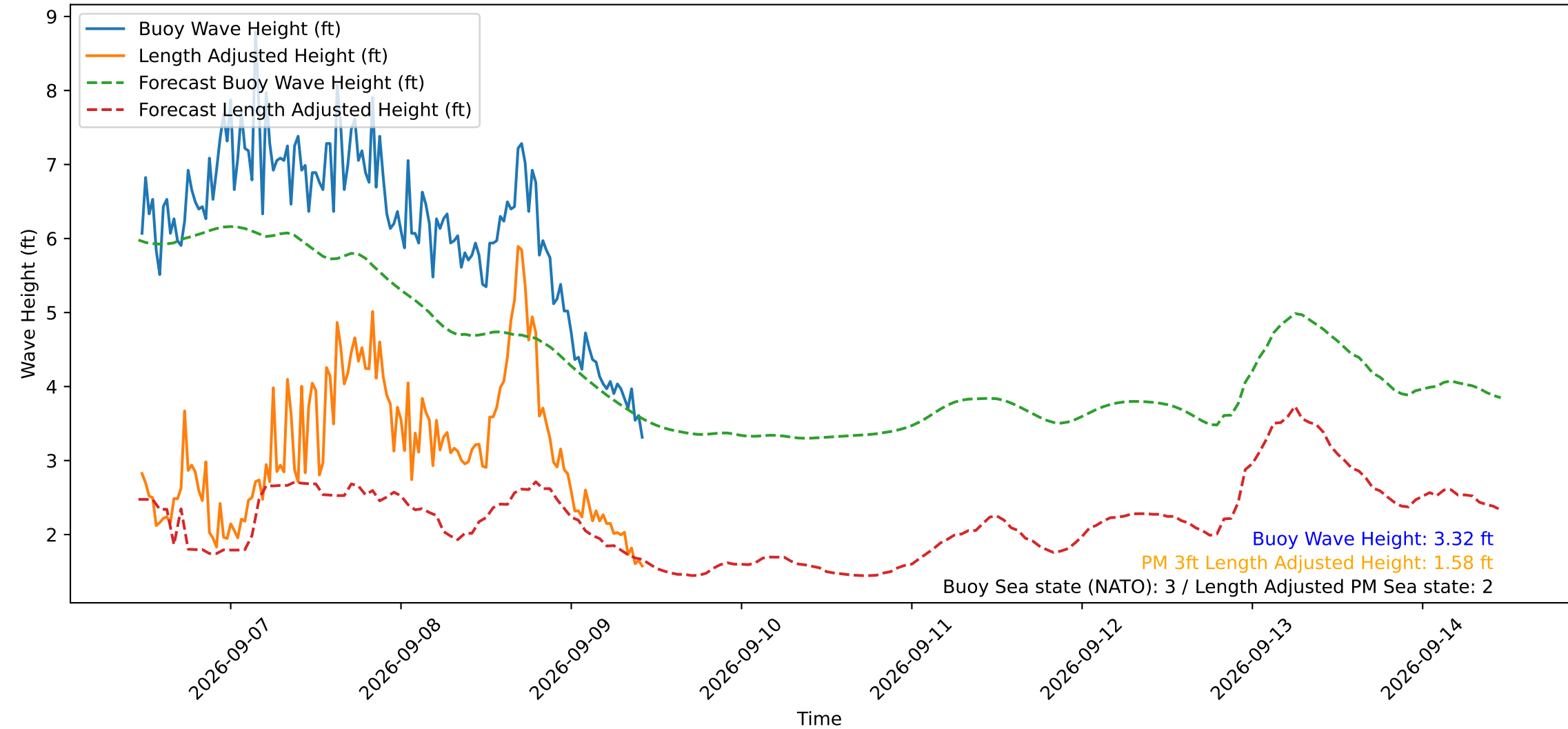
Wave Heights over Time for Green Beach at 2026-09-09 11:01:11
