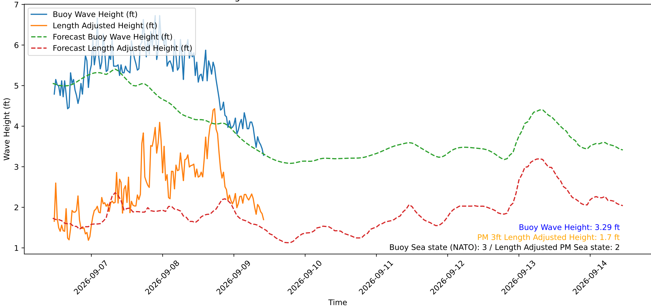
Wave Heights over Time for Red Beach at 2026-09-09 11:00:49
