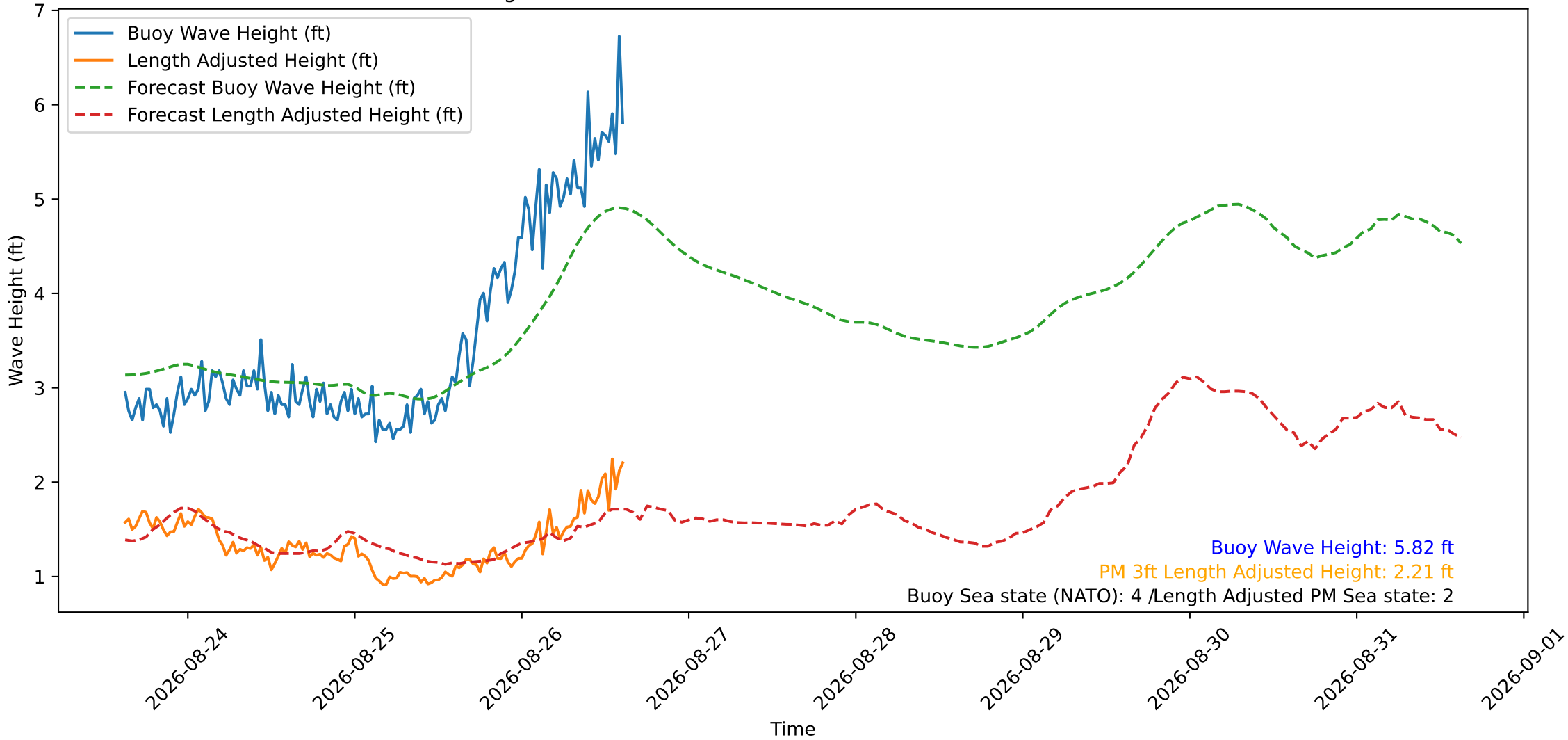
Wave Heights over Time for Oceanside Harbor at 2026-08-26 15:00:29
