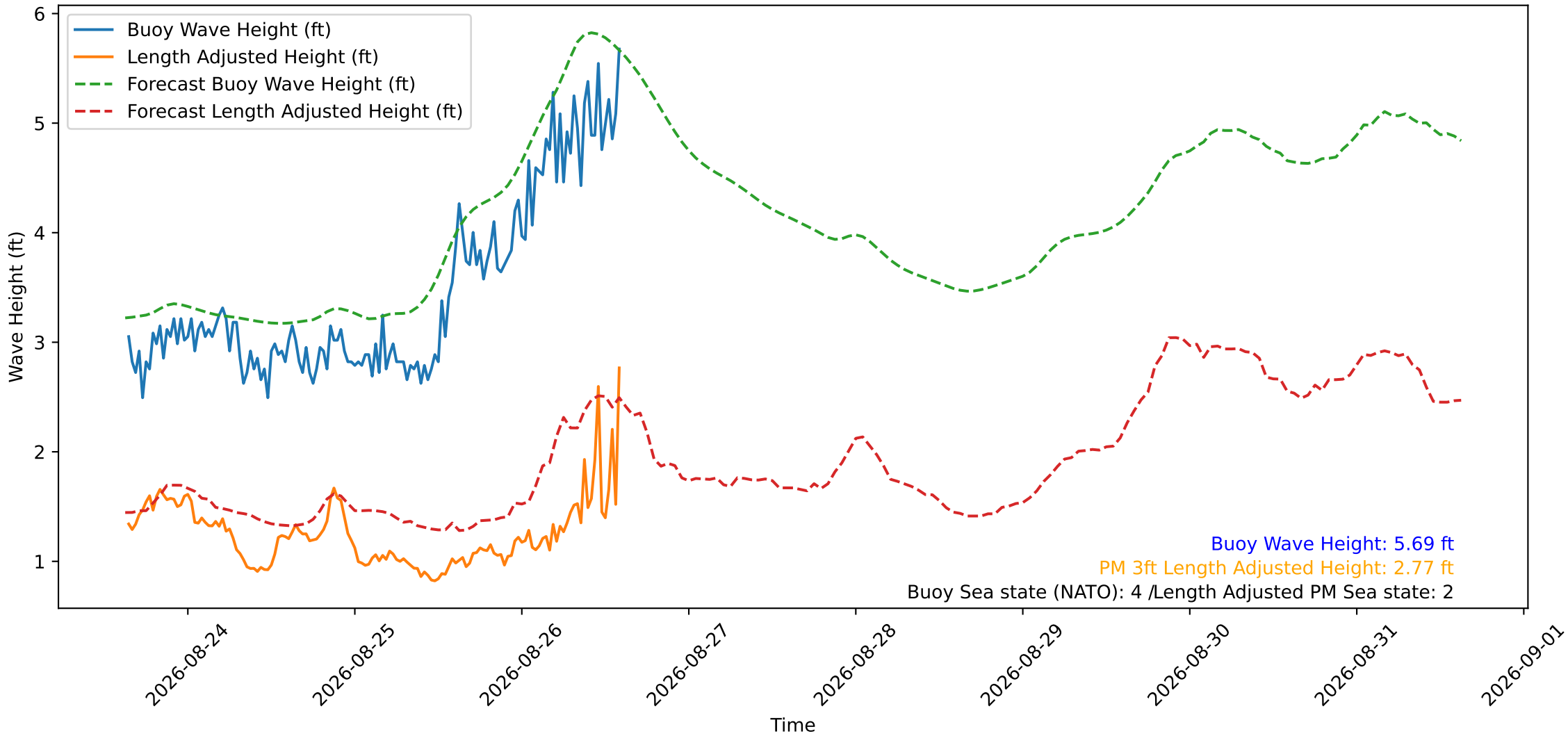
Wave Heights over Time for Green Beach at 2026-08-26 15:01:11
