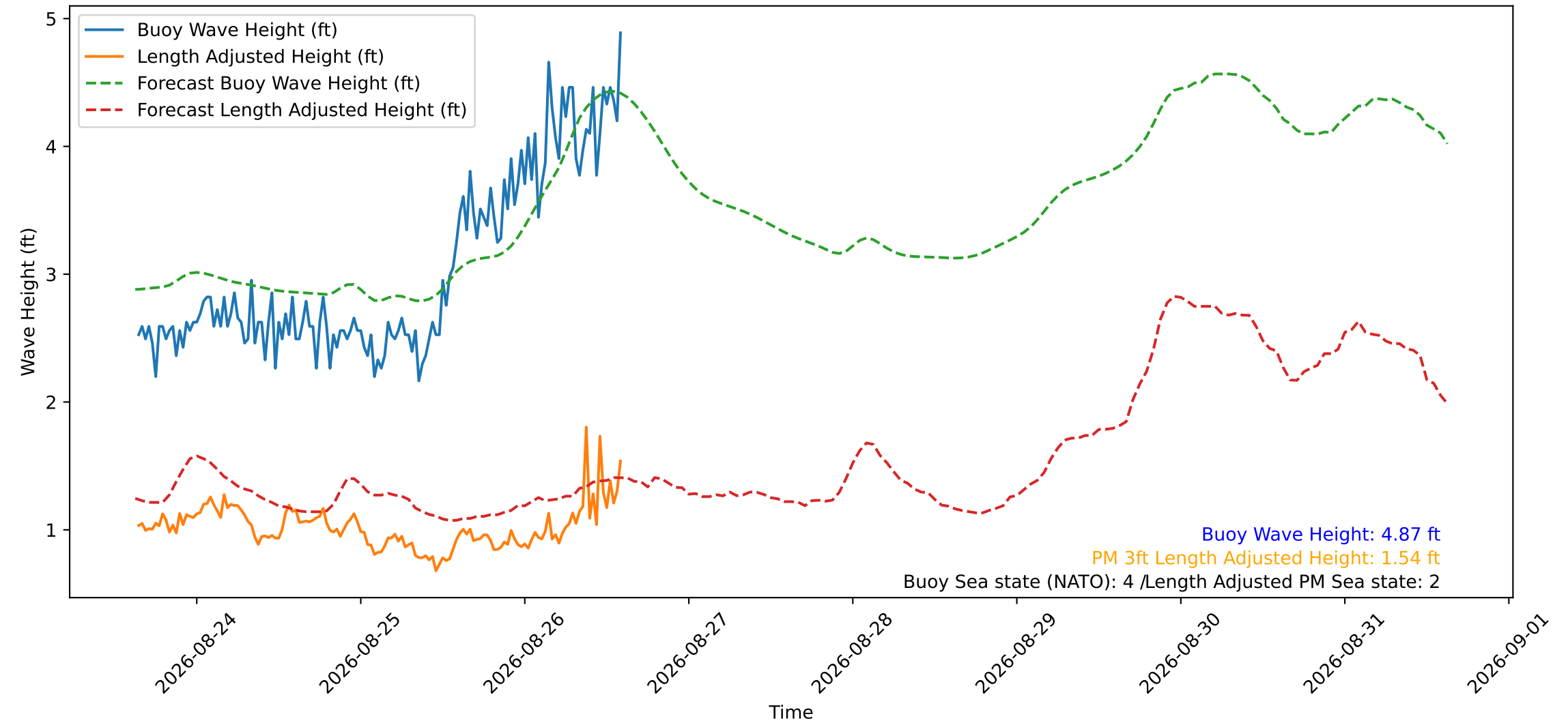
Wave Heights over Time for Red Beach at 2026-08-26 15:00:49
