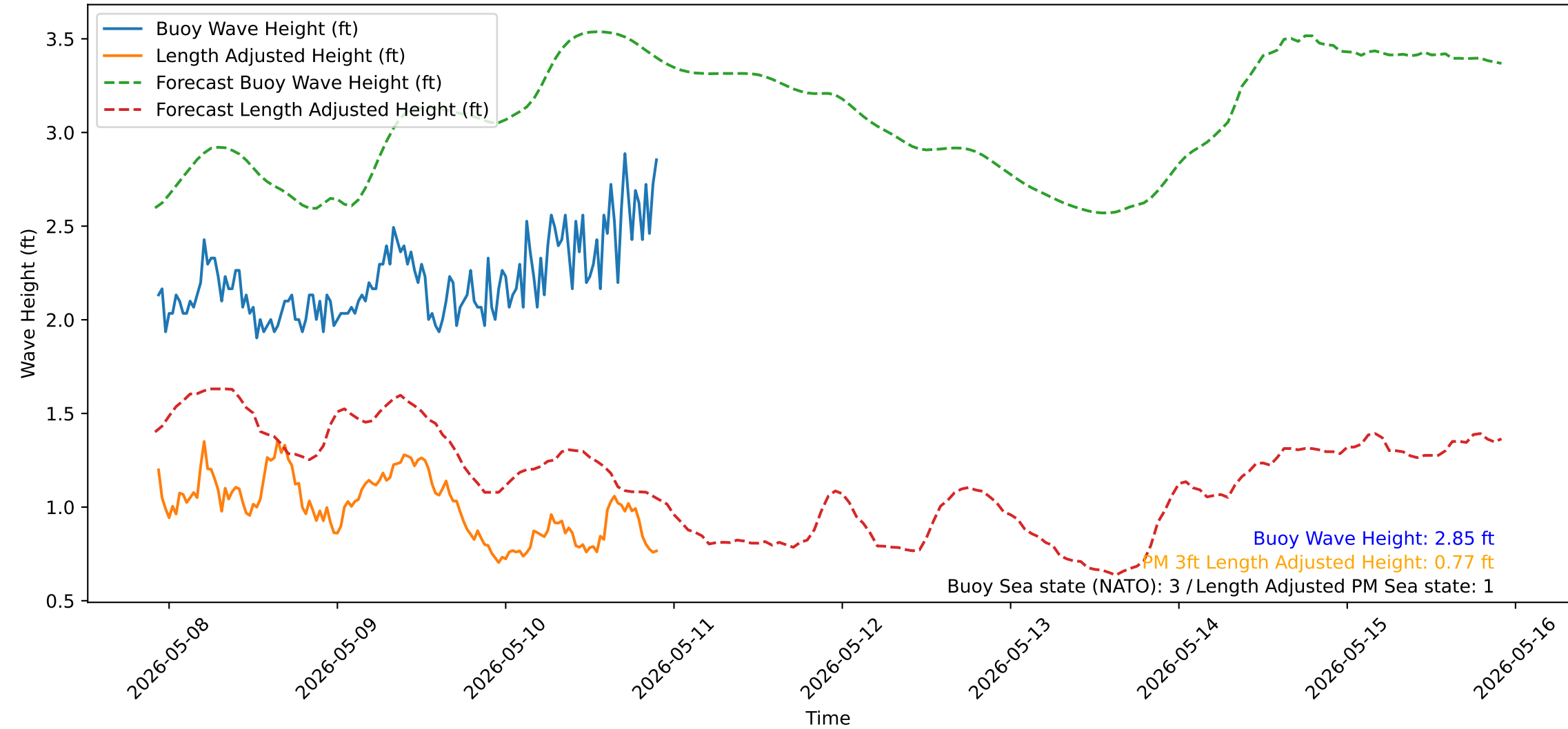
Wave Heights over Time for Red Beach at 2026-05-10 22:10:50
