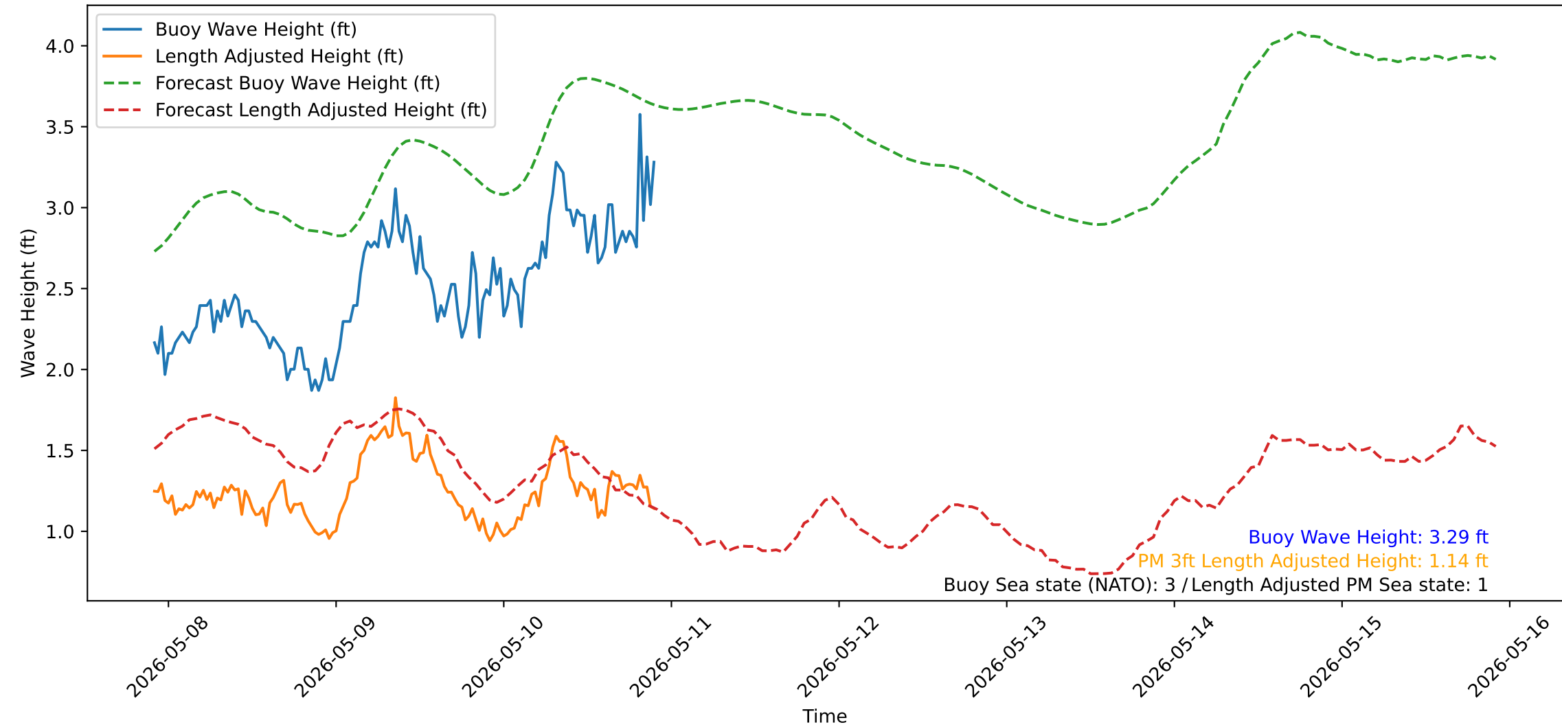
Wave Heights over Time for Oceanside Harbor at 2026-05-10 22:10:31
