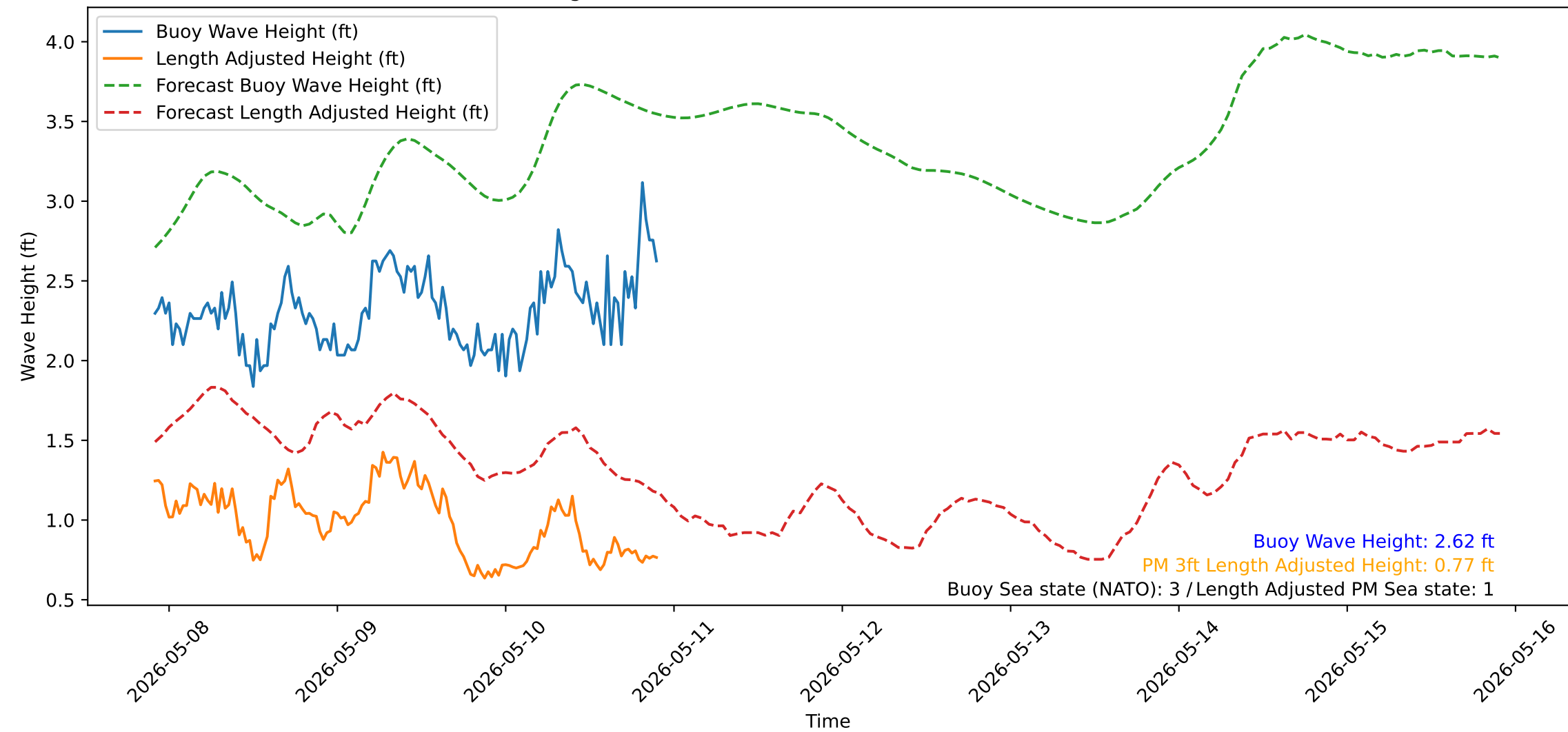
Wave Heights over Time for Green Beach at 2026-05-10 22:11:12
