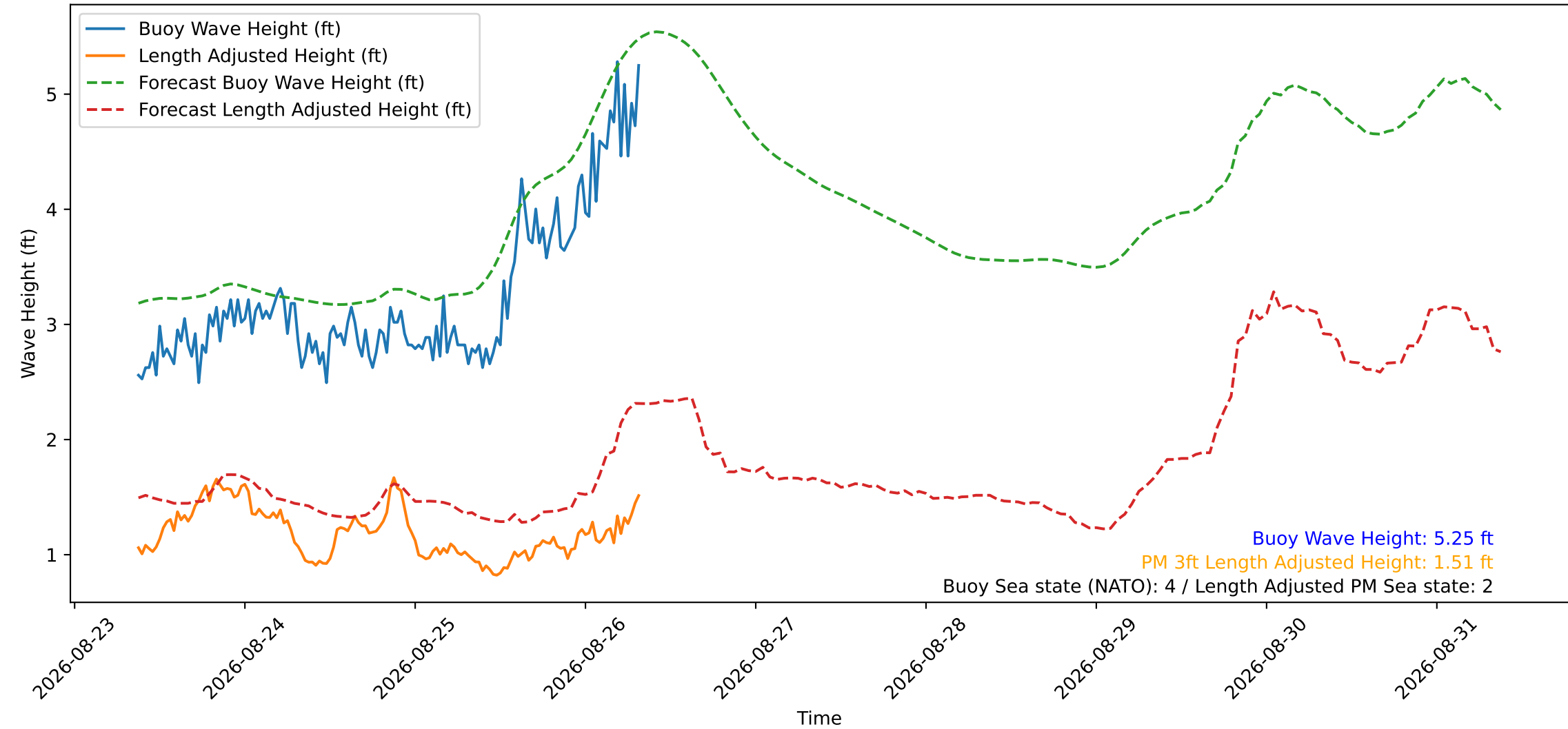
Wave Heights over Time for Green Beach at 2026-08-26 08:31:15
