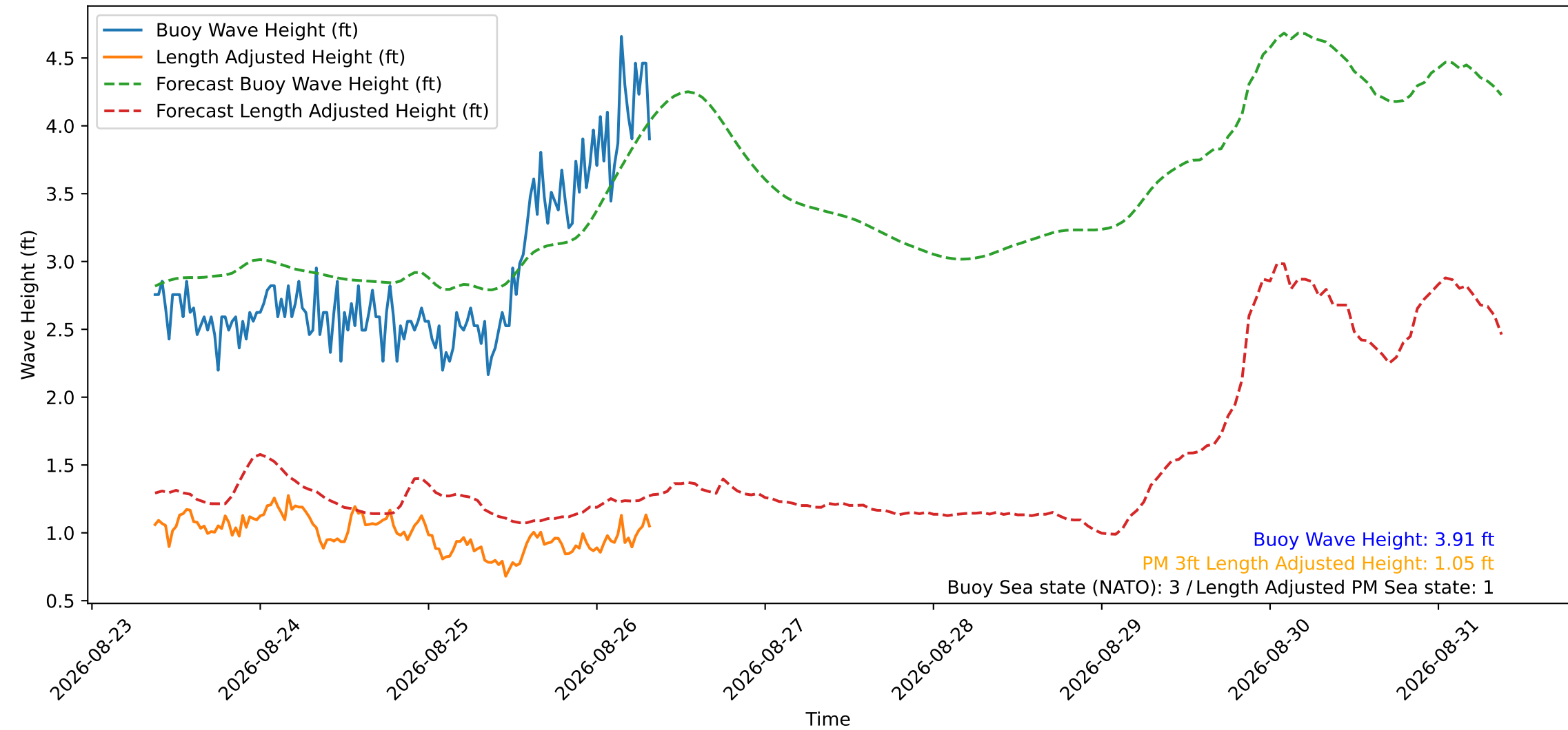
Wave Heights over Time for Red Beach at 2026-08-26 08:30:51
