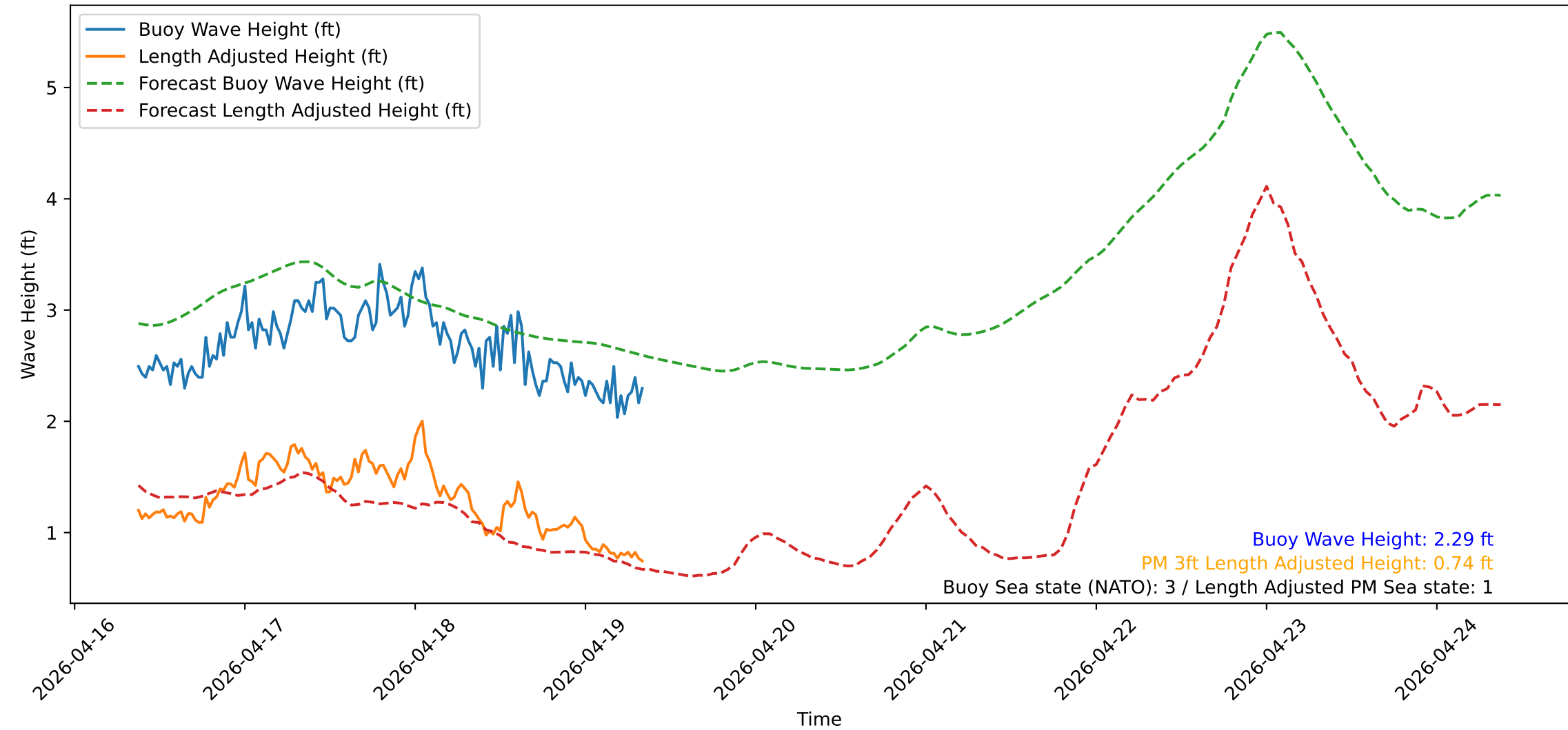
Wave Heights over Time for Oceanside Harbor at 2026-04-19 09:00:31
