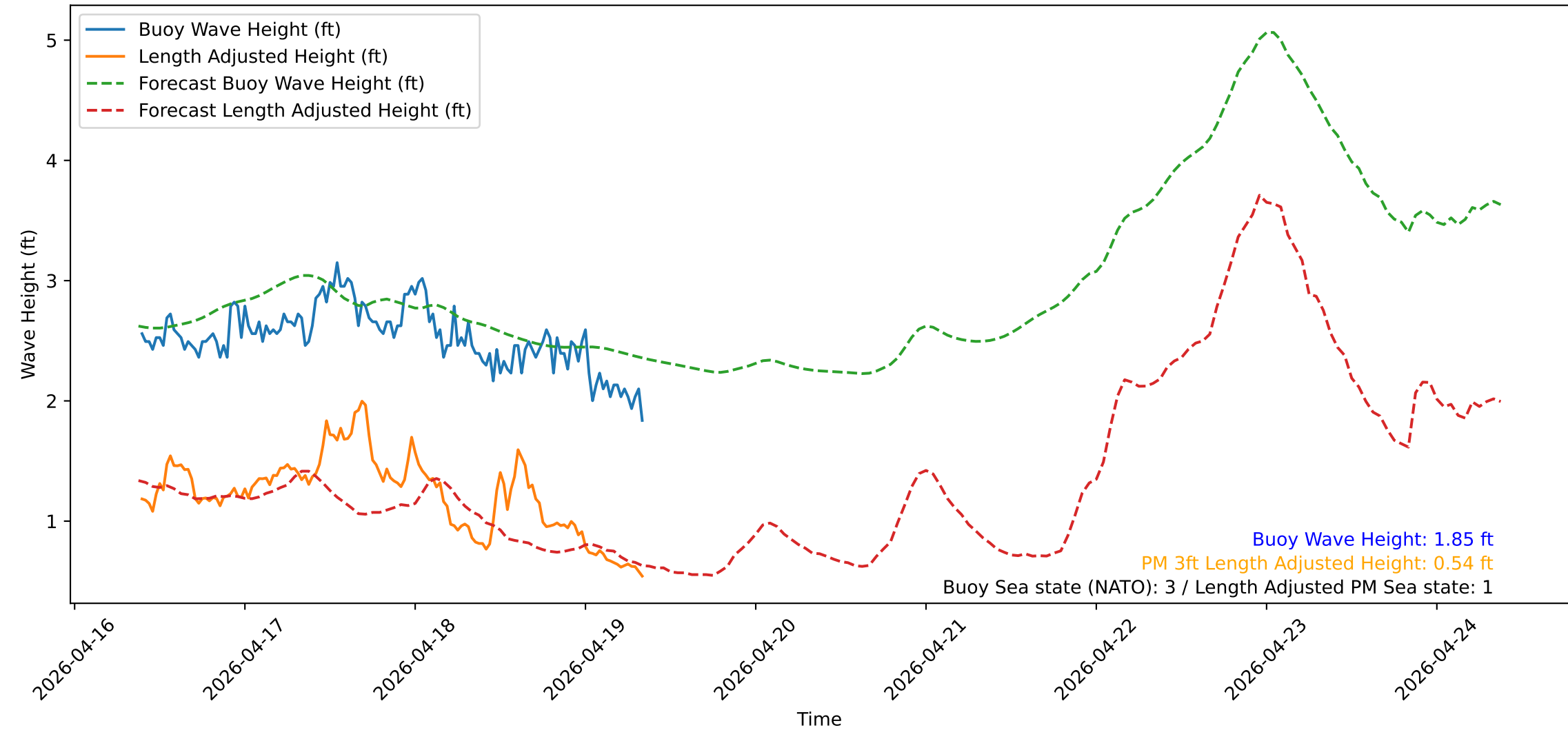
Wave Heights over Time for Red Beach at 2026-04-19 09:00:50
