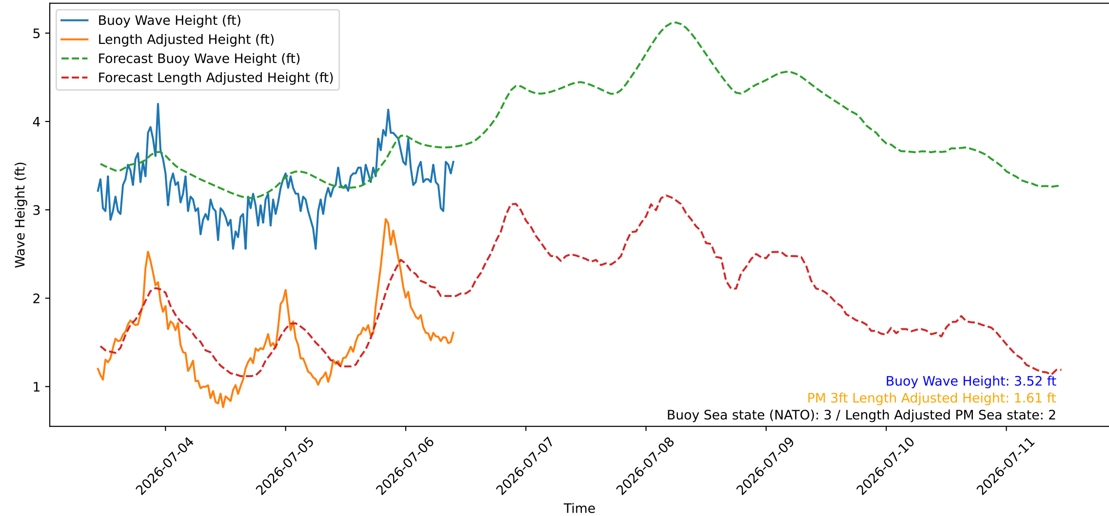
Wave Heights over Time for Green Beach at 2026-07-06 10:31:08
