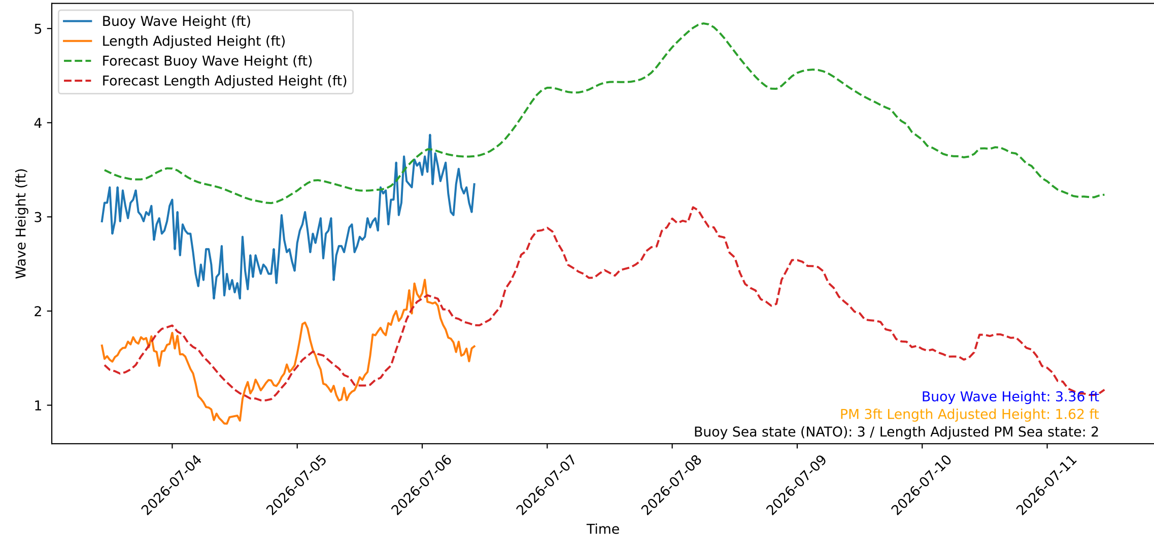
Wave Heights over Time for Oceanside Harbor at 2026-07-06 10:30:26
