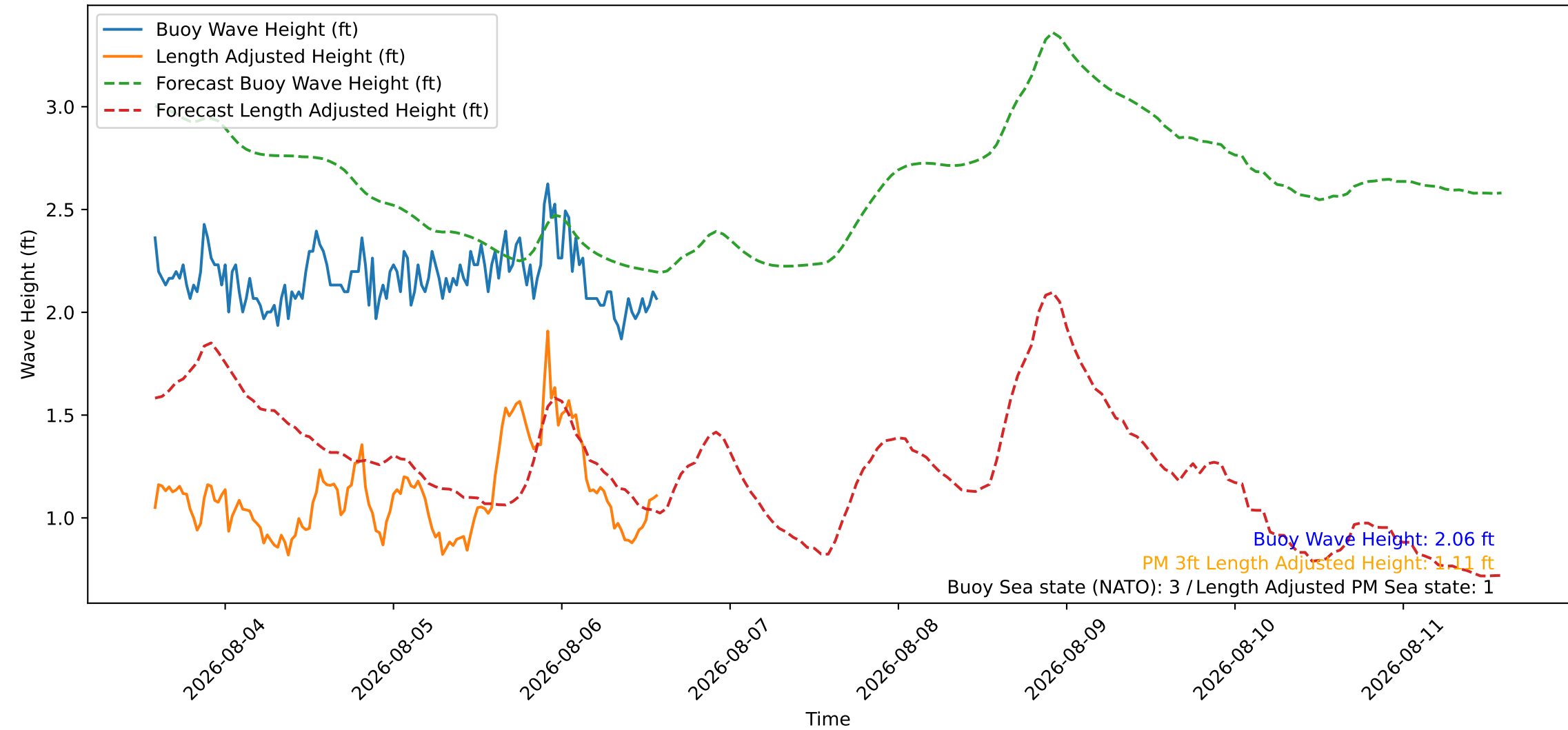
Wave Heights over Time for Green Beach at 2026-08-06 14:11:08
