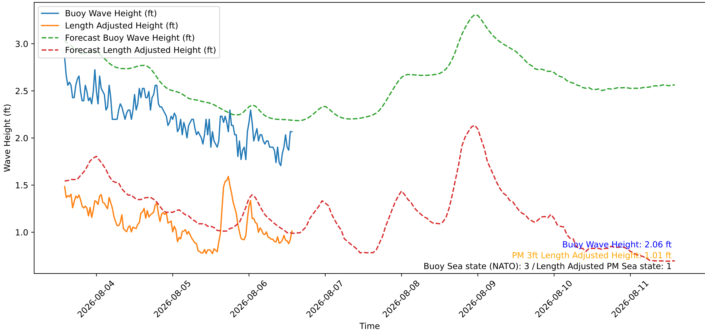
Wave Heights over Time for Oceanside Harbor at 2026-08-06 14:10:27
