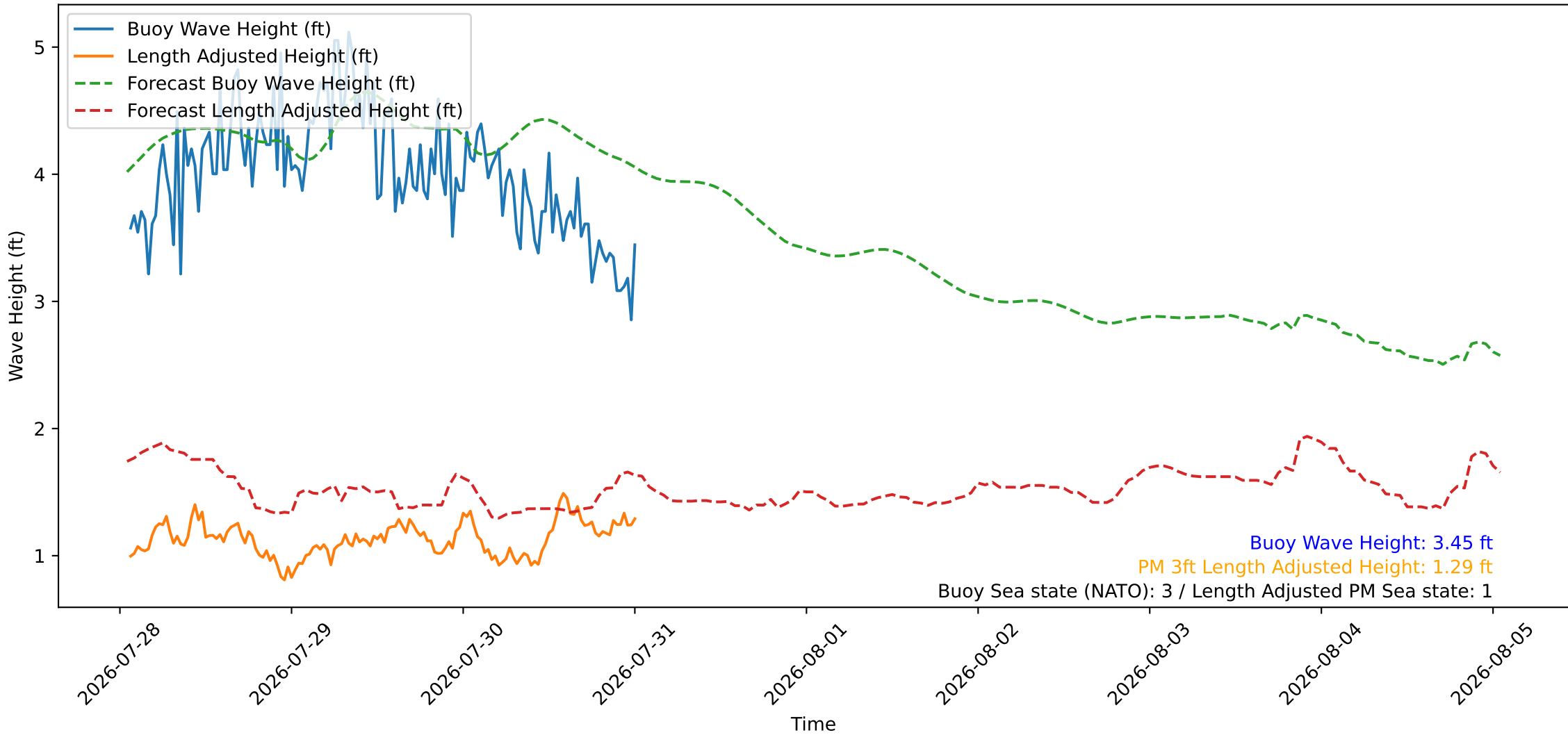
Wave Heights over Time for Red Beach at 2026-07-31 01:00:46
