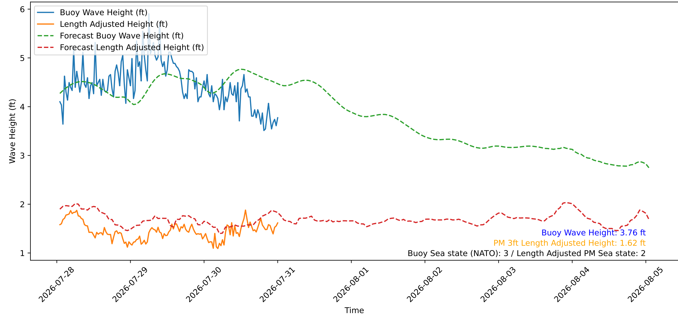
Wave Heights over Time for Oceanside Harbor at 2026-07-31 01:00:26
