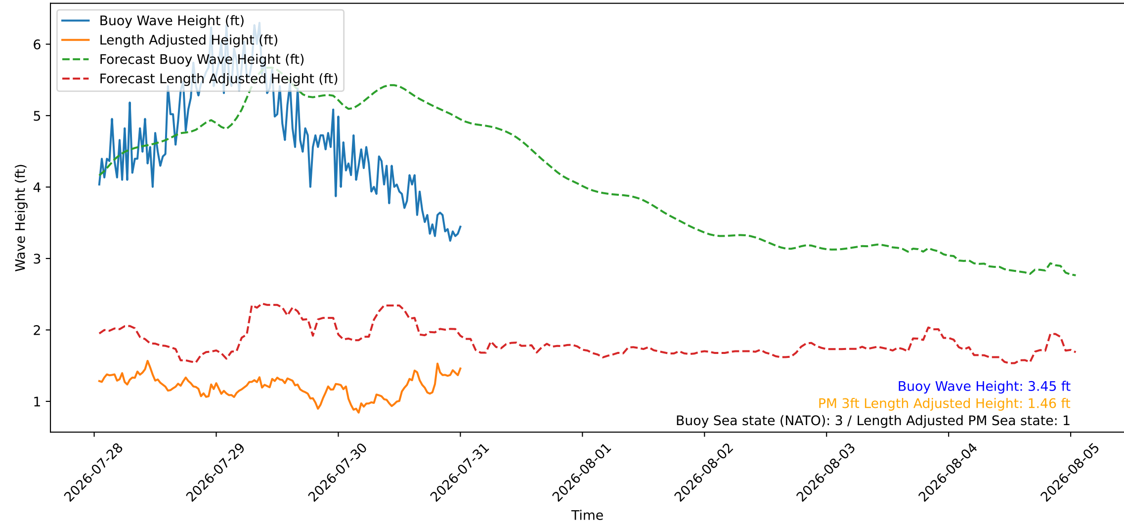
Wave Heights over Time for Green Beach at 2026-07-31 01:01:08
