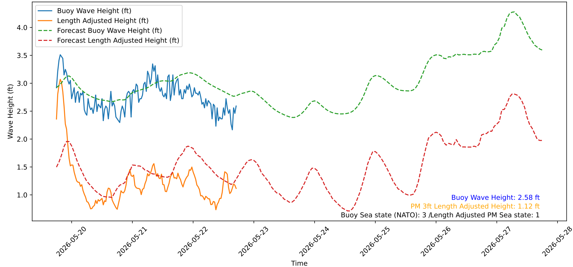
Wave Heights over Time for Red Beach at 2026-05-22 17:50:54
