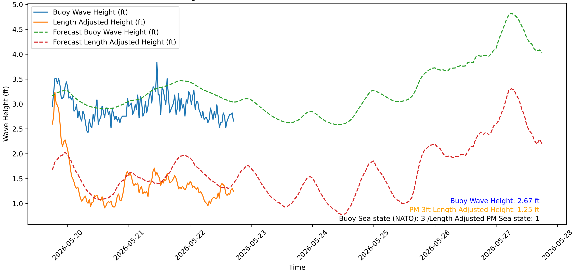
Wave Heights over Time for Oceanside Harbor at 2026-05-22 17:50:32
