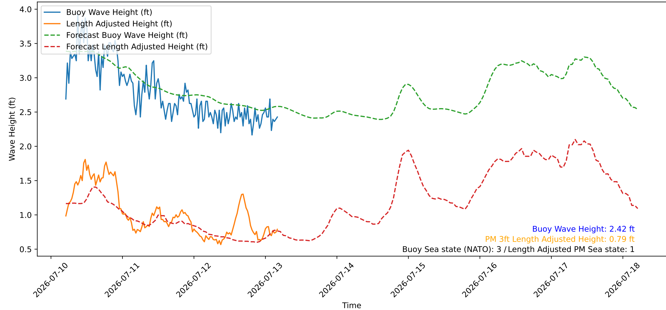
Wave Heights over Time for Red Beach at 2026-07-13 04:50:46
