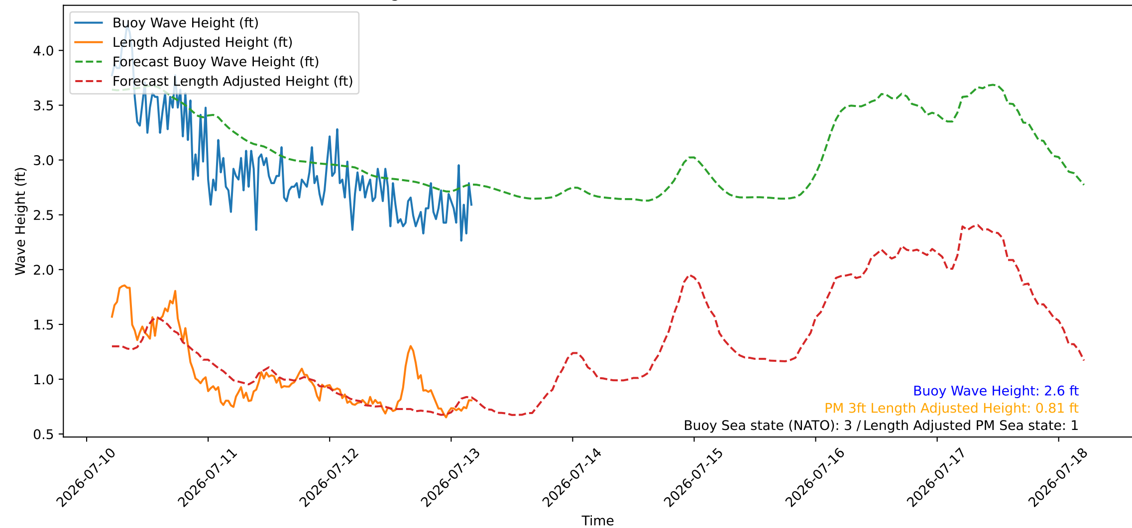
Wave Heights over Time for Oceanside Harbor at 2026-07-13 04:50:26
