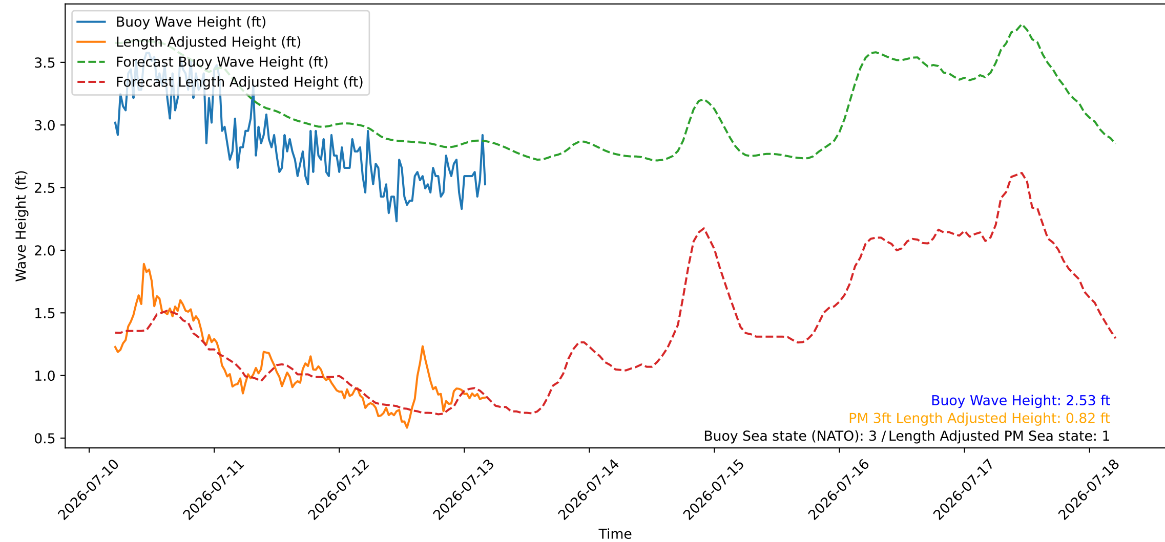
Wave Heights over Time for Green Beach at 2026-07-13 04:51:09
