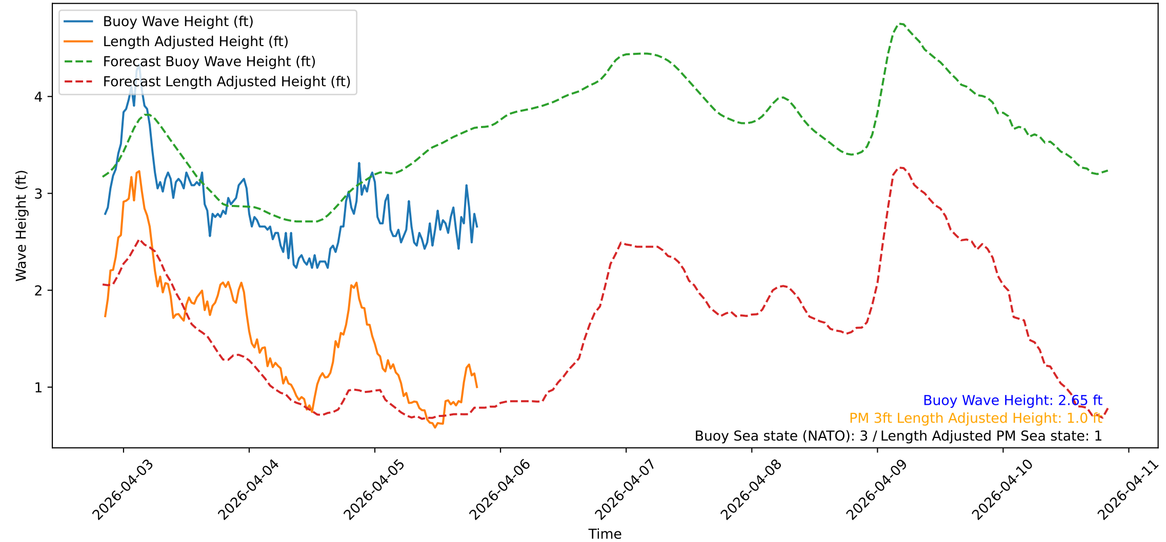
Wave Heights over Time for Green Beach at 2026-04-05 20:21:23
