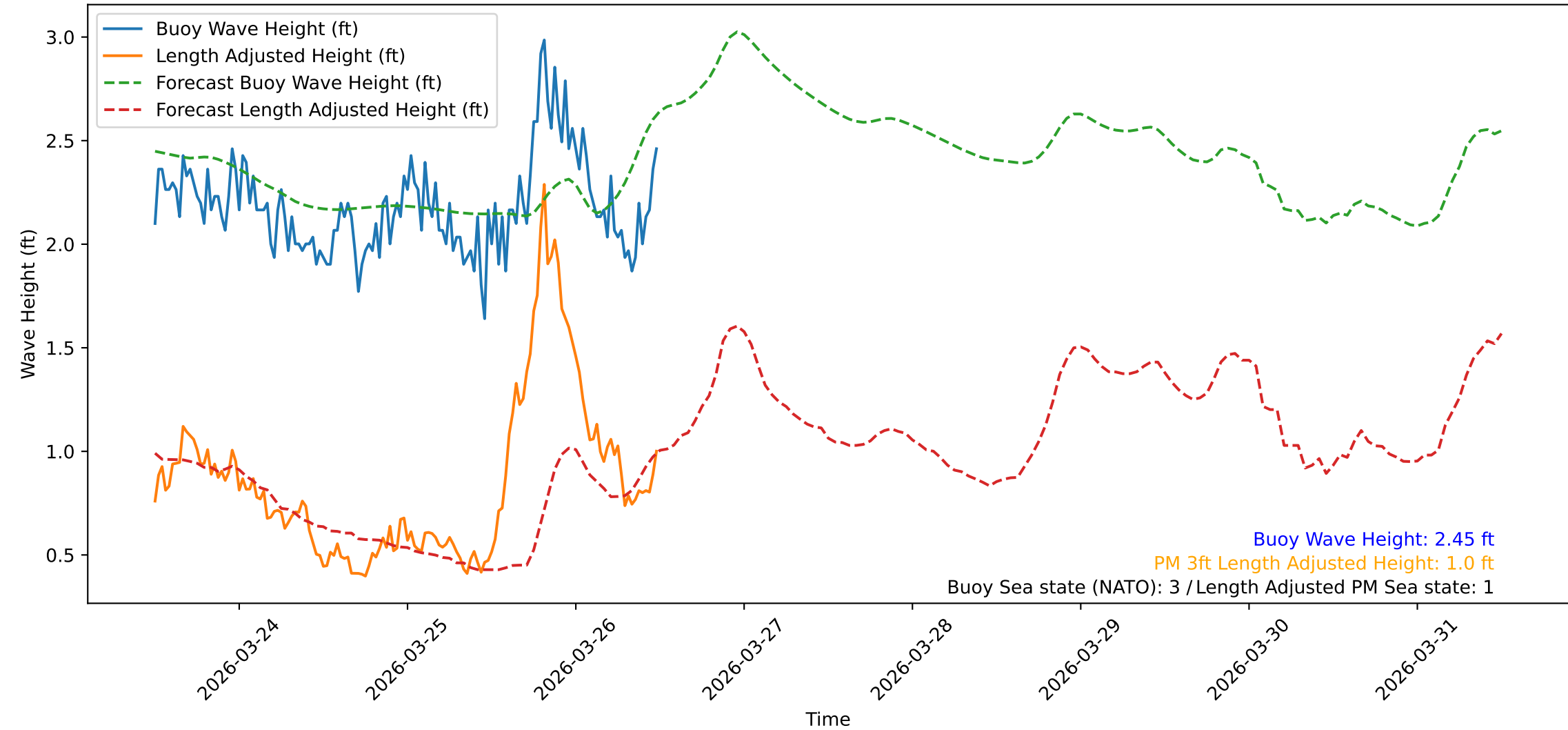
Wave Heights over Time for Green Beach at 2026-03-26 12:11:08
