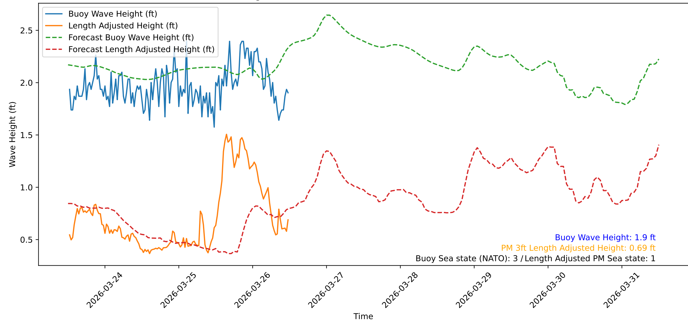
Wave Heights over Time for Red Beach at 2026-03-26 12:10:46
