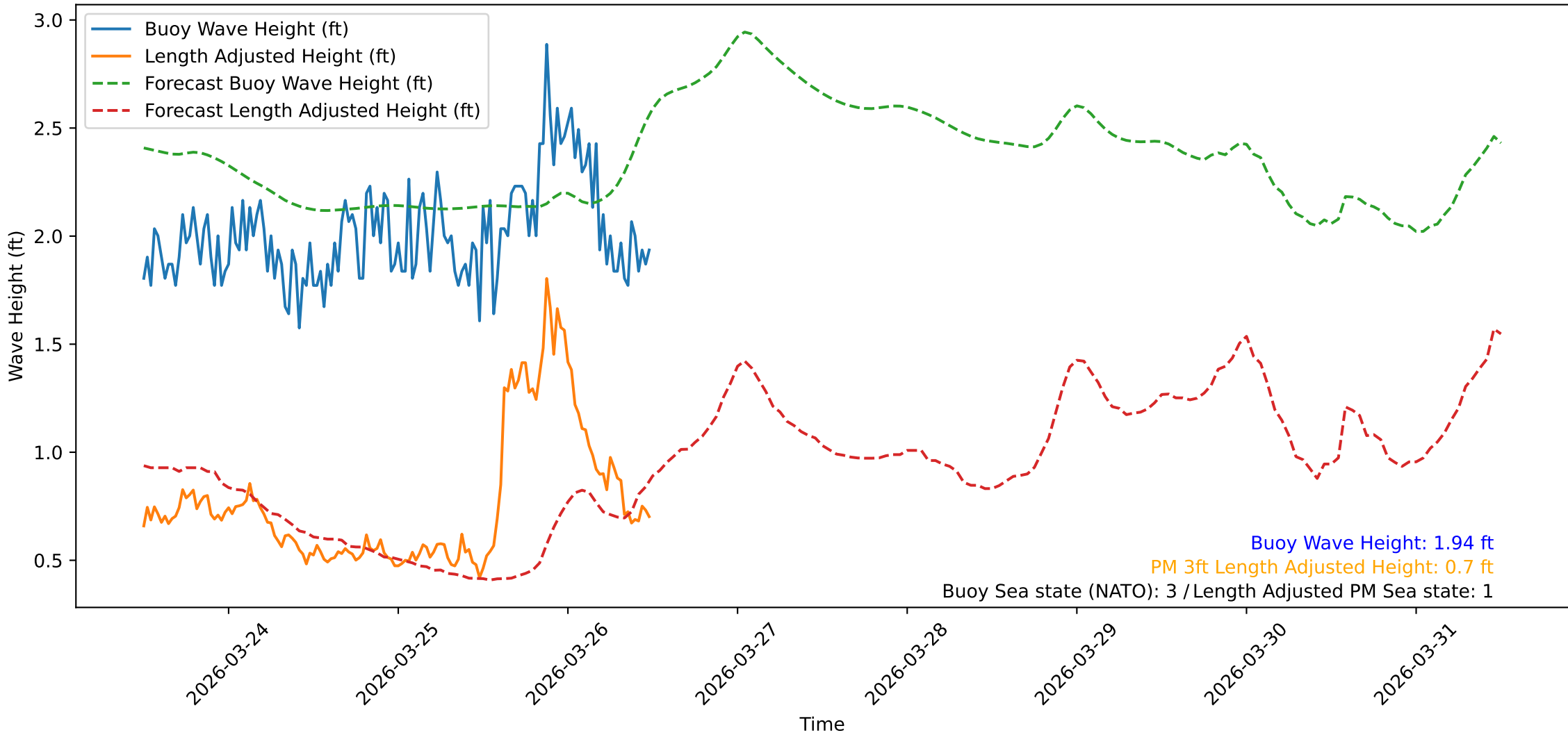
Wave Heights over Time for Oceanside Harbor at 2026-03-26 12:10:30
