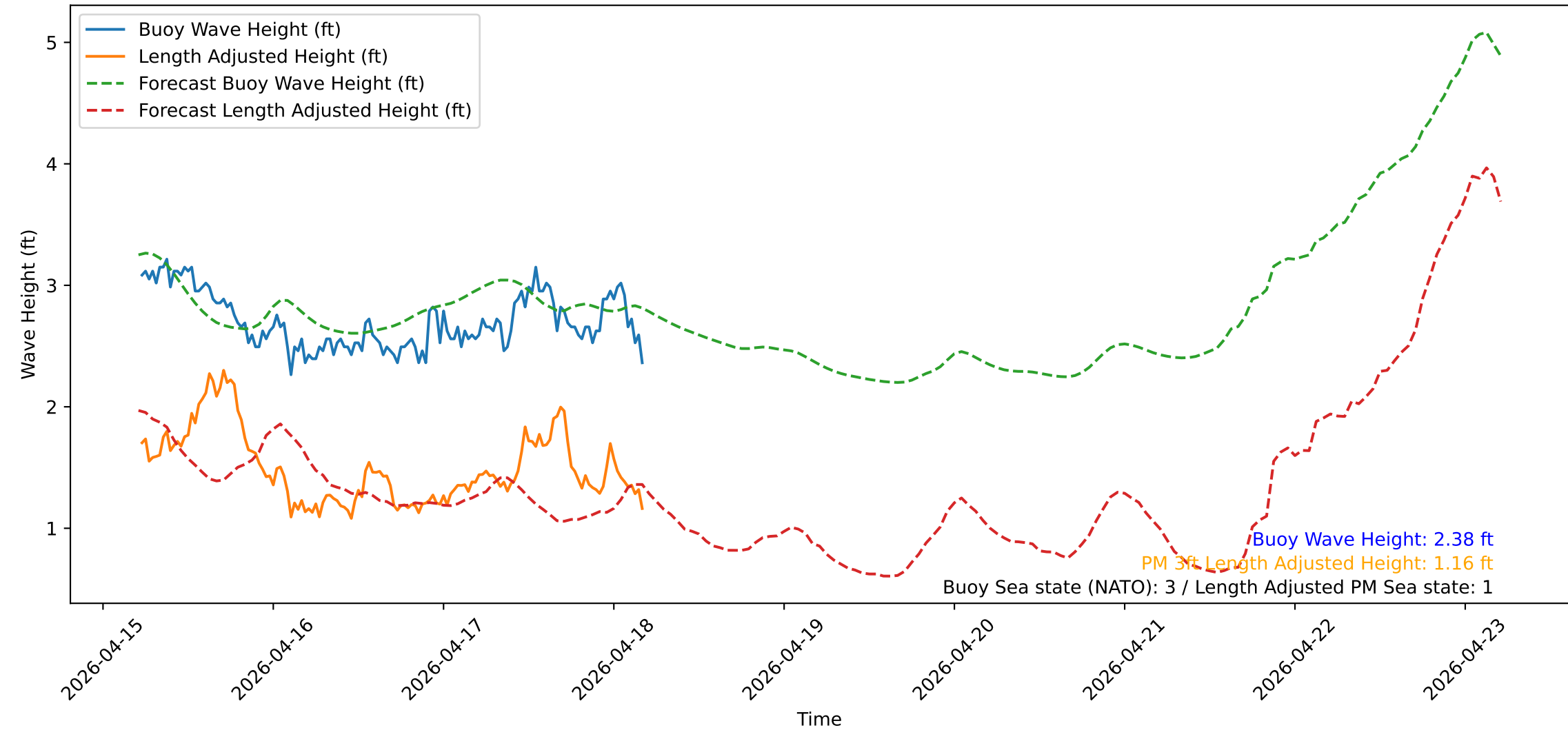
Wave Heights over Time for Red Beach at 2026-04-18 05:10:50
