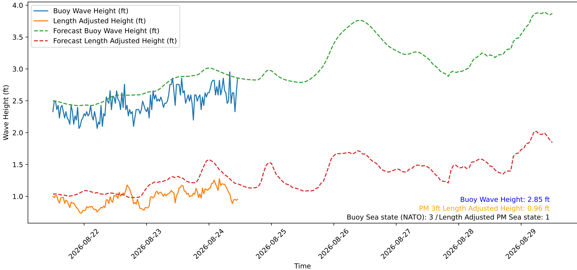
Wave Heights over Time for Red Beach at 2026-08-24 11:50:50
