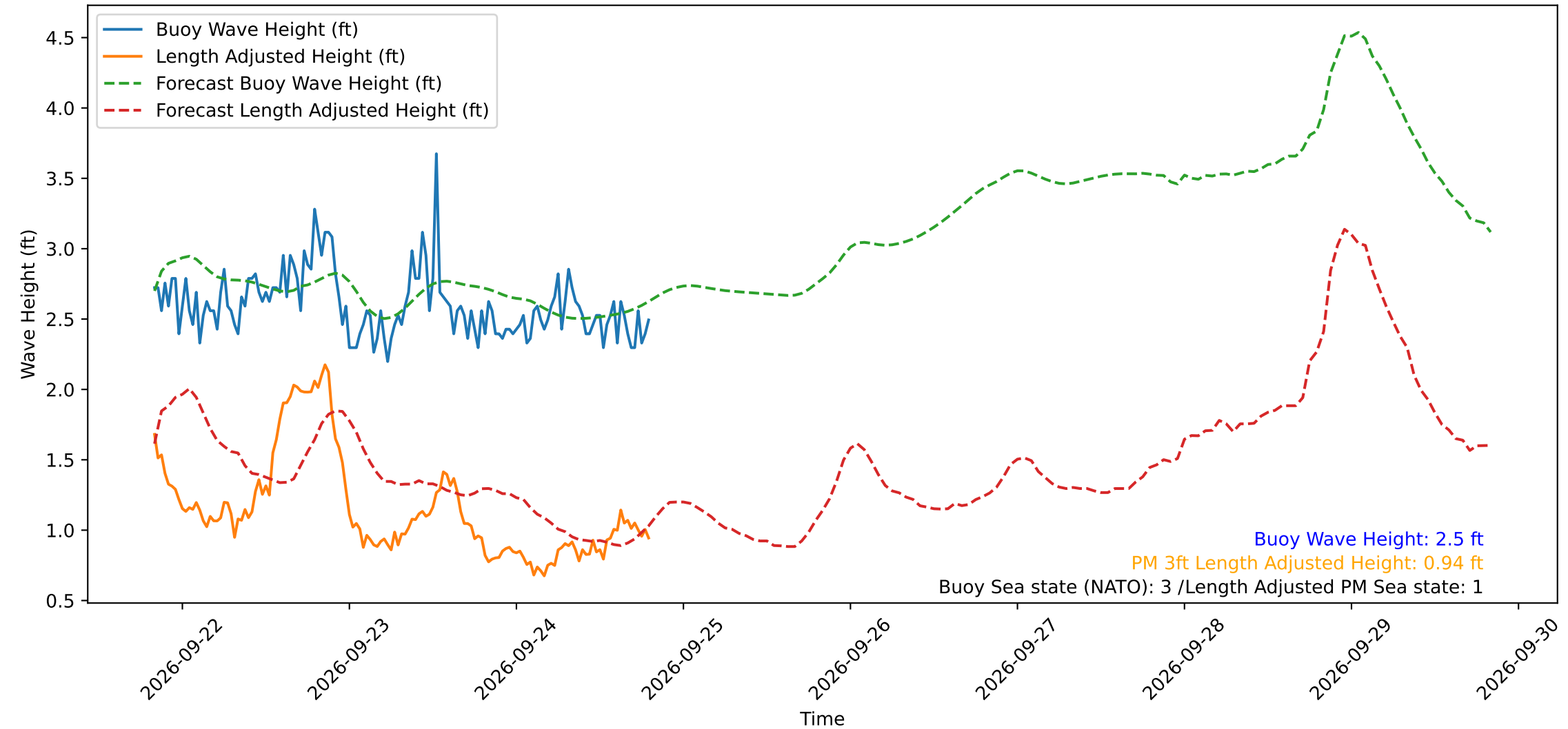
Wave Heights over Time for Red Beach at 2026-09-24 19:40:49
