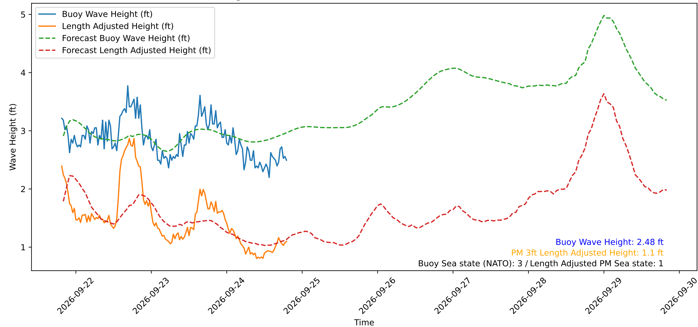
Wave Heights over Time for Oceanside Harbor at 2026-09-24 19:40:29
