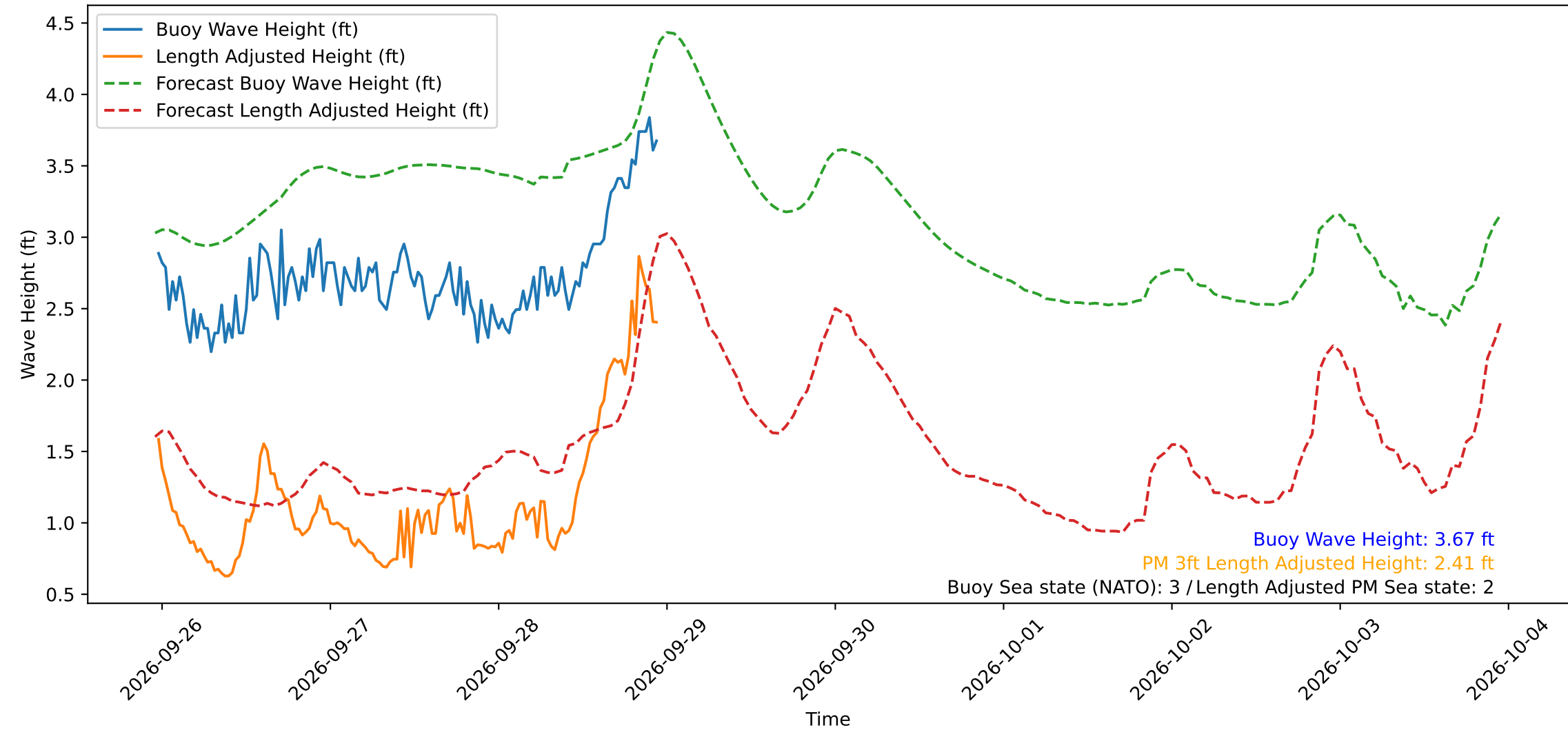
Wave Heights over Time for Red Beach at 2026-09-28 23:10:49
