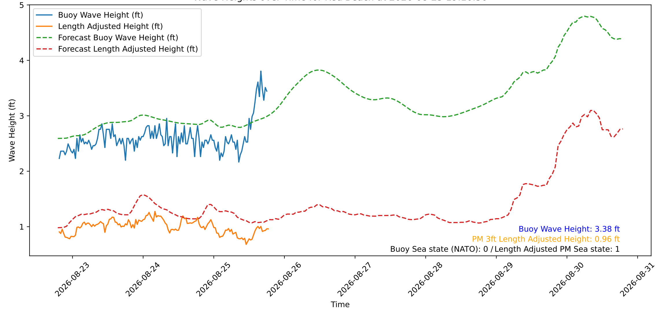
Wave Heights over Time for Red Beach at 2026-08-25 19:10:50
