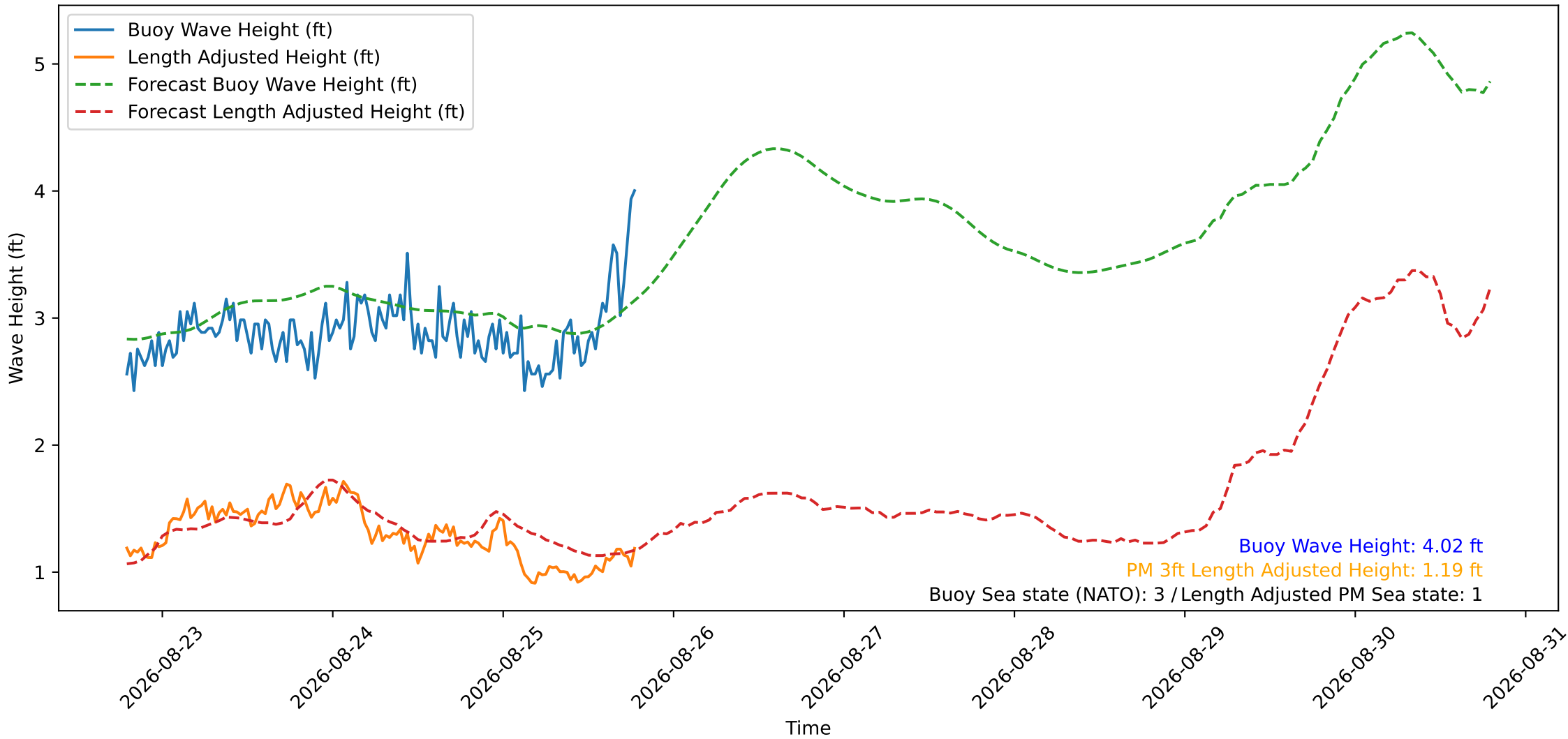
Wave Heights over Time for Oceanside Harbor at 2026-08-25 19:10:30
