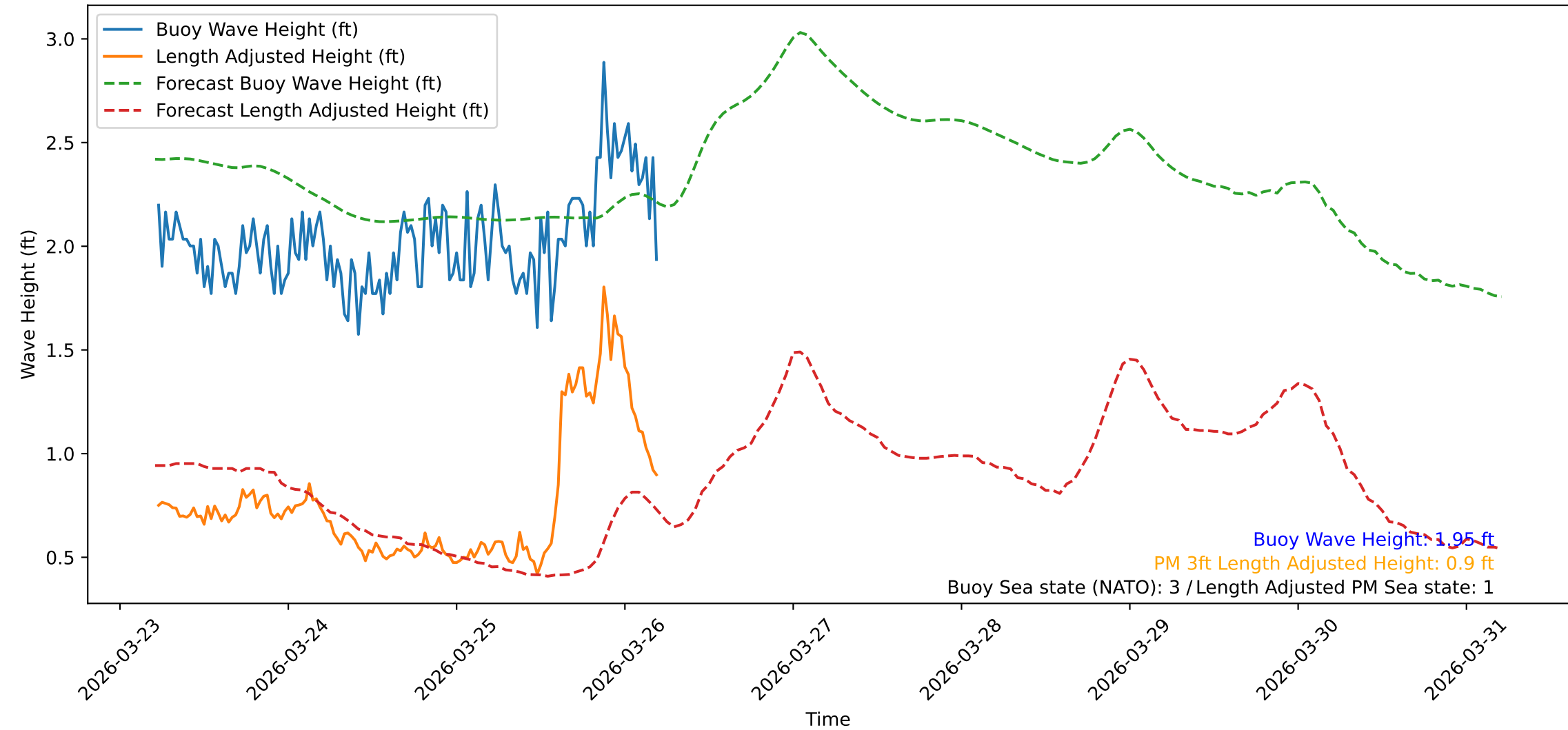
Wave Heights over Time for Oceanside Harbor at 2026-03-26 05:20:31
