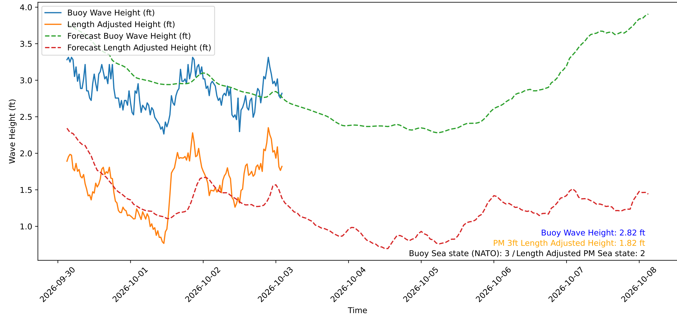
Wave Heights over Time for Oceanside Harbor at 2026-10-03 03:00:29
