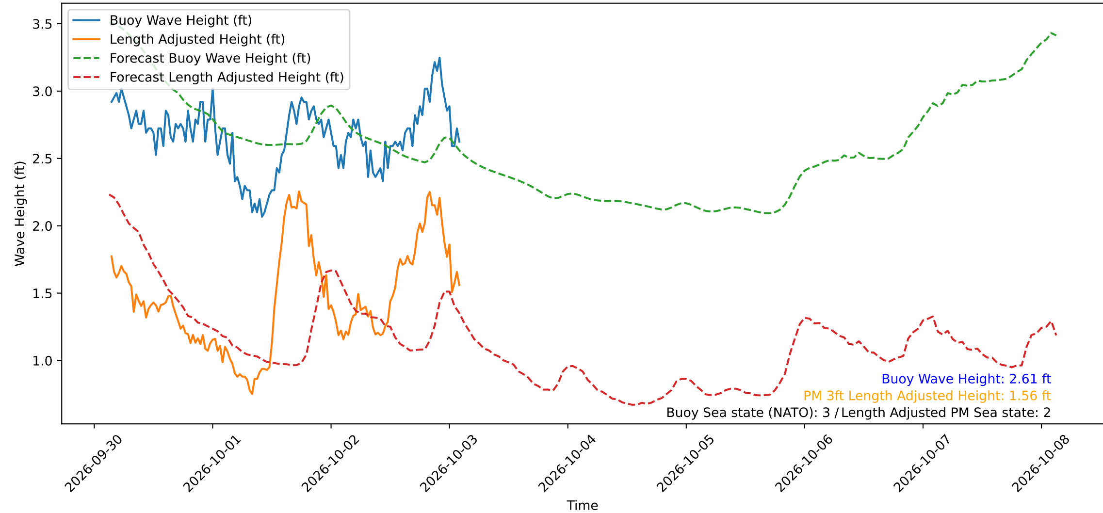
Wave Heights over Time for Red Beach at 2026-10-03 03:00:48
