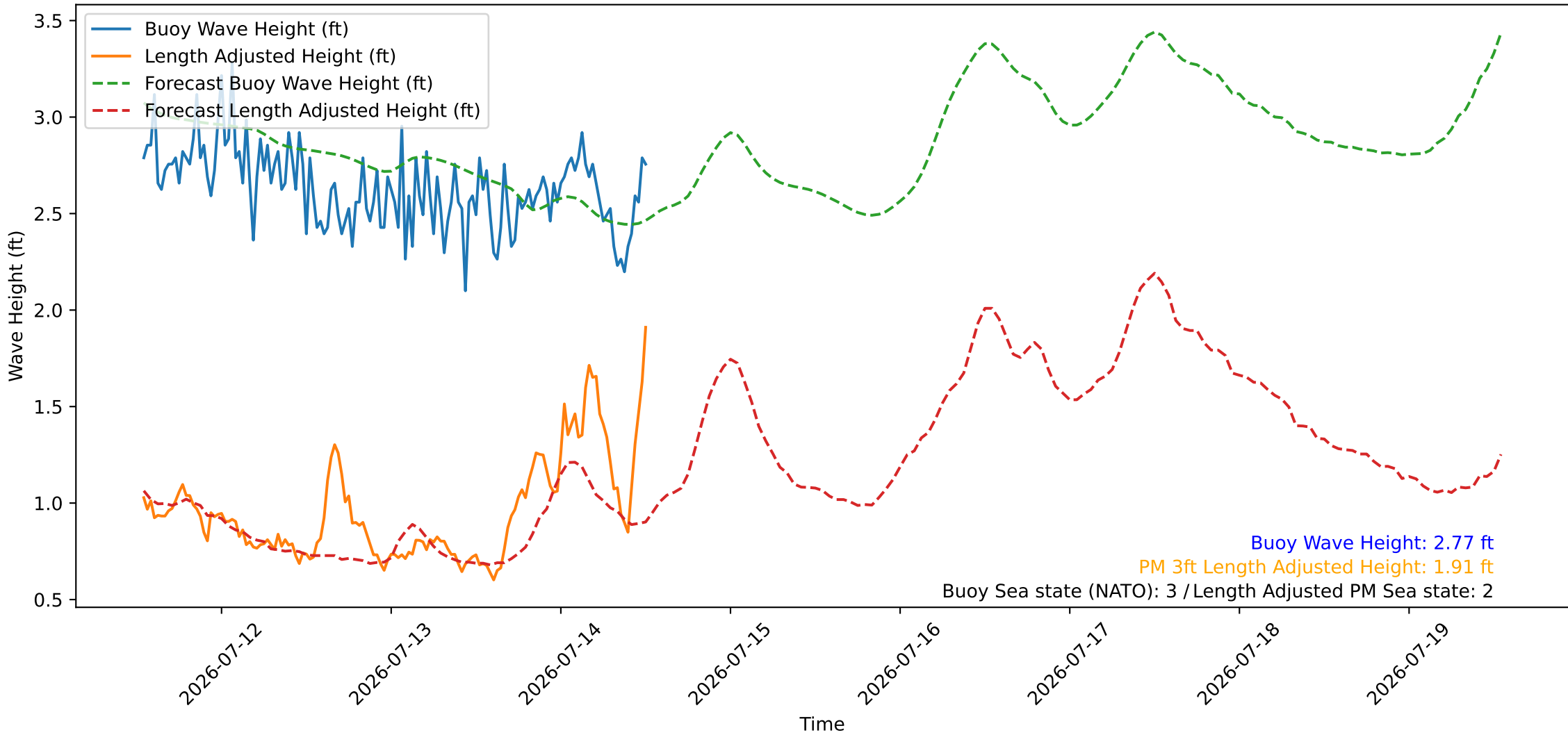
Wave Heights over Time for Oceanside Harbor at 2026-07-14 12:50:26
