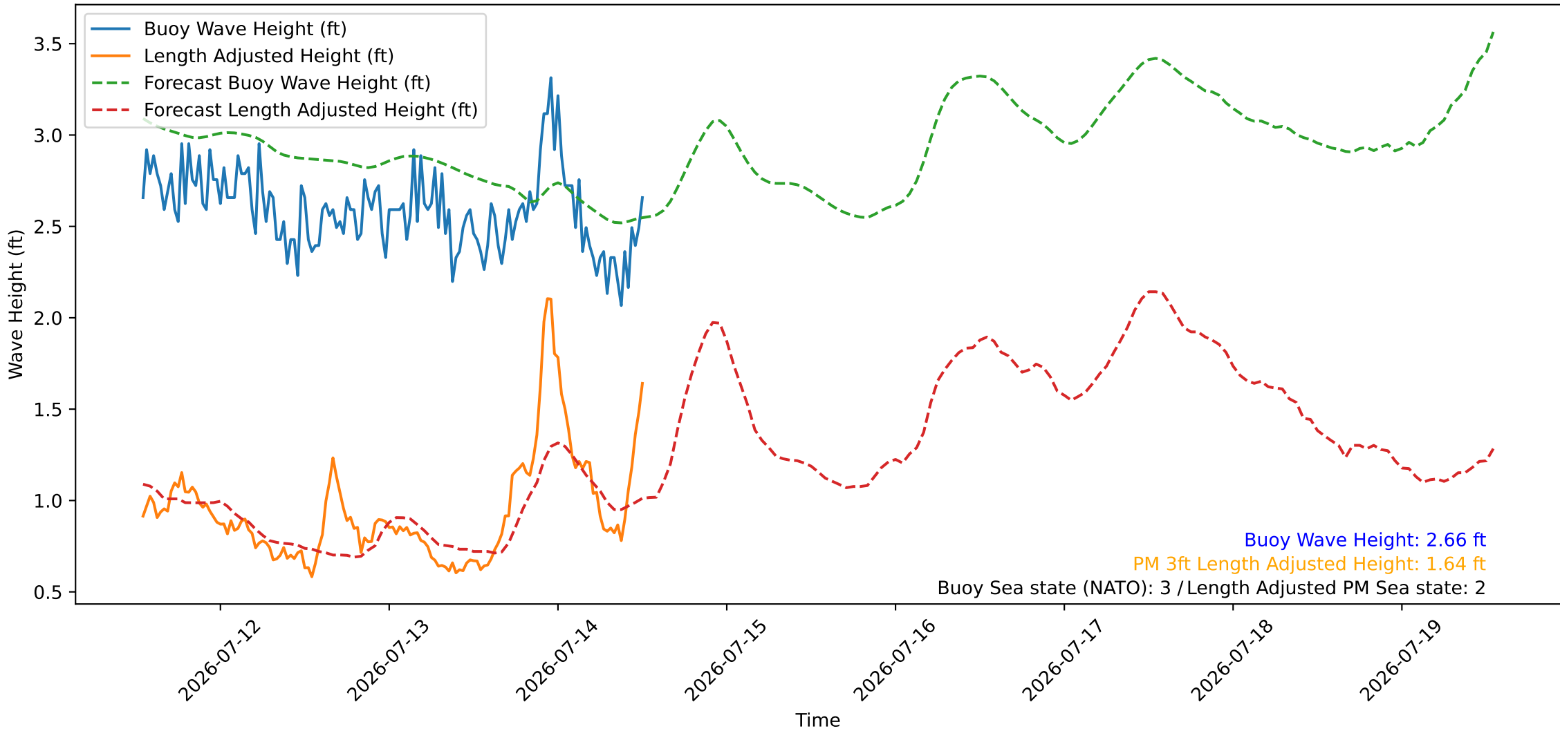
Wave Heights over Time for Green Beach at 2026-07-14 12:51:10
