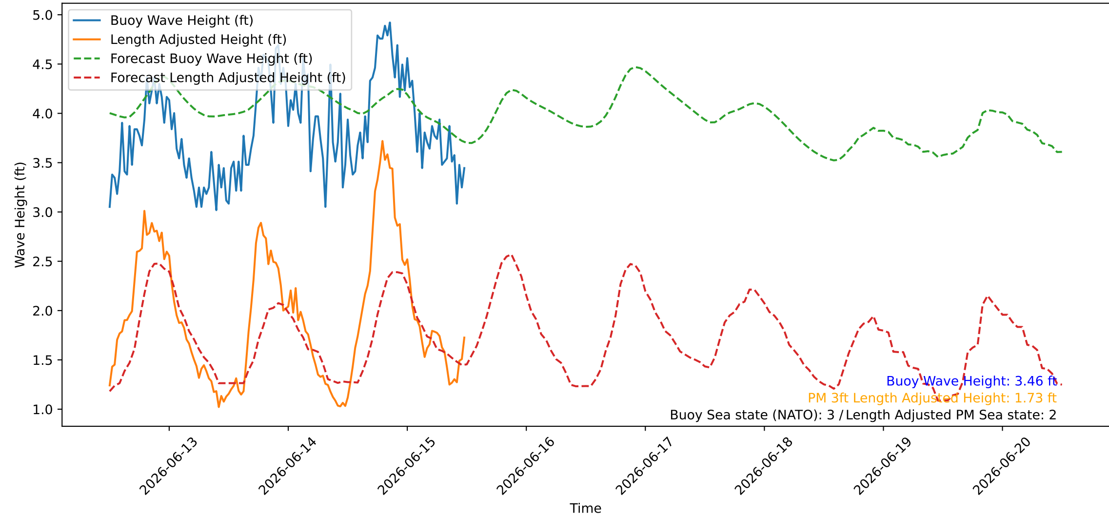
Wave Heights over Time for Green Beach at 2026-06-15 12:11:08
