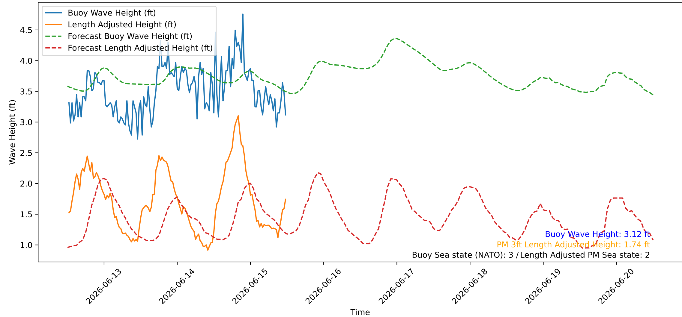
Wave Heights over Time for Red Beach at 2026-06-15 12:10:45
