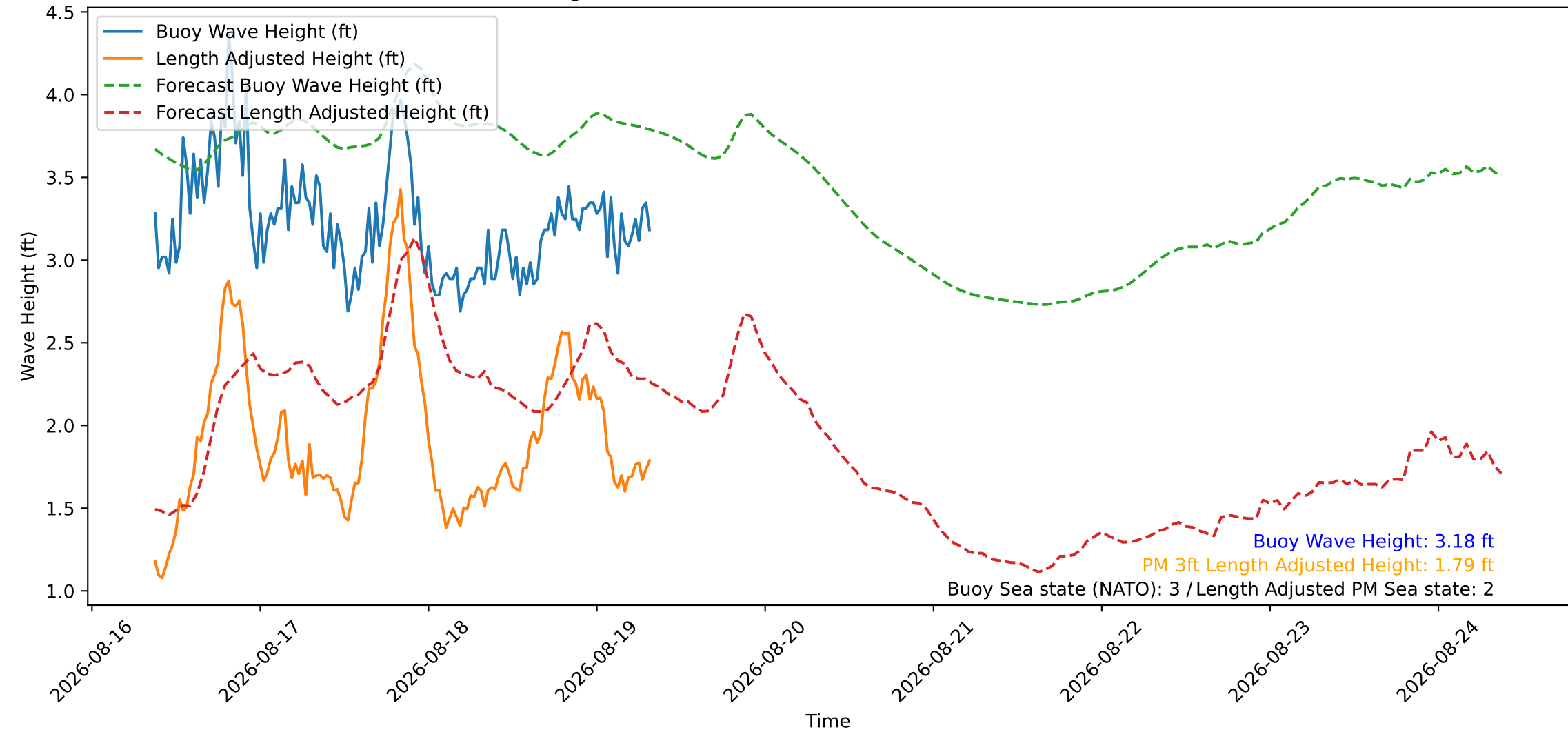
Wave Heights over Time for Green Beach at 2026-08-19 08:31:09
