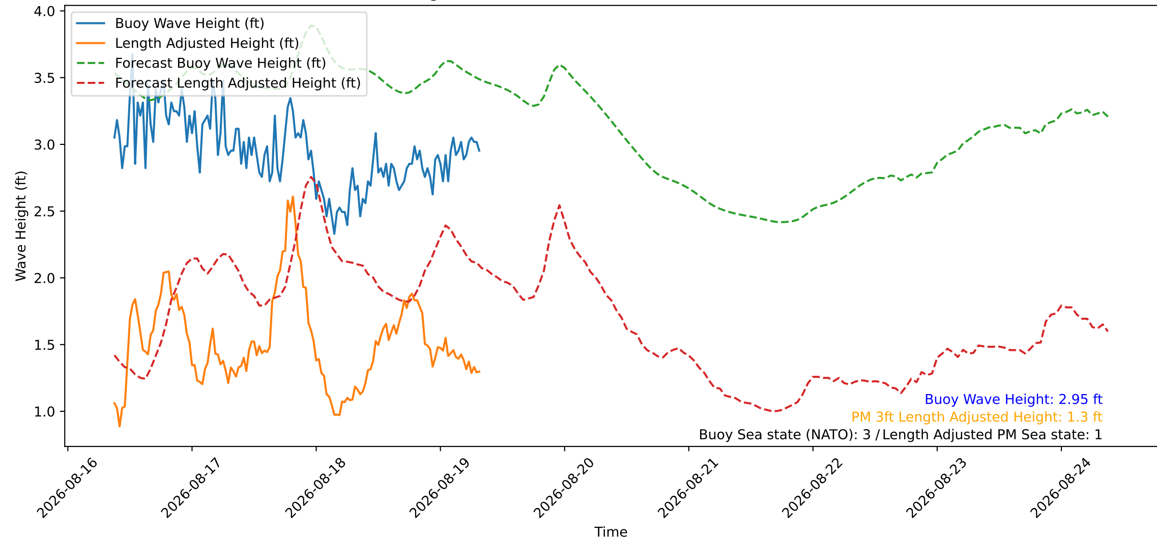
Wave Heights over Time for Red Beach at 2026-08-19 08:30:47
