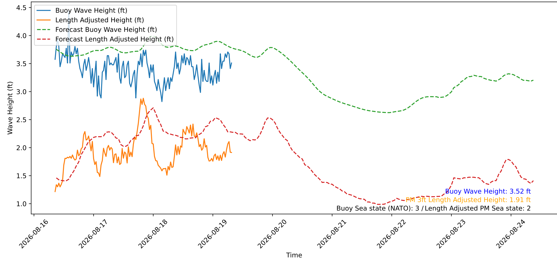
Wave Heights over Time for Oceanside Harbor at 2026-08-19 08:30:27
