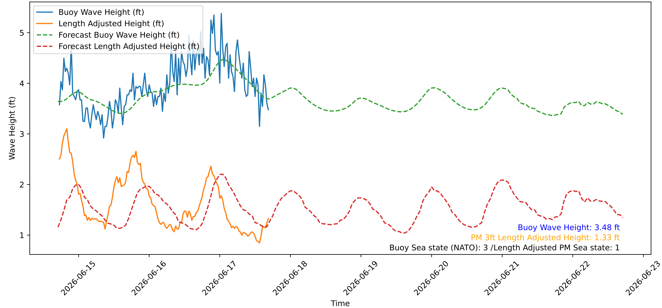
Wave Heights over Time for Red Beach at 2026-06-17 17:20:48
