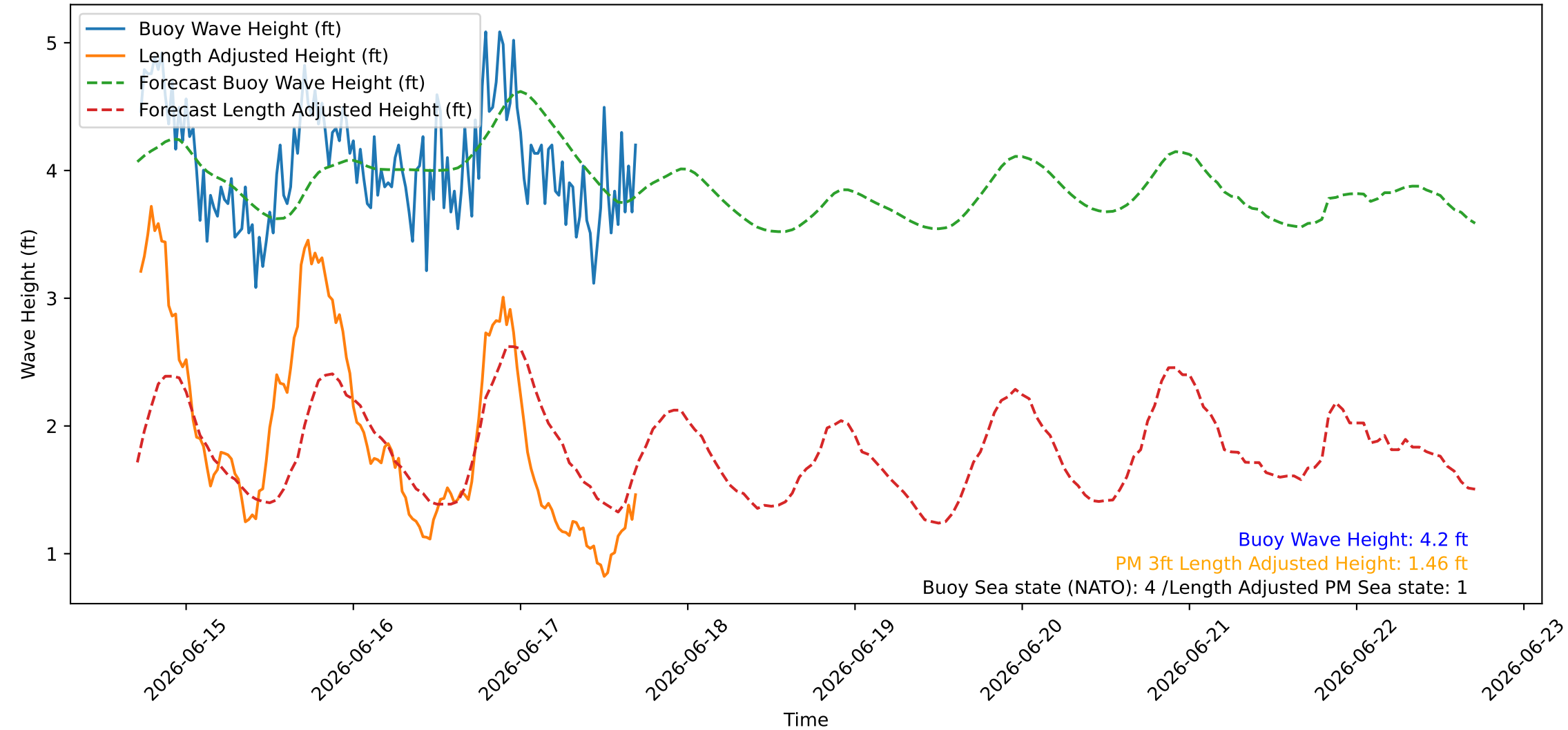
Wave Heights over Time for Green Beach at 2026-06-17 17:21:10
