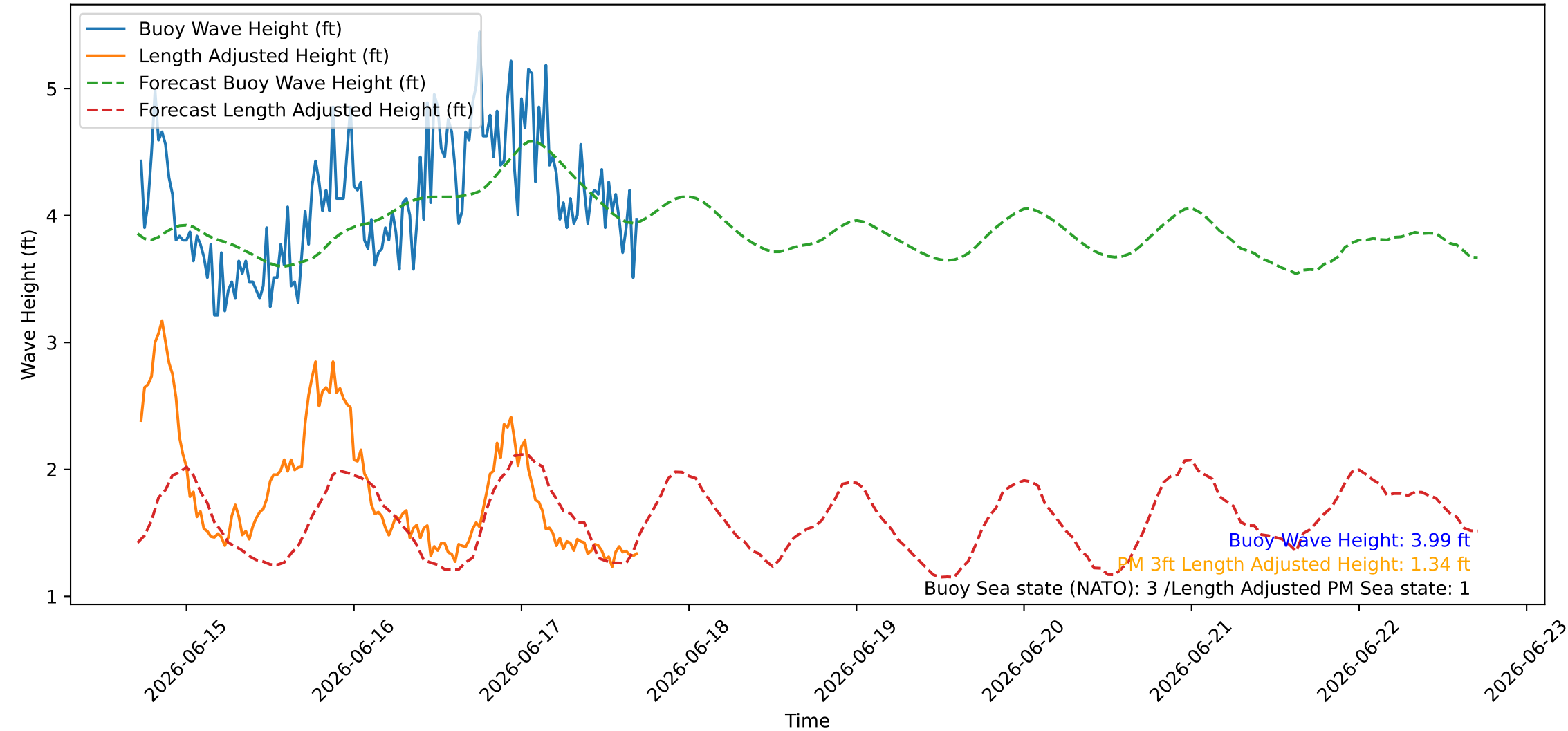
Wave Heights over Time for Oceanside Harbor at 2026-06-17 17:20:27
