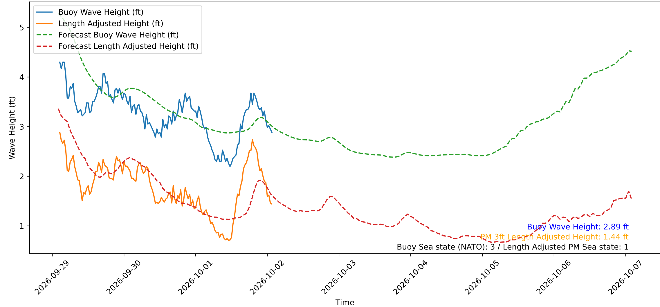
Wave Heights over Time for Green Beach at 2026-10-02 02:21:14
