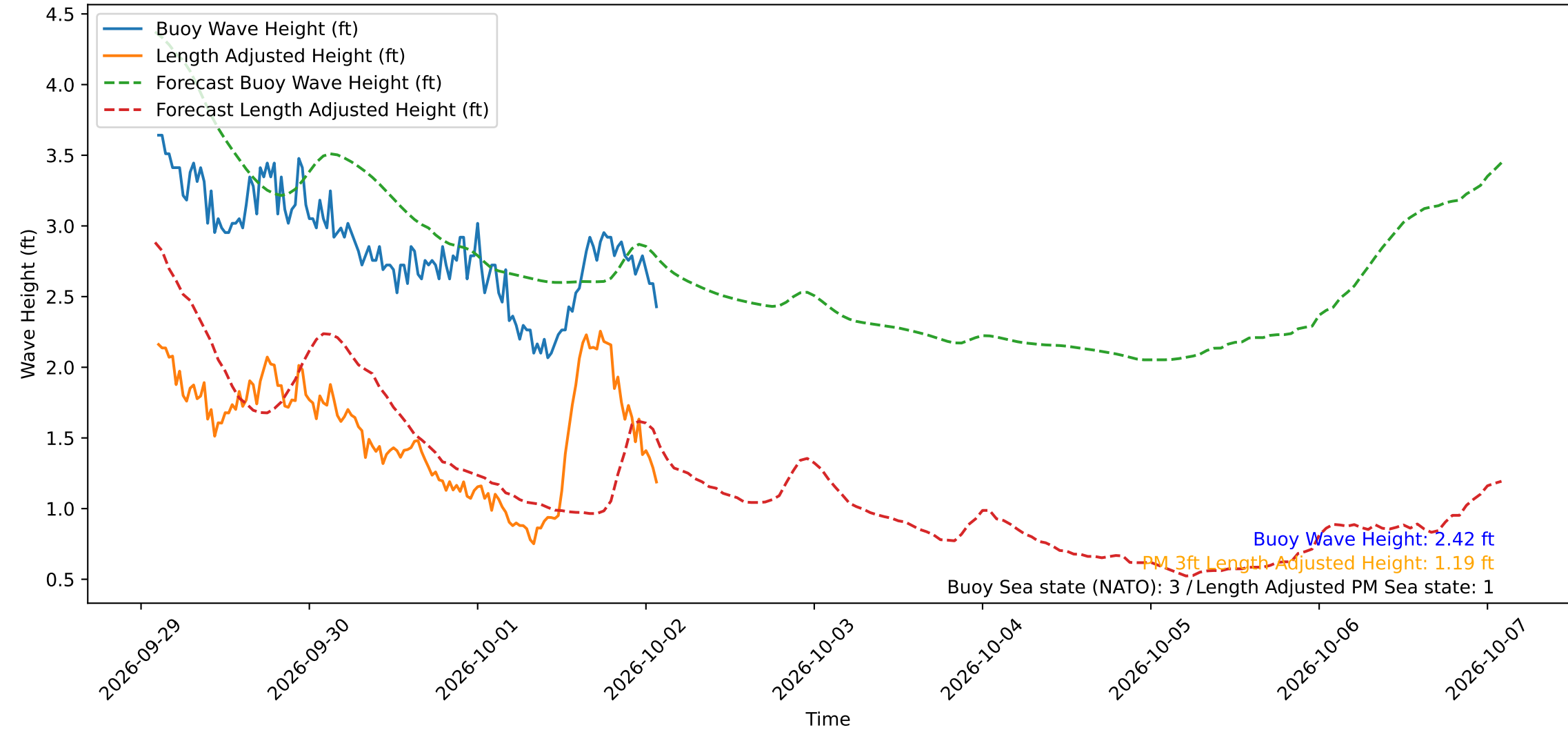
Wave Heights over Time for Red Beach at 2026-10-02 02:20:50
