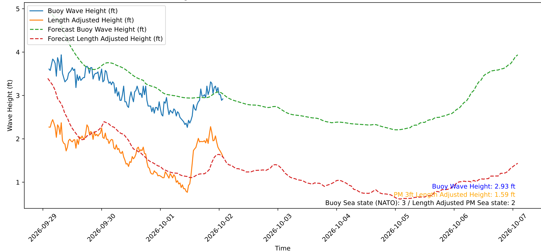
Wave Heights over Time for Oceanside Harbor at 2026-10-02 02:20:29
