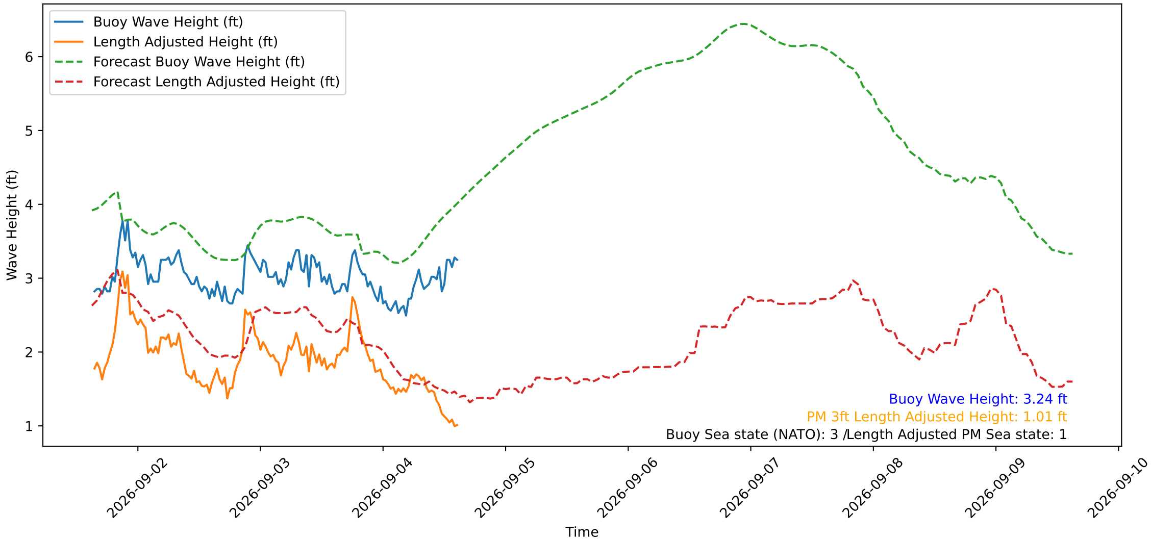
Wave Heights over Time for Green Beach at 2026-09-04 15:11:12
