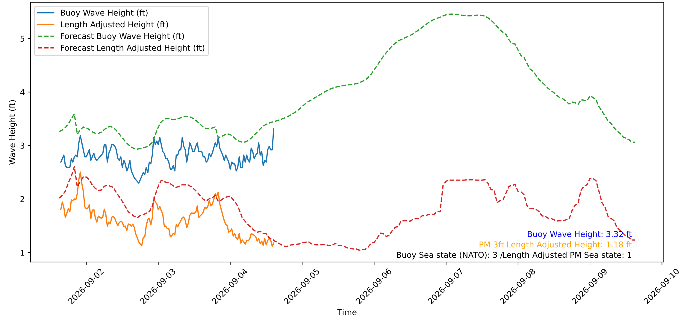
Wave Heights over Time for Red Beach at 2026-09-04 15:10:50
